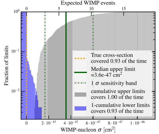
FIG. 9. Distribution of the lower (blue) and upper (gray) toy-MC limits on a 50 GeV/c 2 WIMP cross section. The upper (lower) limits are drawn as a cumulative (complementary cumulative) distribution, to show the fraction of limits that include a certain cross section. The corresponding signal expectation value is shown on the upper horizontal axis. The toy-MC did not include a true signal, indicated with a dashed orange line at 0. All upper limits are above 0, and 0.93 of lower limits are equal to 0, giving a total estimated coverage of 0.93 for the 500 toy-MCs used in this example, part of the dataset used for Fig. 11. As the cross section is constrained to be non-negative, the survival fraction below 0 is 1. Green solid and dot-dashed lines show the median upper limit and 1\sigma sensitivity band.
