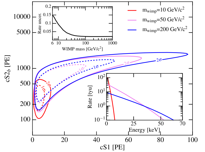
FIG. 8. The main panel shows the 1\sigma (dashed line) and 2\sigma contours of the WIMP signal model in (cS1, cS2_b) space, for WIMP mass of 10 GeV/ c^2 (red), 50 GeV/ c^2 (violet), and 200 GeV/ c^2 (blue), respectively. The lower right inset shows the differential energy rate, which is in unit of tyu, for these three WIMP masses, with an assumed WIMP-nucleon cross section of 10^{-45} \text{ cm}^2 . The upper left inset shows the rate uncertainty of WIMP signal model as a function of WIMP mass.
