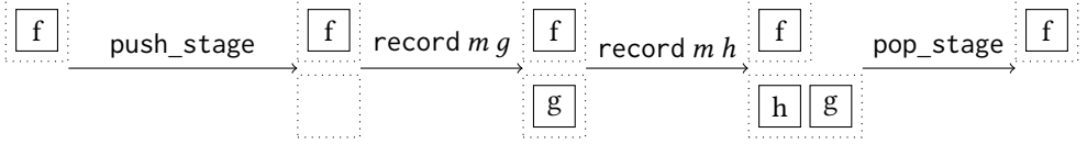
Fig. 6. Effects of the stack manipulation primitives
