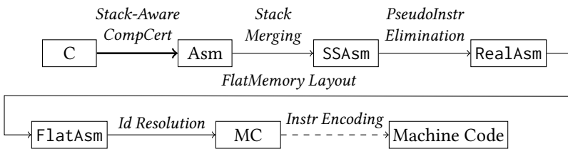
Fig. 10. CompCertMC
