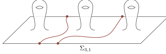
FIG. 7. — A 1-simplex of S'(\Sigma_{3,1})_\bullet .
