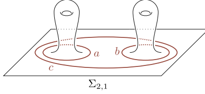
FIG. 4. — Curves such that -\lceil\sigma, \sigma\rceil = t_c t_a^{-1} t_b^{-1}
