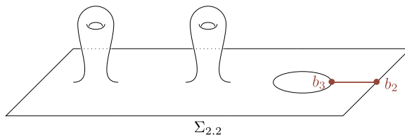
FIG. 9. — A 0-simplex of B_0(\Sigma_{2,2}, b_2, b_3) , with b_2 and b_3 chosen as in case (ii) in the proof of Theorem 4.8
