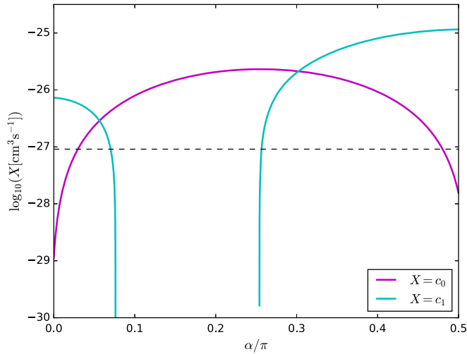
FIG. 6. Dependence of c_0 and c_1 on \alpha : The purple and blue curves show the dependence of c_0 and c_1 on \alpha . The horizontal dotted line corresponds to c_0 \approx 10^{-27} \text{ cm}^3 \text{ s}^{-1} , which is where the \Phi = \Phi_{\text{Fermi}} contour for the idealized case in the right panel of Fig. 5 intersects the c_0 axis. Values of c_0 above the dotted line are constrained by the integrated flux of photons coming from Sgr A*.
