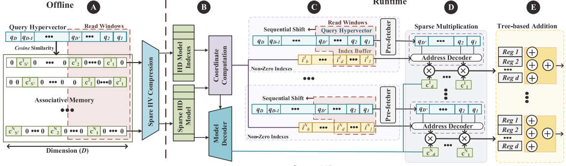
Fig. 6. FPGA implementation of the SparseHD with class-wise sparsity.
