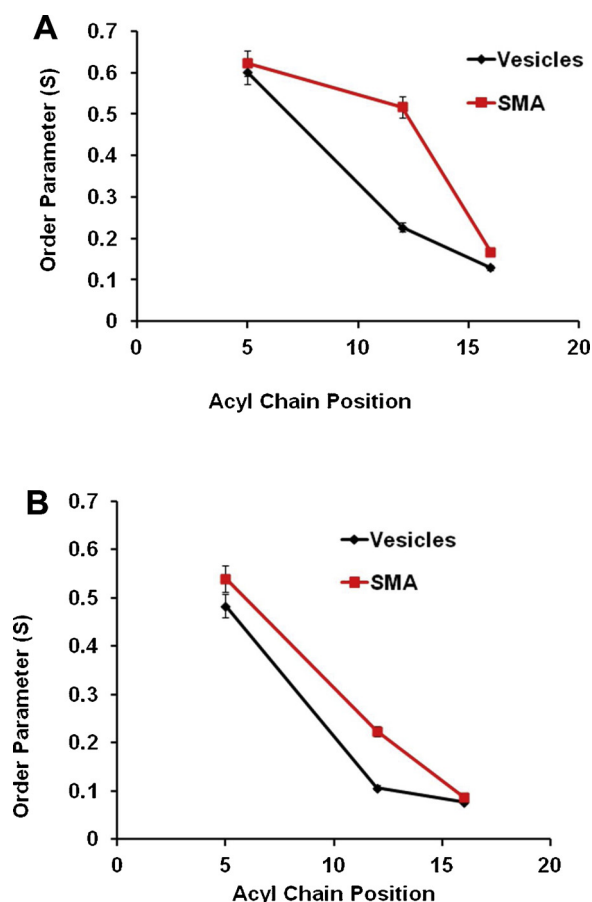
Fig. 5. Order parameter (S) of EPR spectra as a function of spin labeled carbon position in vesicles and with the addition of SMA at temperatures 296 K (23 °C) (A) 318 K (45 °C) (B). The error bars represent uncertainties (standard deviation) arising from the triple batch of sample preparations and data analysis.
