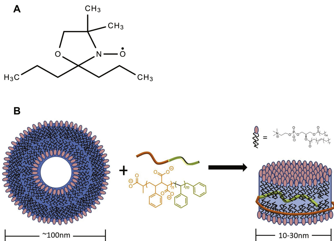
Fig. 1. (A) Chemical structure of the DOXYL lipid spin label probe, (B) Cartoon representation of the addition of a SMA polymer to an intact vesicle and the structural implications of the addition to form the membrane RAFT SMALP.
