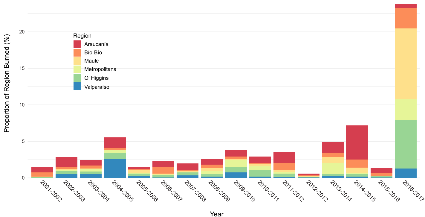
Fig 7. Proportion of each region burned by year. Proportion of each region burned each year (MODIS Collection 6 burned area detections).
