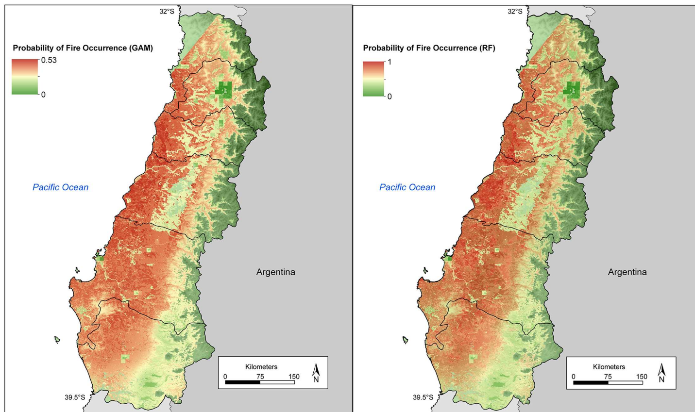
Fig 9. Spatial distribution of the probability of fire occurrence based on best GAM and Random Forests models.
