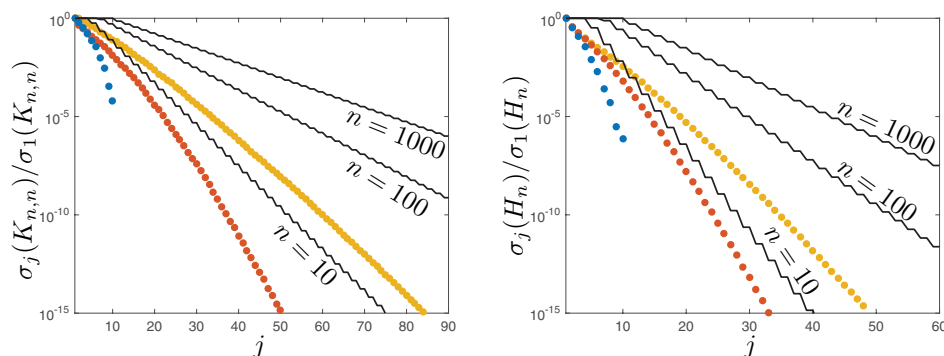
Fig. 5.2 Left: The singular values of the n \times n Krylov matrix (colored dots) compared to the bound in (5.5) for n = 10 (blue dots), 100 (red dots), 1000 (yellow dots). In (5.1) the matrix A is a diagonal matrix with entries taken to be equally spaced points in [-1, 1] and \underline{w} is a random vector with independent Gaussian entries. Right: The singular values of the n \times n real positive definite Hankel matrices (colored dots) associated to the measure \mu_H(x) = \mathbf{1}_{[-1, 1]} compared to the bound in (5.7) for n = 10 (blue dots), 100 (red dots), 1000 (yellow dots).
