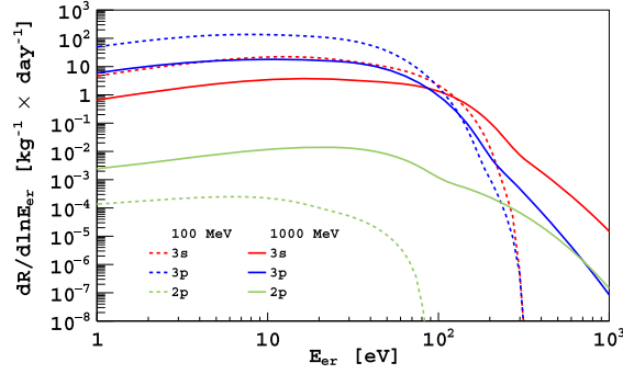
FIG. 1. Contributions of the 3s , 3p , and 2p shells to the DM-electron scattering rate assuming a WIMP-electron cross section of 10^{-36} \text{ cm}^2 and F_{\text{DM}} = 1 for a 100 \text{ MeV}/c^2 DM particle (dashed) and a 1000 \text{ MeV}/c^2 DM particle (solid).
