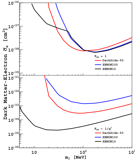
FIG. 4. 90% C.L. limits on the DM-electron scattering cross section for F_{\text{DM}} = 1 (top) and F_{\text{DM}} \propto 1/q^2 (bottom) for DarkSide-50 (red) alongside limits calculated in Ref. [38] using data from XENON10 (black) [50] and XENON100 (blue) [51].
