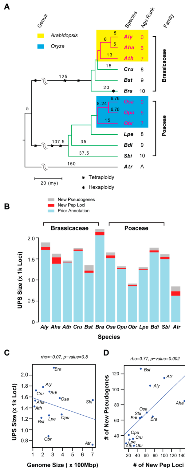
Figure 1. Annotation of the UPS members in Brassicaceae and Poaceae. (A) Phylogenetic relationship of 13 selected species. The tree topology and whole genome duplication events were inferred from literature [29,35]. The age rank is assigned for ordering purpose based on the split time of each species as defined in literature [29]. Species abbreviations in this panel and others are described in Table S2. (B) Comparison of the UPS sizes across 13 plant species. (C) No correlation is present between the genome size and the UPS size in the 13 plant genomes analyzed. Mbp: million base pair. (D) A significant correlation is present between the number of new pseudogenes with the number of new peptide loci in the UPS group of the 13 plant genomes.
