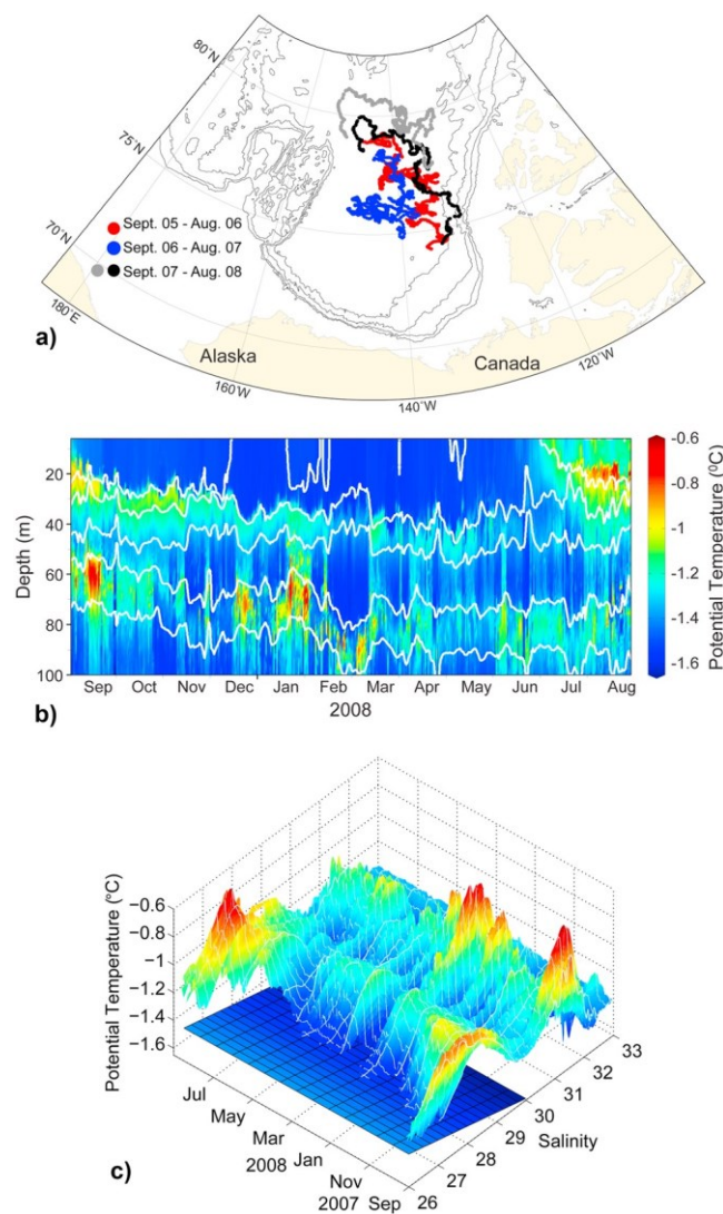
Figure 1. (a) Drift tracks of ITPs that drifted in the Canada Basin (in the region 74°N to 81°N, 130°W to 154°W) between September 2005 and August 2008. In each year, measurements from two ITPs were analyzed (ITP system numbers 1 and 3, 5 and 6, and 8 and 13; see text). (b) Potential temperature-depth time series, where white lines are isohalines (shallowest S = 28 in increments of 1), from ITP 8 (grey track in Figure 1a) from September 2007 for a full year. (c) Evolution of \sigma_t - S structure in the upper ocean (measurements shown in Figure 1b), where the gridded plane indicates the freezing temperature plane.
