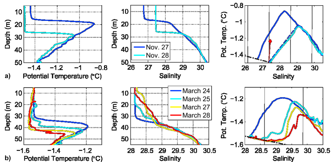
Figure 3. (left column) Potential temperature ( ^{\circ}\text{C} ) and (middle column) salinity profiles, and (right column) corresponding potential temperature-salinity ( \square - S ) plots where the solid black lines are contours of potential density relative to the surface, and the dash-dotted line is the freezing line. (a) ITP 13 profiles for the 2007 days shown. The profiles indicate shear-driven mixing and entrainment of a portion of the warm NSTM layer. The red diamond in the right column is the resulting mixed-layer \square - S derived from homogenizing the initial blue profile to the mixed layer depth of the final cyan profile. The red line is plotted from (2), and its intersection with the freezing line corresponds to the product water of melting sea ice having properties shown by the red diamond. The blue dashed line in the right column is the inferred resulting \square - S profile. (b) Sequence of profiles from ITP 8 (on the 2008 dates shown) indicating ice growth and the injection of cold, salty plumes into the upper ocean.
