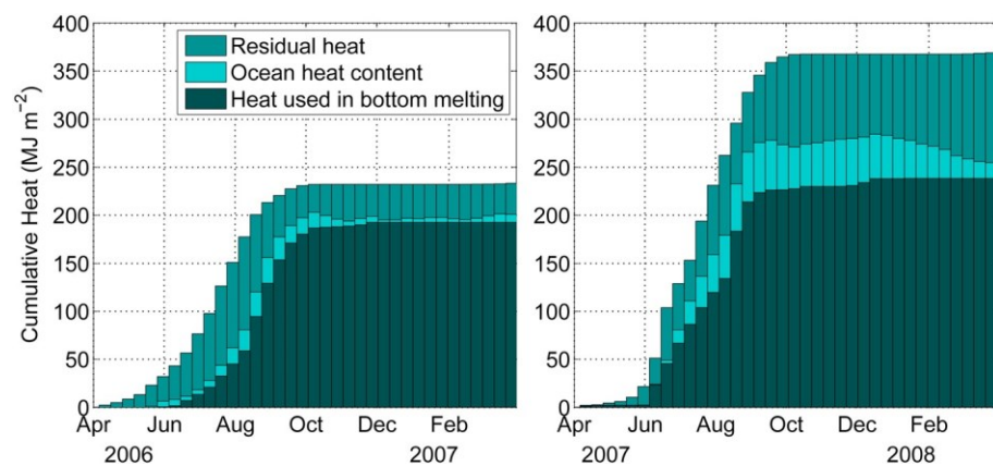
Figure 4. Time series of cumulative heat for (left) 2006–2007 and (right) 2007–2008 for the data shown in Figure 2, where the total height of each bar represents the cumulative solar input to the upper ocean for a bin size of 10 days. The distribution of heat is shown as the sum of heat used to melt ice, the upper ocean heat content (shallower than the warm Pacific layers) in excess of its value at the start of the melt season (computed from the black line in Figure 2, bottom), and the remainder (either heat lost to the atmosphere or heat used to slow the growth of sea ice).
