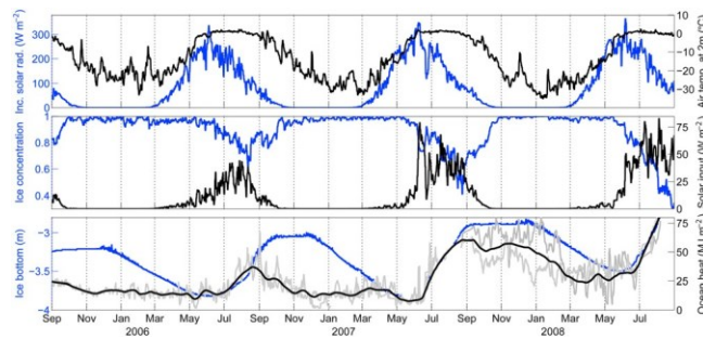
Figure 2. (top) Time series of incident solar radiation ( \text{W m}^{-2} ) and 2 m air temperature ( ^{\circ}\text{C} ) from ERA-40 reanalysis, where values are the areal average in a region bounded by 74^{\circ}\text{N} to 81^{\circ}\text{N} and 130^{\circ}\text{W} to 154^{\circ}\text{W} ; (middle) fractional sea ice concentration (averaged over the same area) and solar input to the surface ocean ( \text{W m}^{-2} , see text for calculation); and (bottom) sea ice bottom position (m) measured by IMBs and ocean heat content ( \text{MJ m}^{-2} ) in the NSTM layer (see text). The grey lines in the bottom panel show ocean heat content for two ITPs in each of the years, and the black line shows the average of these at any given time. Note that most of the bottom melt takes place when the solar warmed water is in contact with sea ice (i.e., before the formation of the summer halocline and underlying NSTM).
