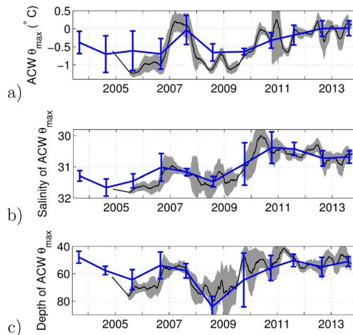
Figure 6. (a) ACW \theta_{max} ( ^{\circ}C ), (b) salinity of ACW \theta_{max} , and (c) depth (m) of ACW \theta_{max} in the CCB. Tick marks on the x axis represent 1 January of each year. ITP data are shown by the black lines: 60 day running means are plotted, and the shading represents one standard deviation. BG CTD data are shown in blue: mean values in a given year are plotted with bars indicating one standard deviation. In most years, CTD stations with an even distribution over the entire CCB (Figure 1) were occupied in the same month.
