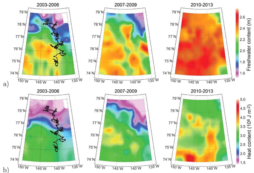
Figure 11. (a) Maps of freshwater content (m) and (b) heat content ( \text{J m}^{-2} ) in the range 31 < S < 33 in the CCB for the years shown. Freshwater content is calculated relative to a reference salinity of 33, and heat content is calculated relative to freezing temperature. The profile locations of ITP 6 between 1 September 2006 and 31 August 2007 are shown on the 2003–2006 period maps.
