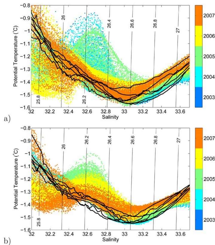
Figure 13. Potential temperature ( h , [°C]) versus salinity ( S ) plots in the region of h - S space for sBSW from (a) mooring B and (b) mooring C. Black lines are BG CTD profiles at each of the mooring sites taken in fall in each year from 2008 to 2013; the entire measurement records from moorings A and D (beginning in 2003 and 2005, respectively) lie in the range of the black profiles shown in each plot (i.e., no sBSW h_{max} is observed at these mooring sites). Labeled contours indicate potential density anomaly ( \text{kg m}^{-3} ) referenced to the surface.
