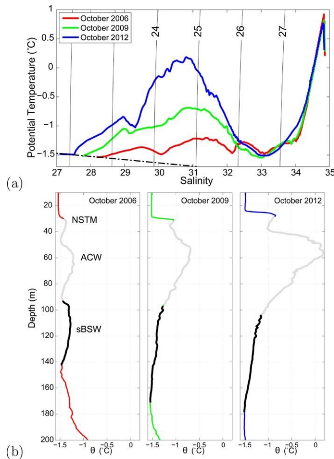
Figure 2. (a) Typical potential temperature ( h , [°C]) versus salinity ( S ) profiles from the CCB (around 78°N, 140°W) in October 2006, 2009, and 2012. Contours indicate potential density anomaly ( \text{kg m}^{-23} ) referenced to the surface (densities vary primarily in accordance with the salinities); the dashed line is the freezing line at 0 dbar. (b) Profiles of potential temperature corresponding to the curves in Figure 2a. The gray and black portions of the profiles mark the salinity ranges found here to be appropriate for the ACW ( 29 < S \leq 32.2 ) and sBSW ( 32.2 < S \leq 33 ), respectively. Notice in the latter 2 years, the absence of a maximal temperature in the salinity range of sBSW.
