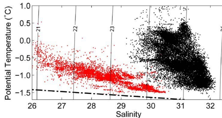
Figure 4. Potential temperature versus salinity plot of h_{max} and corresponding salinity (for all CTD and ITP profiles [2003–2013] in the CCB) where the red dots indicate the shallowest temperature peak in the upper 40 m and the black dots indicate the warmest temperature peak that is deeper than 40 m with S < 32.2 . The two clusters show a clear delineation between the NSTM (red dots) and the ACW h_{max} (black dots).
