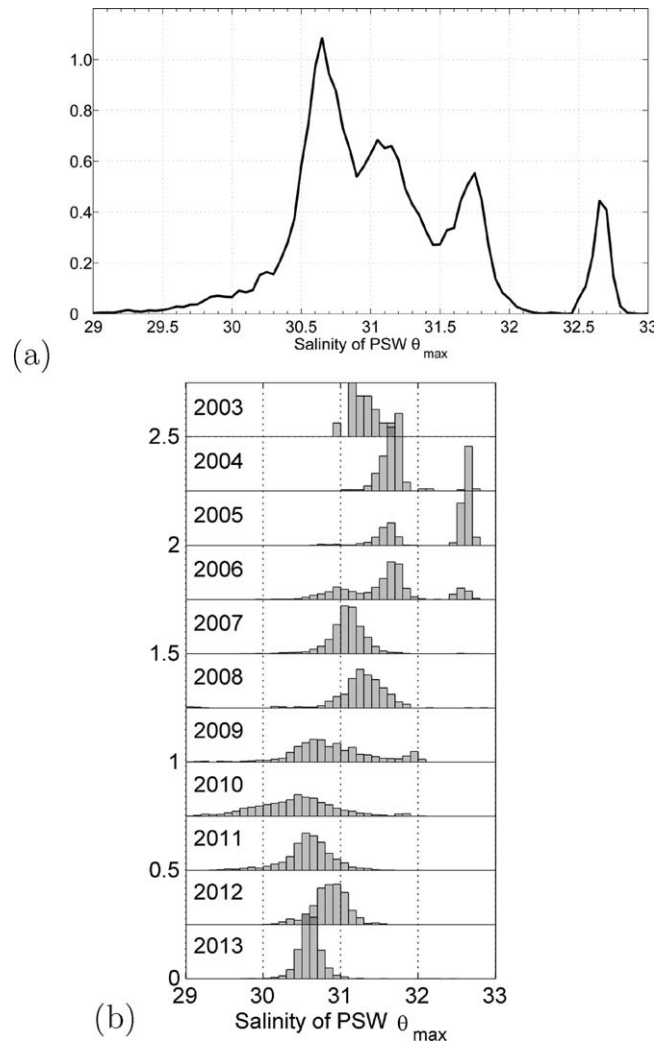
Figure 3. (a) PDF of the salinity of the h_{max} for S < 33 and deeper than 40 m for all CTD and ITP profiles (2003–2013) in the CCB. A binsize of 0.05 is used in the calculation. (b) Yearly histograms of the salinity of the h_{max} . Binsize is 0.1 and number in each bin is divided by the total number of observations in a given year. Each year is offset on the y axis by 0.25.
