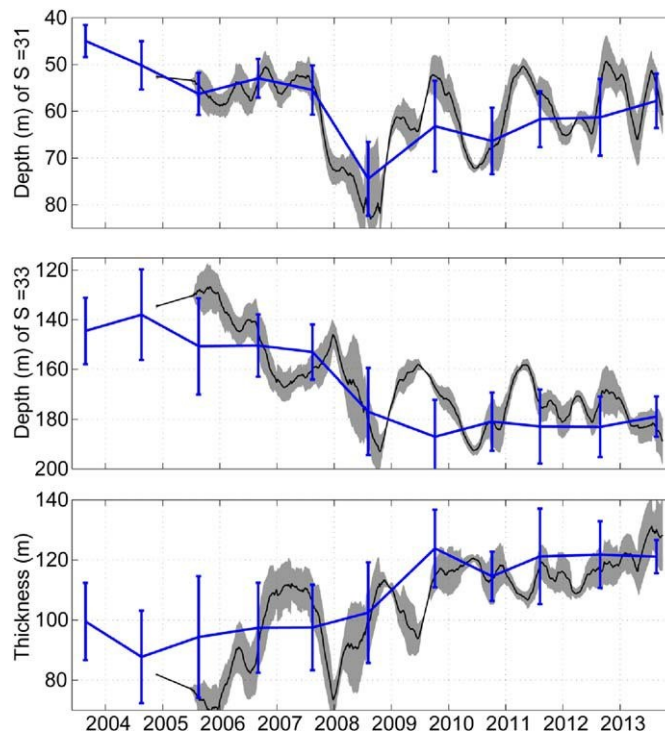
Figure 9. Depth (m) of the (top) S = 31 and (middle) S = 33 isohalines, and (bottom) thickness of the layer defined by 31 < S < 33 in the CCB. BG CTD data are shown in blue: mean values in a given year are plotted with bars indicating one standard deviation. ITP data are shown by the black lines: 60 day means are plotted, and the shading represents one standard deviation.
