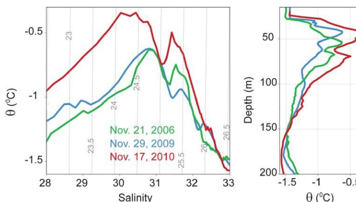
Figure 5. (left) Potential temperature versus salinity in the CCB for the dates shown. Contours indicate potential density anomaly ( \text{kg m}^{-3} ) referenced to the surface. Two temperature peaks can be seen in the salinity range of the ACW ( 29 < S < 32 ). Cooler sBSW peaks are present (before 2009) around a salinity of 32.4. (right) The corresponding potential temperature profiles showing the two peaks (in the ACW salinity range) in each profile between around 45 and 65 m depth.
