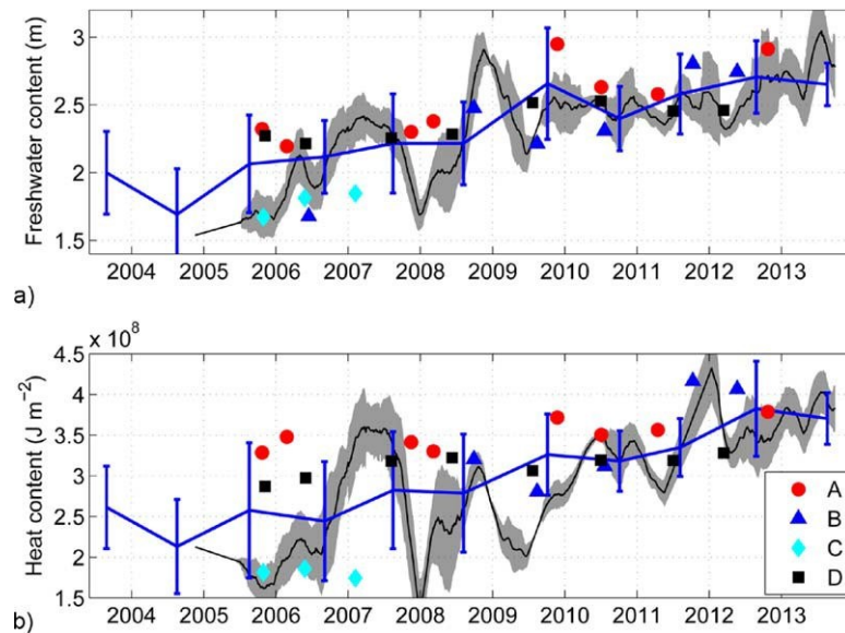
Figure 8. (a) Freshwater content (m) and (b) heat content ( J m^{-2} ) in the range 31 < S < 33 in the CCB. Waters fresher than S \leq 31 are not considered as in early years, the NSTM lies at the fresh end of the salinity range that encompasses the ACW for all years. Freshwater content is calculated relative to a reference salinity of 33. Heat content is calculated relative to freezing temperature. BG CTD data are shown in blue: mean values in a given year are plotted with bars indicating one standard deviation. ITP data are shown by the black lines: 60 day running means are plotted, and the shading represents one standard deviation. Mean values from each of the four BGOS mooring A, B, C (2003–2008), and D deployments are shown by the symbols (each symbol is plotted at the mean date for which MMP profiles were obtained during the yearly deployments).
