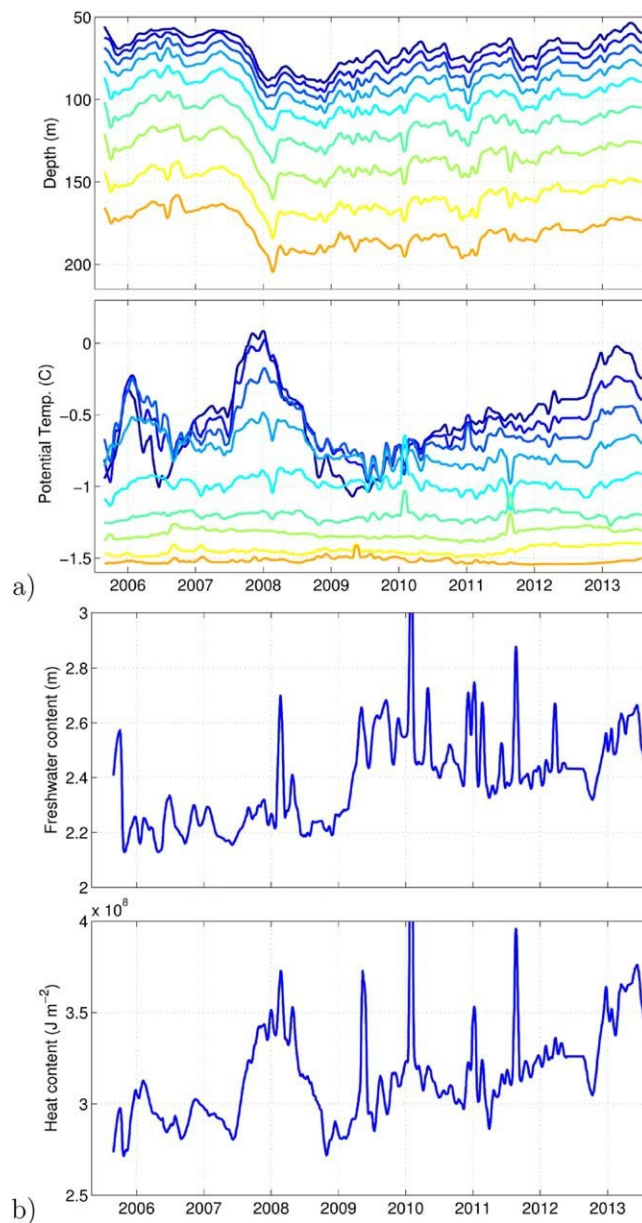
Figure 10. (a) Top: mooring D (75°N, 140°W) depth of selected isohalines S 31 to 33, with spacing of 0.25. Bottom: potential temperature (°C) on isohalines shown in the top plot. Mooring D was only deployed starting in 2005. Seasonal variability of isohaline depths is related to intensified wind-stress curl in winter with no apparent seasonal variability in temperature on these isohalines. (b) Freshwater content (m) (top) relative to S 33 and heat content (J m -2 ) calculated relative to freezing temperature in the range 31 < S < 33; 30 day running averages are plotted. Narrow peaks and troughs can be attributed to mesoscale eddies; values for the two peaks that extend beyond the plot ranges are 3.2 m (top) and 4.53 × 10 8 J m -2 (bottom).
