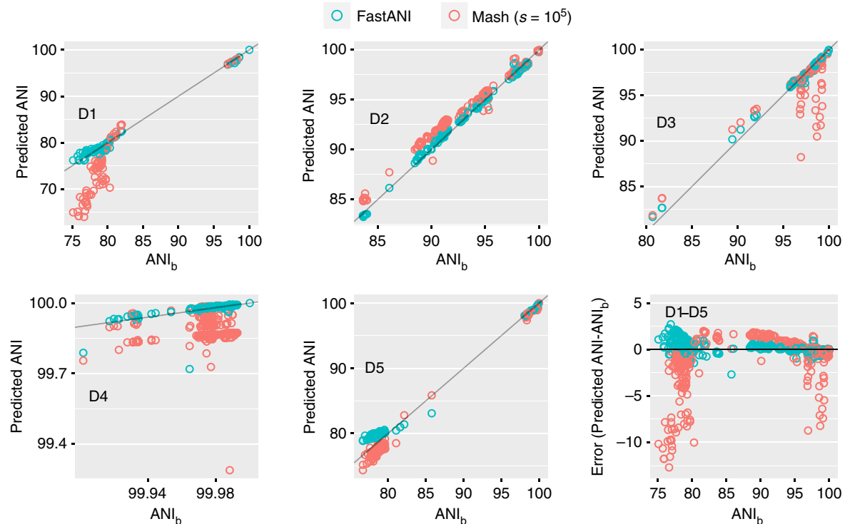
Fig. 1 Correlation of FastANI and Mash-based ANI output with ANI b values for datasets D1–D5. Because FastANI assumes a probabilistic identity cutoff that is set to 80% by default, it reports 76, 570, 4271, 464, and 130 genome matches for the individual queries in datasets D1–D5 respectively. To enable a direct quality comparison against FastANI, Mash is executed for only those pairs that are reported by FastANI. Notice that each dataset encompasses a different nucleotide identity range (x-axes). Gray line represents a straight line y = x plot for reference. Pearson correlation coefficients corresponding to these plots are listed separately in Table 2. Last plot shows error of these methods w.r.t. ANI b using all five datasets
