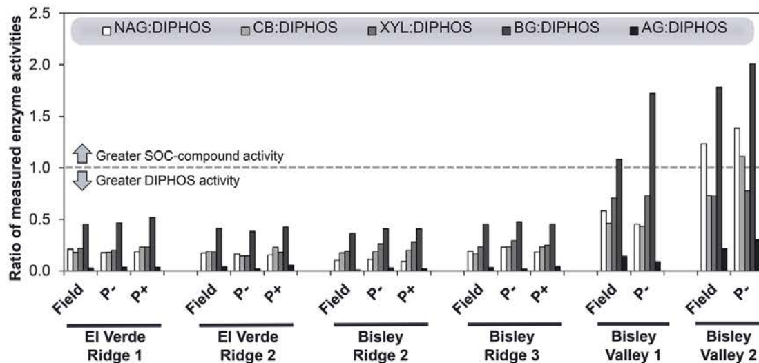
Fig. 2. Relative enzymatic activity for soils from field (Field), control incubations (P-), and incubations amended with phosphorus (P+). Values are expressed as the ratio between various soil organic carbon-specific enzyme activities and the activity of phosphodiesterase (DIPHOS; see key on the top). Labels are AG:α-glucosidase, BG:β-glucosidase, CB:β-D-cellubiosidase, NAG:N-acetyl-β-glucosaminidase, XYL:β-xylosidase, DIPHOS:Phosphodiesterase. Incubation endpoints and the corresponding field soils used for enzyme assay analysis can be found in Fig. S2. Numbers (i.e., 1, 2, or 3) preceding site names correspond to the unique ~1 kg replicate samplings taken at each site.
