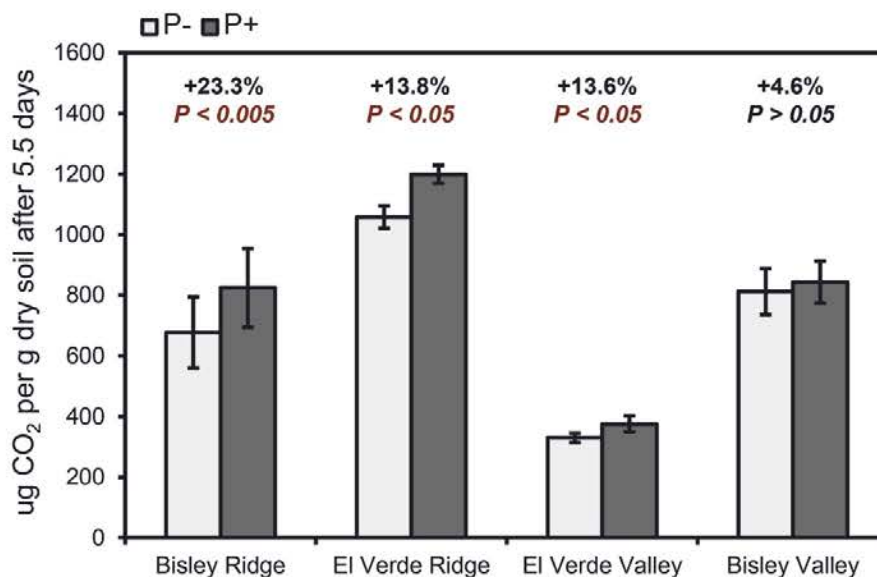
Fig. 1. Cumulative CO 2 respired after ~5.5 days of incubation for soils without (P–, light gray) and with (P+, dark gray) exogenously added phosphorus. Bars denote the mean CO 2 respired ( \pm the standard error of the mean) for control incubations vs. incubations amended with exogenous phosphate as 30 mg PO 4 3- -P per kg, for soils sampled from each of the four locations, based on five replicate incubations for each site and experimental condition. See also Fig. S2 for incubation layout.
