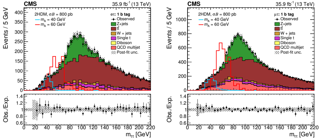
Figure 2. Measured m_{\tau\tau} distribution in the e\tau_h (left), and \mu\tau_h (right) channel, compared to the expected SM background contributions. The signal distributions for b\bar{b}A with a pseudoscalar mass of 40 and 60 GeV are overlaid to illustrate the sensitivity. They are normalized to the cross section times branching fraction of 800 pb. The uncertainty bands represent the sum in quadrature of statistical and systematic uncertainties obtained from the fit. The lower panels show the ratio between the observed and expected events in each bin.
