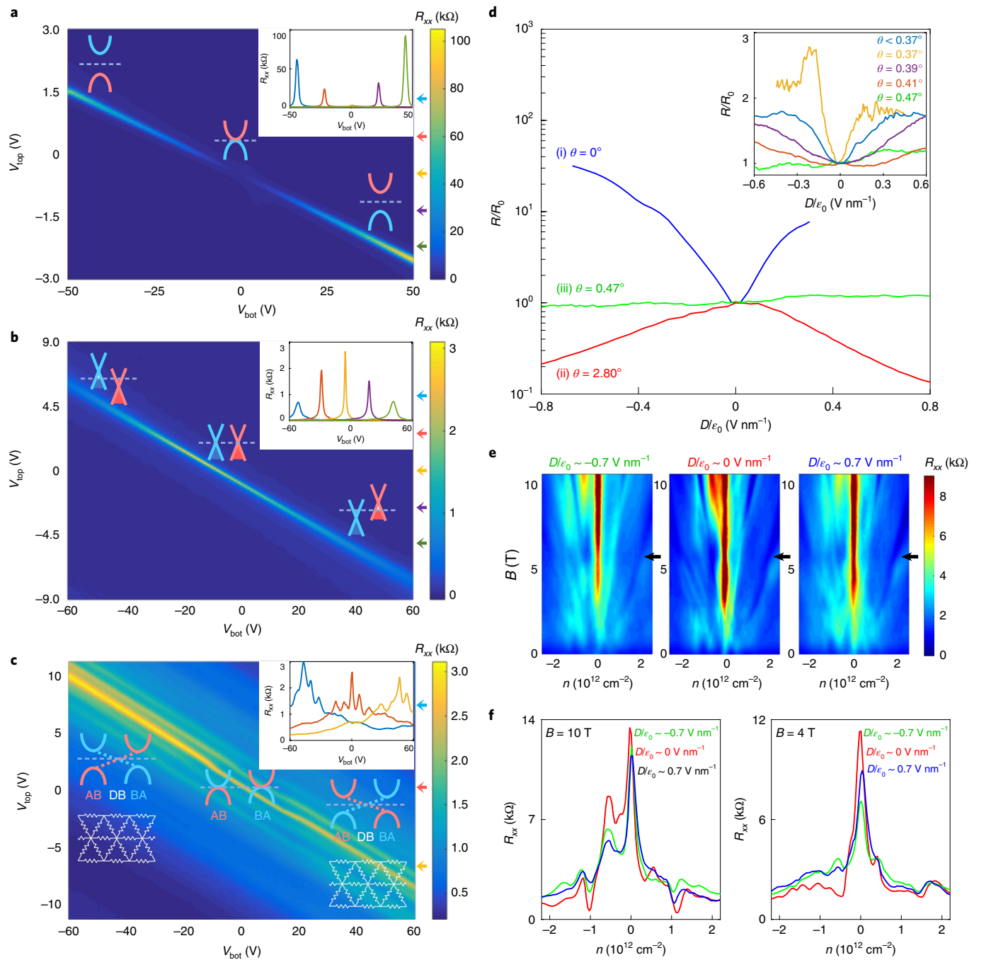
Fig. 3 | Transport properties of BLG with a controlled twist angle. a–c, The top- and bottom-gate dependence of the longitudinal resistance R_{xx} in Bernal-stacked BLG ( a ), large-angle TBG (2.8°) ( b ) and small-angle TBG (0.47°) ( c ). The insets in the top right corner show several line cuts at fixed top-gate voltages marked with coloured arrows on the right side of the main panels. Schematic band structures in the inset show how the band structures change as a function of the perpendicular electric displacement field, D . The schematic diagram of the triangular network of resistors in c represents the current paths generated along the domain boundaries obtained by gapping out AB and BA domains with transverse electric field. DB denotes the domain boundaries. d , Normalized Dirac peak resistances as a function of transverse displacement field obtained from a–c . The inset shows a linear-scale plot of normalized Dirac peak resistances as a function of the electric displacement field, D , for small-angle TBG devices. e , Displacement field-dependent Landau fan diagrams showing longitudinal resistance R_{xx} . The fan diagrams shown in the left, middle and right panels were obtained at the displacement field D/\epsilon_0 \approx -0.7, 0 and 0.7 V nm ^{-1} , respectively. f , Displacement field-dependent longitudinal resistance R_{xx} acquired at constant B = 10 T (left) and 4 T (right). Green, red and blue curves correspond to the displacement field D/\epsilon_0 \approx -0.7, 0 and 0.7 V nm ^{-1} , respectively. All the transport measurements were performed at 1.7 K.
