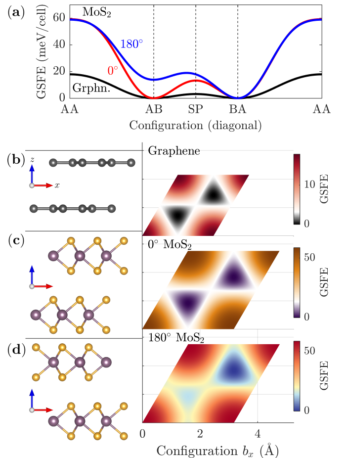
FIG. 3. (a) The generalized stacking fault energy (GSFE) evaluated on stackings sampled along the unit-cell diagonal for three different bilayers. (b)–(d) Side views of the ground-state stacking orientation for each bilayer, and corresponding GSFE dependence on configurations in the unit-cell \Gamma . The color scale in each case is chosen to make the saddle point (SP) energy white or bright yellow.
