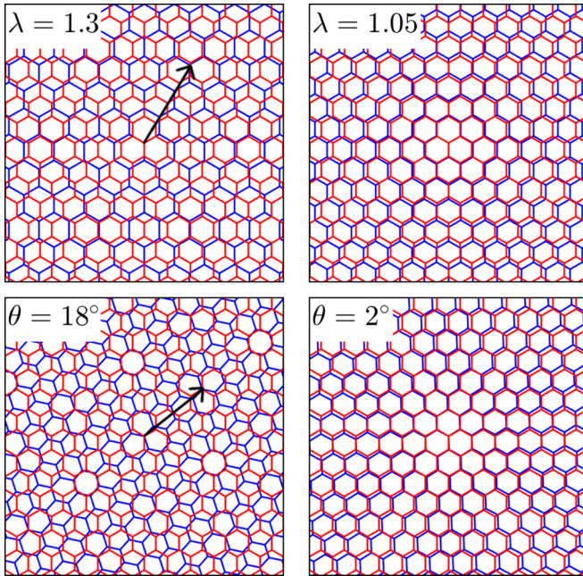
FIG. 2. Examples of misaligned lattices. Top panels show bilayers whose lattice constants differ by a factor of \lambda while the bottom panels show bilayers with a relative twist angle \theta . The left panels show misaligned structures with small moiré length (moiré wavelength given by the black arrow), while the right panels show nearly aligned structures with large moiré length.
