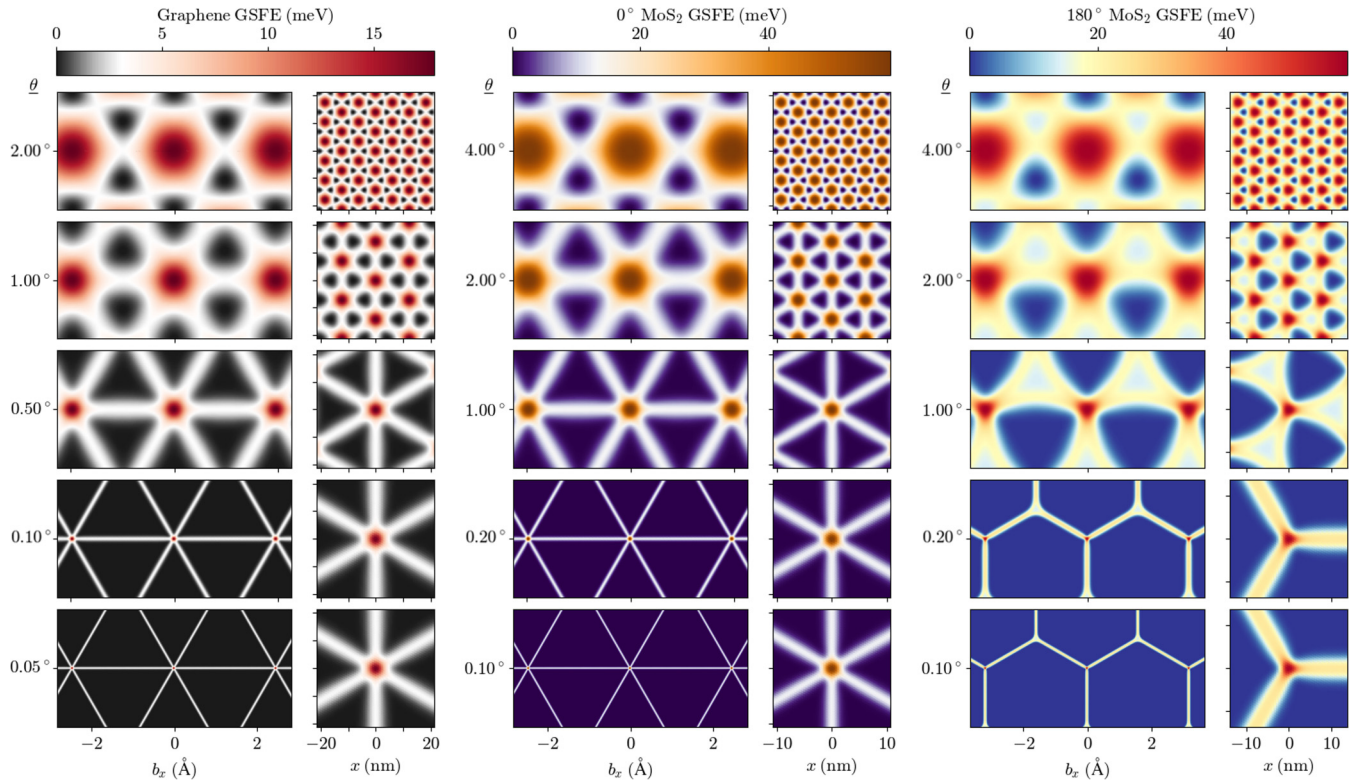
FIG. 5. Configuration relaxation results for twisted bilayers with five incommensurate twist angles each. The left panel of each column shows V_{\text{GSFE}}[\mathbf{b} + 2\mathbf{u}(\mathbf{b})] over \Gamma (the relaxation pattern in configuration space) and the right panel shows V_{\text{GSFE}}(\mathbf{r}) (over real space).
