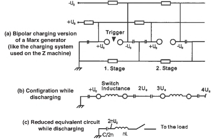
Fig. 12. The operating principles of a bipolar Marx generator. The Marx generators on the Z machine are bipolar. Relative to the unipolar Marx generator (Fig. 11), the bipolar Marx generator requires half the number of stages/switches, which reduces the Marx generator's overall size, cost, and inductance. (a) Prior to the discharge triggering event, the capacitors are charged in parallel at a charging voltage of either +U_0 or -U_0 , and the gas-filled spark-gap switches are in an open state. (b) Upon the triggering event, the switches close, and the capacitor configuration changes from parallel to series. (c) A reduced equivalent circuit after the triggering event. Note that the n shown here for the bipolar circuit would be half the value of the n shown for the unipolar circuit of Fig. 11 when generating the same total output voltage. (Figure source: Ref. [83].)
