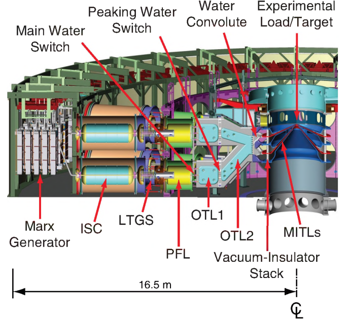
Fig. 9. Cross-sectional drawing of one radial half of the Z pulsed-power facility (this is not an LTD facility). The various components/stages are described in the text. A zoomed-in drawing of the vacuum section (containing the water-vacuum insulator stack, the MITLs, and the experimental load/target region) is provided in Fig. 10. (Figure source: Ref. [80].)
