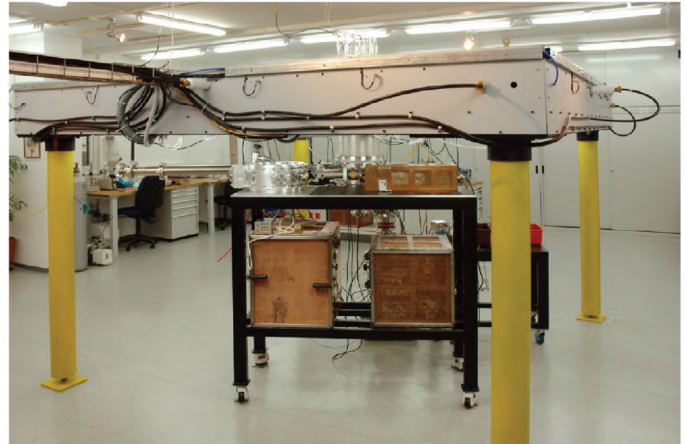
Fig. 29. Photograph of the 500-kA, 500-ns LTD at the Weizmann Institute of Science in Israel.
