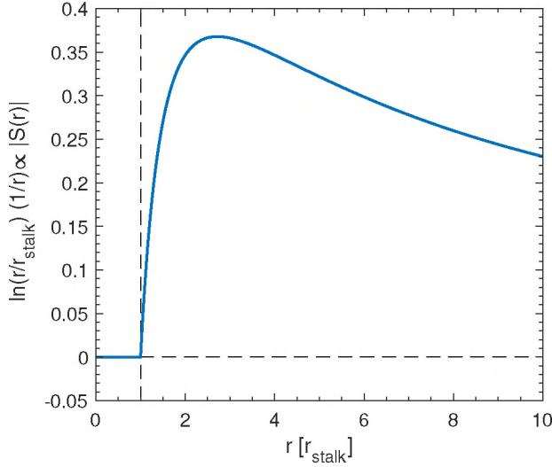
Fig. 8. Plot of \ln(r/r_{\text{stalk}}) \cdot (1/r) , which is proportional to |S(r)| for the stationary (non-imploding) cavity illustrated in Fig. 1(a). The r axis is in units of r_{\text{stalk}} . The Poynting flux is maximal at r = e \cdot r_{\text{stalk}} = 2.71828 \cdot r_{\text{stalk}} and goes to zero at r = r_{\text{stalk}} .
