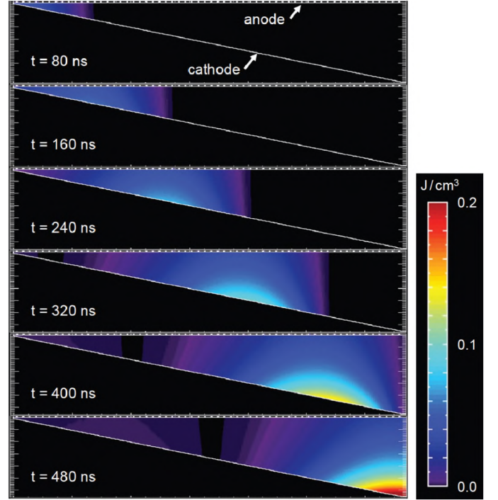
Fig. 21. 2D LSP simulation results illustrating an electromagnetic pulse propagating down an impedance-matched LTD module with very little back reflections. (Figure source: Refs. [116], [117].)
