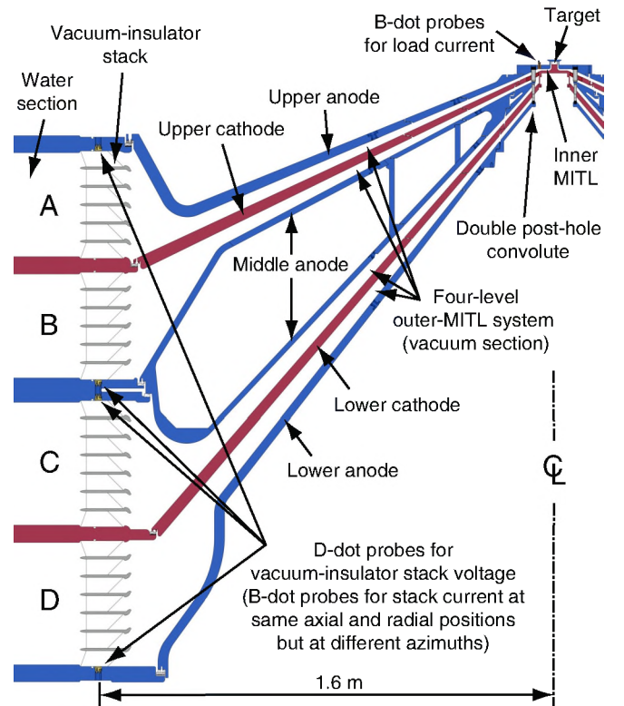
Fig. 10. Cross-sectional drawing of one radial half of the Z vacuum section. (Figure source: Ref. [80].)
