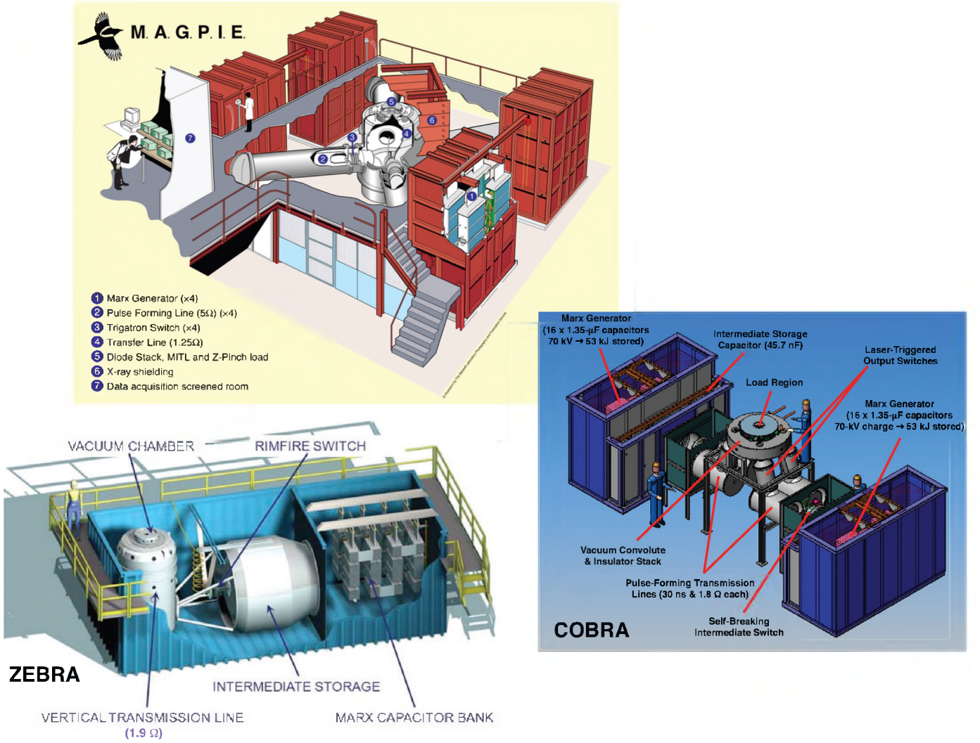
Fig. 15. Graphical representations of some of the largest university-scale ( \sim 1 MA) Marx-generator/PFL-based facilities used for studying HEDP (these are not LTD facilities). Shown are the \sim 1 -MA, 250-ns MAGPIE generator at Imperial College, UK [100], [101], the \sim 1 -MA, 100-ns ZEBRA generator at the University of Nevada, Reno [102], [103], and the \sim 1 -MA, 100-ns COBRA generator at Cornell University [104].
