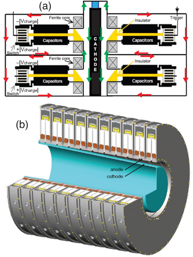
Fig. 19. (a) A schematic representation of two LTD cavities stacked on top of one another to form a 2-cavity LTD module. (Figure adapted from source in Ref. [32].) This axisymmetric cross-sectional representation illustrates how the desired load current channel (green arrows) flows relative to the undesired, parasitic current channels (red arrows). (b) A 10-cavity LTD module design by Sandia National Laboratories. Here one can see the output gaps from each cavity stacked on top of one another, forming the anode path, which surrounds the central cathode stalk. Stacking the output gaps in series like this increases the voltage of the overall driver (think of batteries being stacked on top of one another with the \pm polarities all aligned). Additionally, and again because of the series configuration, the inductances of the cavities add together, while the effective capacitance of the module is reduced. Thus, the characteristic impedance of the module is proportional to the number of cavities in the module. (Figure source: Ref. [36].)
