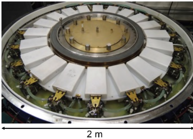
Fig. 31. Photograph of the \sim 1 -MA, 200-ns LTD-III generator [138], which is now being assembled at the University of California, San Diego.
