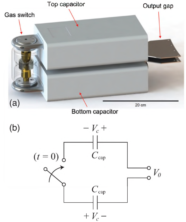
Fig. 17. (a) A Sandia brick design capable of storing up to 800 J of electrical energy and supplying up to 5 GW of electrical power. (b) An equivalent circuit model for a single brick.
