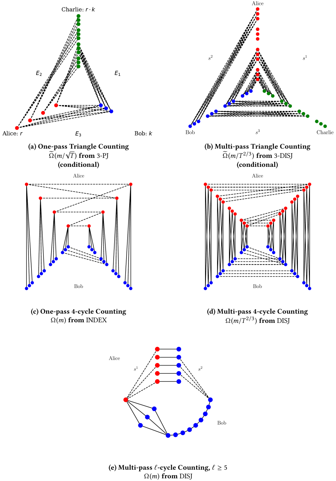
Figure 1: Lower bound constructions.
