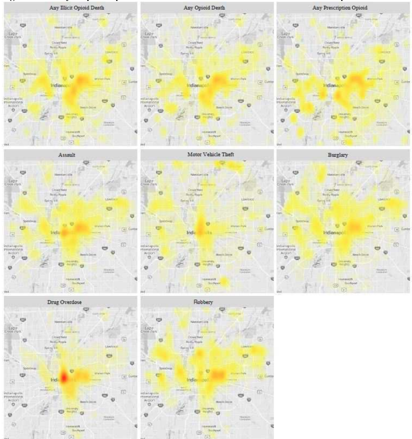
Figure 2: Density Maps of Opioid Death Concentrations within Other Incident Hot Spots
