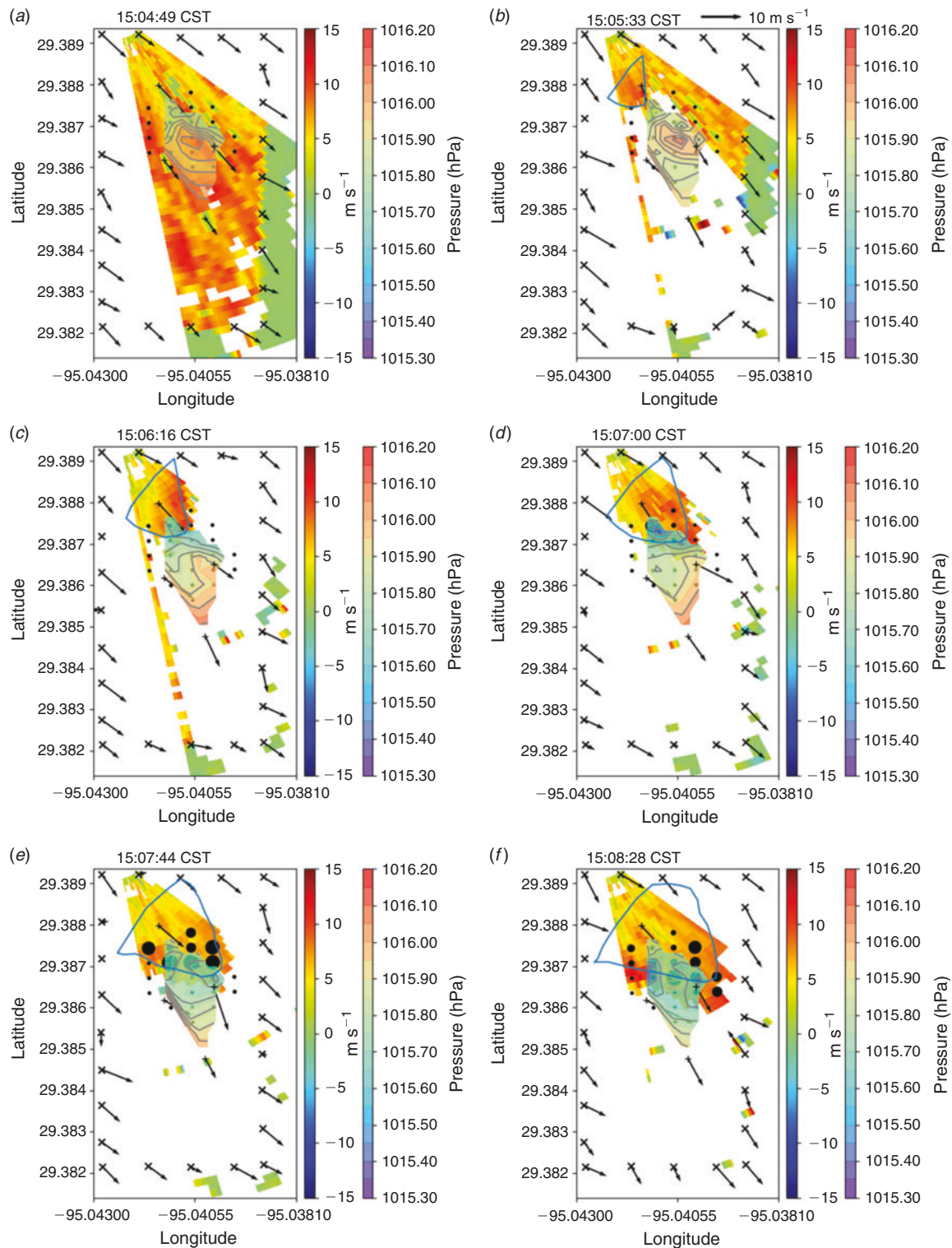
Fig. 15. Composite of surface winds from tower and anemometer arrays (vectors), Doppler lidar radial velocities (shading), 3-m barometric surface pressure (shading and contours) and soil surface temperature (black dots; larger size indicates higher temperature). The estimated fire perimeter (indicated by single blue outline) was derived from infrared temperature data obtained from the observation tower.
