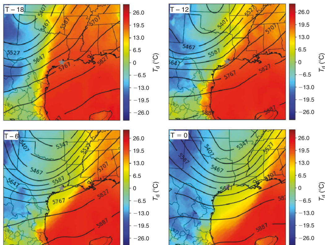
Fig. 8. North American Regional Reanalysis (NARR) 500-hPa geopotential height (contours) and surface dew point, T_d (shading). The geopotential height contours are in increments of 60 geopotential m. These data show the progression of the trough and cold front (dewpoint boundary) across Texas in the 18 h preceding ignition where T -18 is 2100 CST (Central Standard Time) on 29 Jan 2013, T -12 is 0300 CST on 30 Jan, T -6 is 0900 CST on 30 Jan, and T = 0 is 1500 CST on 30 Jan.
