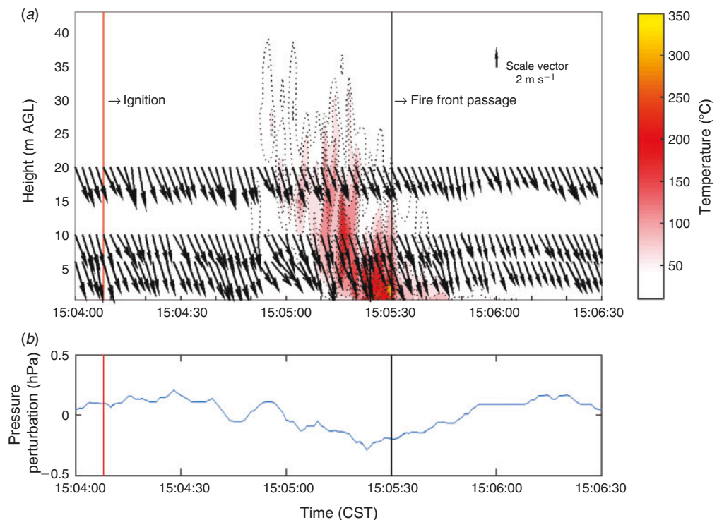
Fig. 14. Time height plot of thermodynamic plume structure, winds and surface pressure perturbation, measured at the 43-m tower. (a) Thermocouple temperatures (shading and contours) and horizontal wind vectors 5.8, 10 and 20 m AGL; and (b) the pressure perturbation, p' time series is shown in the lower panel. The vertical red line is the time of ignition and the black vertical line is the time of fire front passage.
