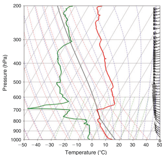
Fig. 11. Radiosonde sounding taken at 1424 CST (Central Standard Time) just before ignition on 30 January 2013. The red line represents the temperature and the green line the dew point.
