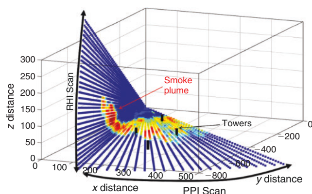
Fig. 4. Schematic of lidar scanning strategy. The L-pattern allowed horizontal plan position indicator (PPI) scans across the fire front and the vertical range height indicator (RHI) scan captured the plume structure along the flank of the fire. Data shown are lidar backscatter intensity.
