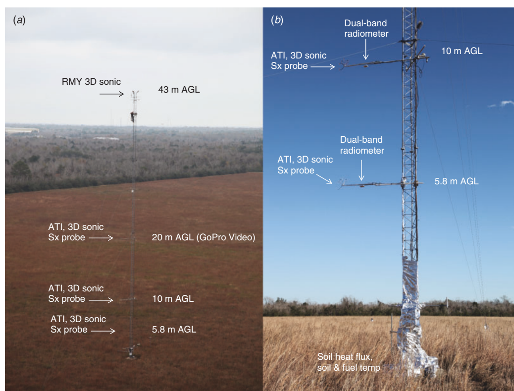
Fig. 2. Photos of the 43-m tower showing the arrangement of the sonic anemometers on the tower (a); and a close-up of the first 10 m of the tower (b) (ATI, Applied Technologies, Inc.).
