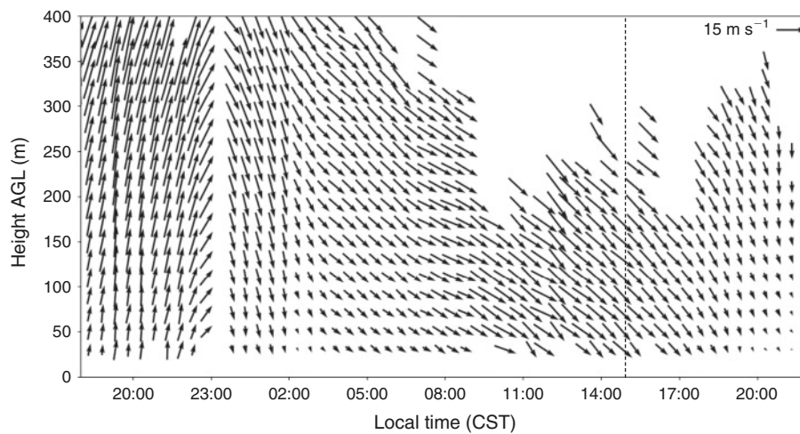
Fig. 10. Time–height plot of vertical wind profiles obtained from the Doppler sodar located next to the burn unit, near the University of Houston Atmospheric Laboratory (Fig. 1). Data are from 29–30 January 2013. Dashed line indicates time of ignition.
