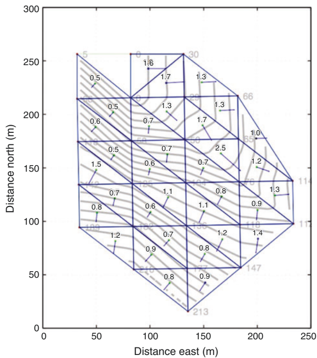
Fig. 13. Rate of spread vector calculation made from 25 HOBO ground thermocouples: arrival times (s) at each HOBO, isochrones at 10-s intervals, ROS (rate of spread) vectors and ROS speed.
