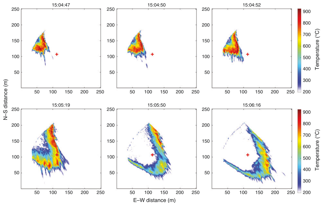
Fig. 6. Series of geo-referenced infrared (IR) temperature ( ^\circ\text{C} ) observations from the 40-m observation tower located north of the unit boundary. Red cross shows location of the 43-m tower inside of the burn unit (see Fig. 1 for locations of all towers). Times are HH:MM:SS (Central Standard Time, CST).
