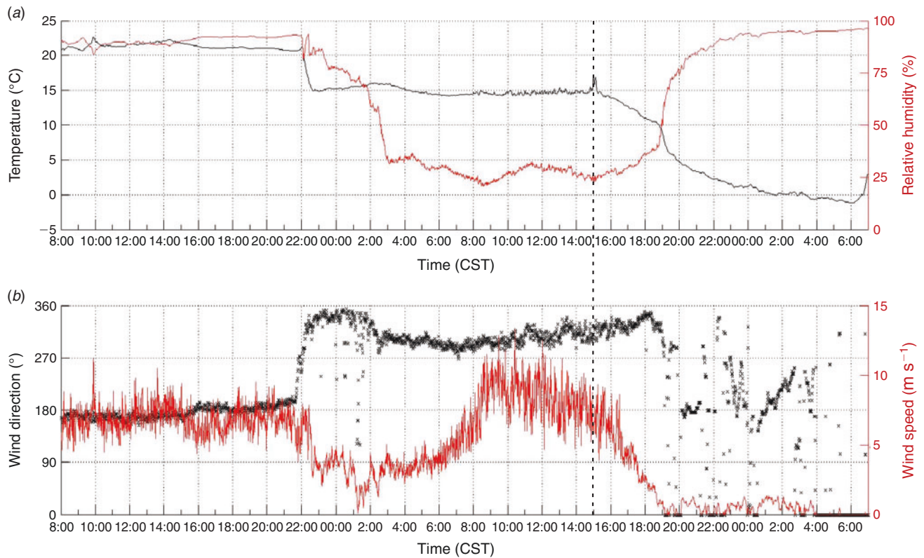
Fig. 9. Time series of temperature, relative humidity (a), surface wind speed and wind direction (b) for 29–30 January 2013 taken from the University of Houston Atmospheric Laboratory located on the western edge of the burn unit (Fig. 1, sodar location). Ignition time is marked by the vertical dashed line.
