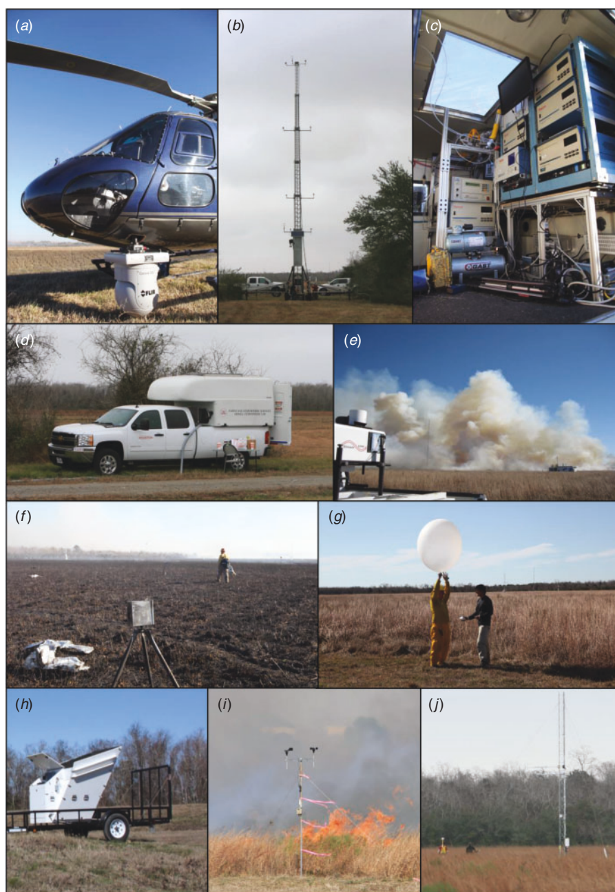
Fig. 3. (a) Helicopter-mounted FLIR camera and gimble system (Corona 350); (b) 32-m California State University Mobile Atmospheric Platform System (CSU-MAPS) tower; (c) mobile air quality instruments; (d) mobile air quality laboratory; (e) Doppler lidar; (f) fire behaviour video package; (g) radiosonde release; (h) ART VT-1 sodar; (i) cup anemometer on burn unit perimeter; (j) 10-m interior tower.
