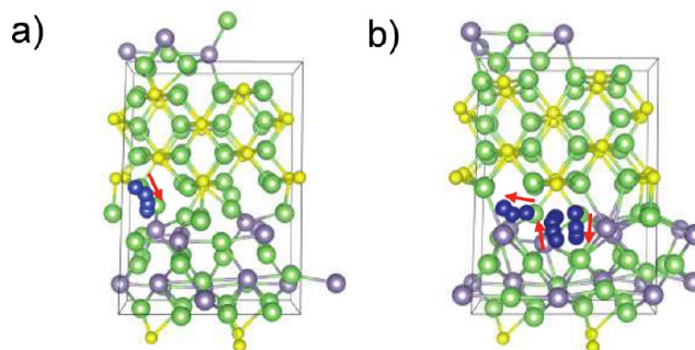
Figure 11. Mechanism of Li + diffusion (a) for a < 0.1 eV barrier at the Li 2 S/Li 3.5 Sn interface and (b) for a 0.3 eV barrier within a Li 3.5 Sn crystallite. Blue spheres and red arrows show exemplary Li + paths.
