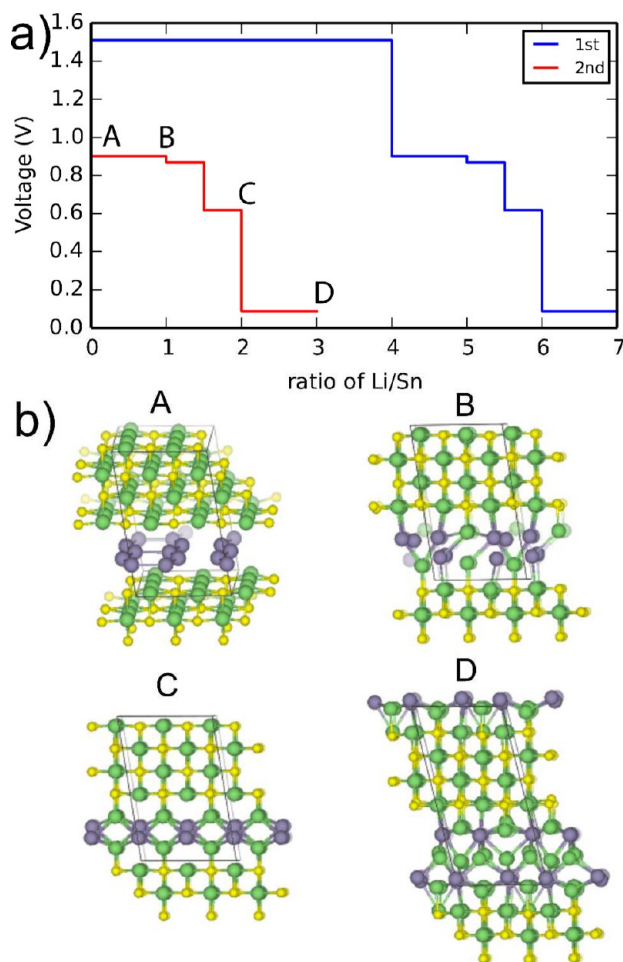
Figure 10. (a) Calculated voltage profiles of the first and second lithiation cycles of the SnS 2 . (b) Sandwich structures along the convex hull determining the voltage profile. Green spheres are Li + ; yellow are S 2- ; and gray are Sn.
