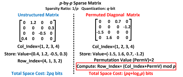
Fig. 4: Storage requirement comparison.
