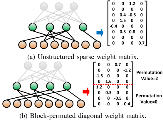
Fig. 1: Weight representation by using (a) conventional unstructured sparse matrix. (b) block-permuted diagonal matrix.
