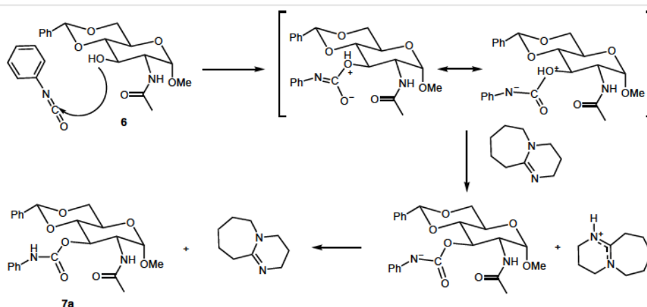
Scheme 2 Proposed mechanism of the reaction
