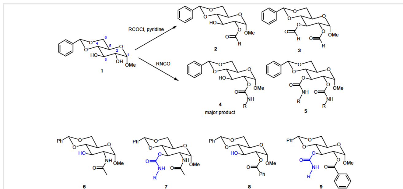
Scheme 1 Selective acylation of 4,6-O-benzylidene methyl \alpha -D-glucopyranoside and the structures of the targeted 3-carbamate sugar derivatives 7 and 9 and their precursors
