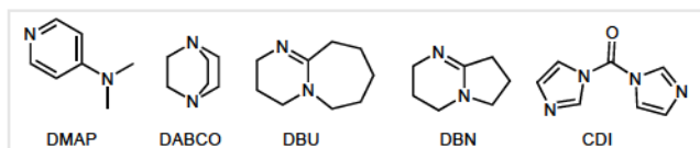
Figure 1 Structures of organic bases and reagents useful for carbamate formation
