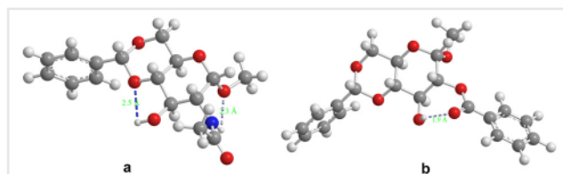
Figure 2 The energy-minimized structures of compounds 6 (a) and 8 (b)
