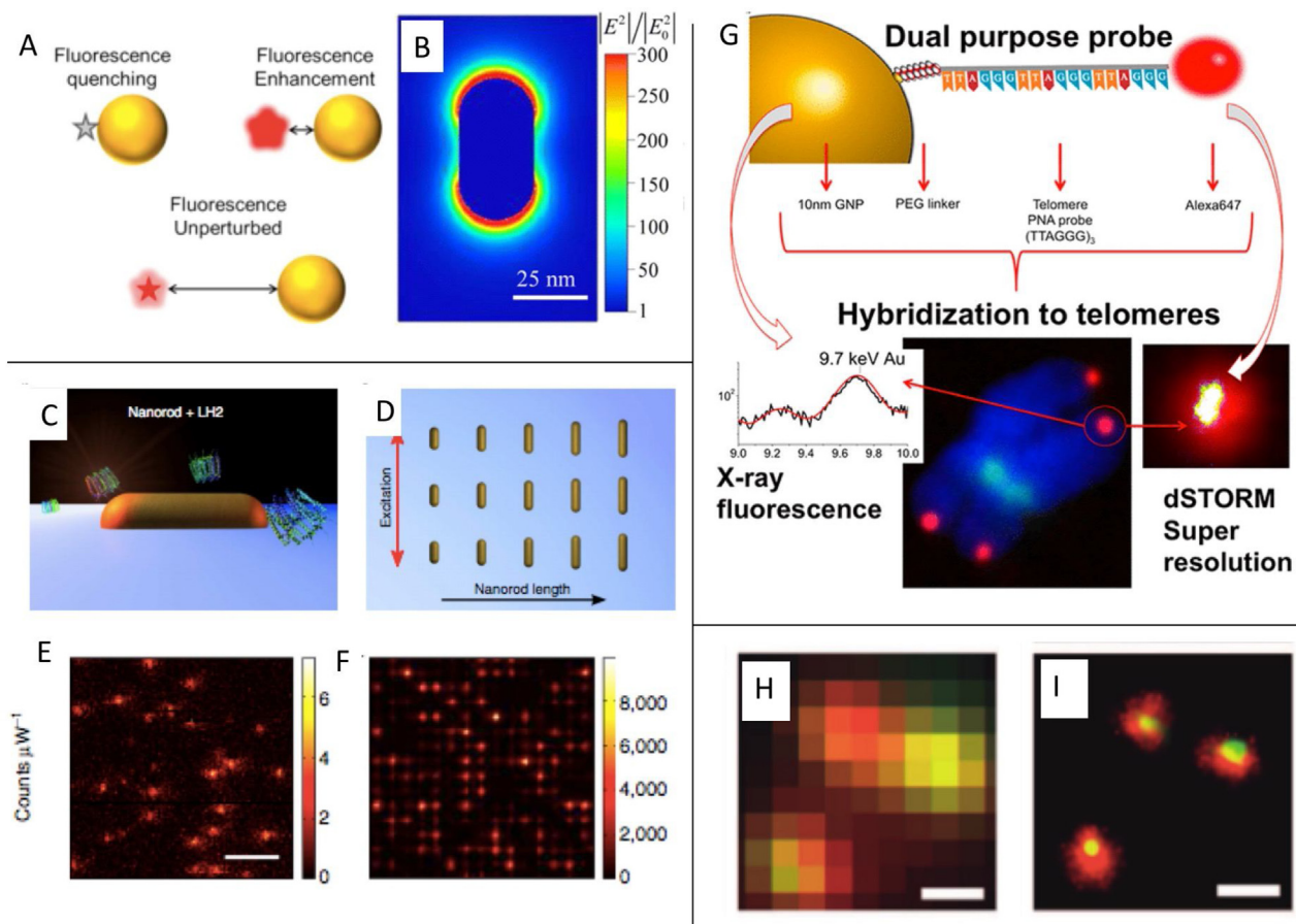
Fig. 10. (A) Plasmon-enhanced fluorescence (PEF) working principle. Printed with permission from American Chemical Society [129]. (B) PEF of individual AuNR for single molecule detection. Printed with permission from American Chemical Society [136]. (C–F) AuNR arrays for studying the light harvesting complex 2 protein. C shows the schematic of an AuNR with an LH2 complex at the hot spot. D is a schematic figure of the AuNRs array. E and F are Fluorescence images of LH2 complexes on the surface of PVA (E, without AuNRs) and on the surface of AuNR arrays (F). Printed with permission from Springer Nature [137]. (G) AuNPs with DNA points accumulation for imaging in nanoscale topography (DNA-PAINT) for determining the telomeres distance. Printed with permission from American Chemical Society [144]. (H–I) the difference in resolution of (H) a wide-field and (I) a STORM image for protein corona. Scale bar: 200 nm. Printed with permission from John Wiley and Sons [146].
