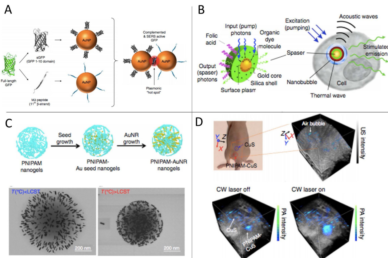
Fig. 14. (A) Schematic of assembly of AuNPs by green fluorescent protein (GFP) and M3 peptide fragments to form hot-spot SERS and photoacoustic nanoprobe. Printed with permission from Springer Nature [185]. (B) Schematic of spacer for PA imaging. Printed with permission from Springer Nature [186]. (C and D) poly (n-isopropyl acrylamide) (PNIPAM)-AuNR for enhancing PA signal. (C) The schematic and transmission electron microscope (TEM) characterization of PNIPAM-AuNR below or above the lower critical solution temperature (LCST). (D) A model mouse with both Copper Sulfide nanospheres (CuS NSs) and PNIPAM-CuS injected. The PNIPAM-CuS exhibits dramatically enhanced intensity compared with CuS. C and D are printed with permission from Springer Nature [187].
