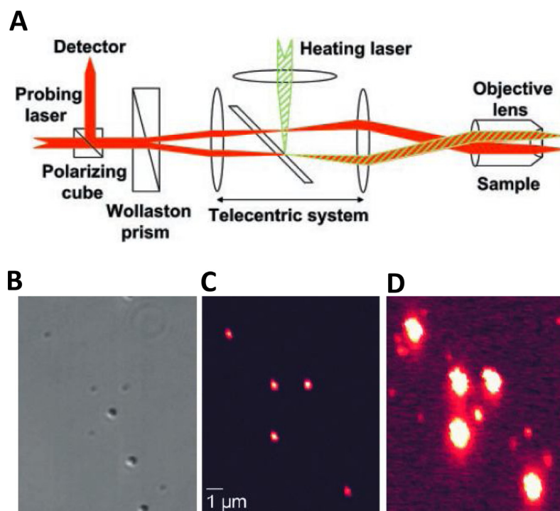
Fig. 6. (A) Optical setup of photothermal optical microscope. (B) Differential interference contrast (DIC) imaging and (C–D) photothermal images of a sample containing 300 nm latex spheres, 80 nm Au nanospheres, and 10 nm Au nanospheres. DIC image shows the 80 nm Au nanospheres and 300 nm latex spheres, while the 10 nm Au nanospheres are invisible. (C) The photothermal image with lower laser heating intensity showing the 80 nm Au nanospheres. (D) The photothermal image with higher laser heating intensity enables clear visualization of 10 nm Au nanospheres with 80 nm AuNPs reaching saturated detection. Printed with permission from American Association for the Advancement of Science [80].
