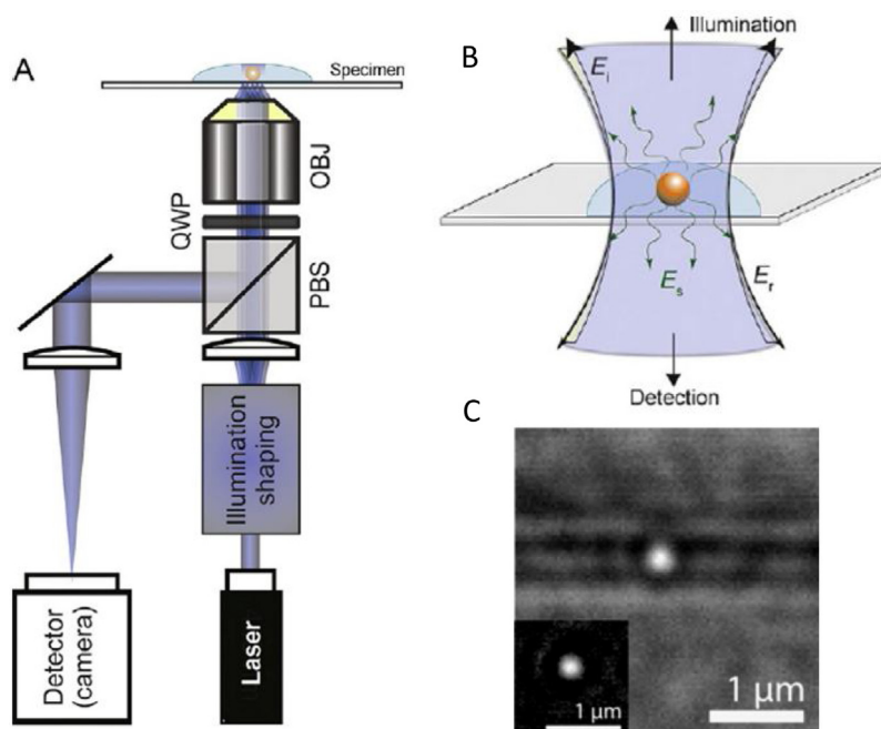
Fig. 5. (A) Optical setup for interferometric scattering (iSCAT) microscopy. OBJ: microscope objective; PBS: polarizing beam splitter; QWP: quarter-wave plate. (B) Operating principle of iSCAT. E_i is incident electric field; E_s is scattered electric field; E_r is reflected electric field. A and B are printed with permission from Elsevier [75]. (C) Raw iSCAT image of a 30 nm AuNP walking along a microtubule. (Inset) The image after background subtraction. Printed with permission from National Academy of Sciences [74].
