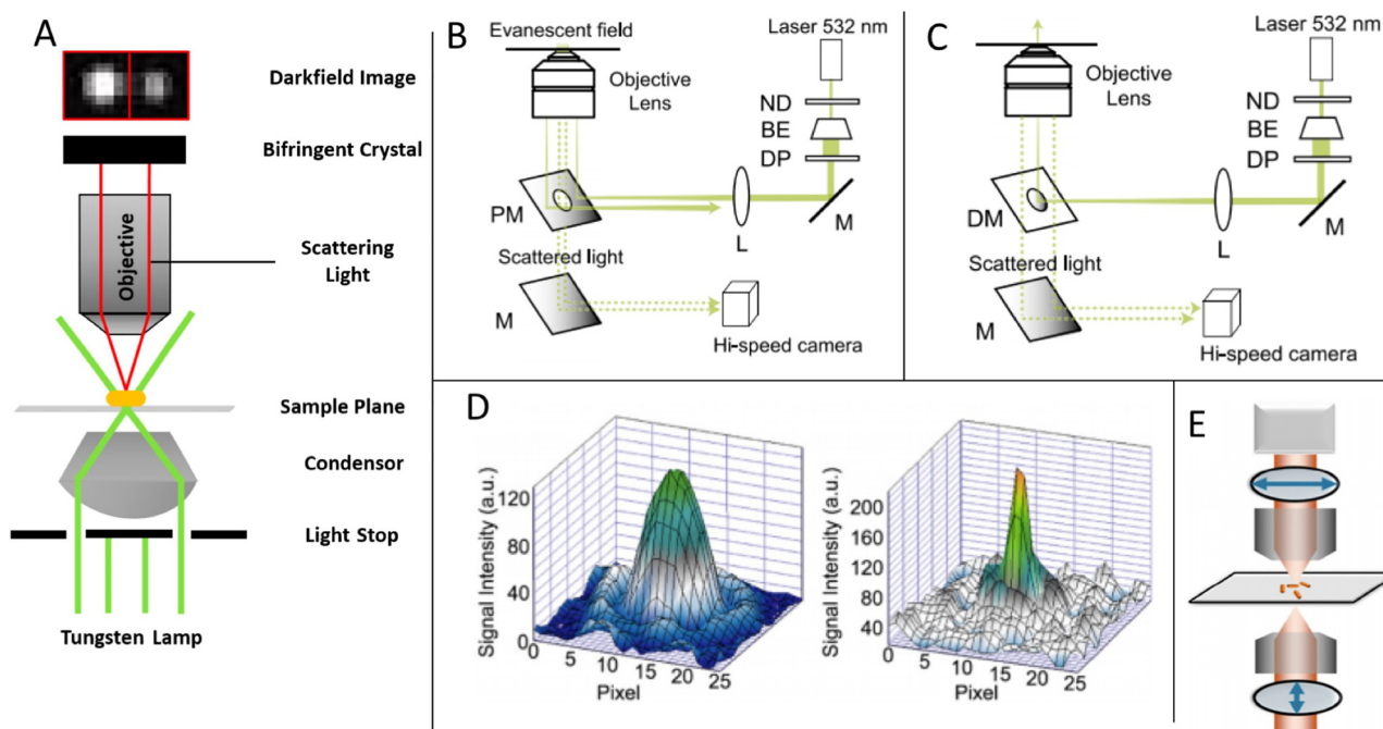
Fig. 3. (A) The working principle of dark field (DF) microscopy. Printed with permission from Iowa State University [57]. (B) Schematic illustrations of objective-type total internal reflection dark-field microscopy (TIRDFM) with a perforated mirror (PM) and (C) vertical illumination dark-field microscopy (VIDFM) with a dot mirror (DM). (ND) neutral density filter, (BE) laser beam expander, (DP) diaphragm, (M) mirror, (L) lens. (D) Intensity profiles of 40-nm gold nanoparticles by TIRDFM (left) and VIDFM (right). Pixel size = 88.5 nm. The profile was fitted by 2D-Gaussian. FWHM of PSF were 672 \pm 36 and 623 \pm 41 nm ( n = 15 ), and 259 \pm 48 and 212 \pm 34 nm ( n = 15 ) in the x- and y directions, for TIRDFM and VIDFM, respectively. Values are means \pm SD. B–D are printed with permission from Elsevier [54]. (E) Setup for orientation-dependent localization microscopy (ODLM) for background free 3D imaging. Printed with permission from Springer Nature [56].
