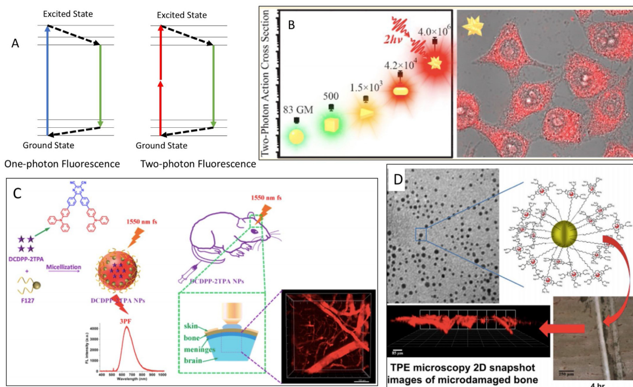
Fig. 12. (A) Two-photon imaging (TPI) working principle. (B) Difference enhancements from varied sizes of AuNPs. The right side contains gold nanostars for TPI in HepG2 cancer. Printed with permission from American Chemical Society [168]. (C) Aggregation-induced emission luminogen with a large three-photon absorption cross section in vivo . The DCDPP-2TPA NPs were synthesized with F127 as the encapsulation matrix which absorb 1550 nm excitation light and have three-photon fluorescence beneath the skull of a mouse. Printed with permission from American Chemical Society [171]. (D) Eu(III)-complexes surface-modified AuNPs as contrast agents for 3D imaging of microdamaged bones with two-photon fluorescence imaging, after being immersed for 4 h in AuNPs. Printed with permission from Elsevier [173].
