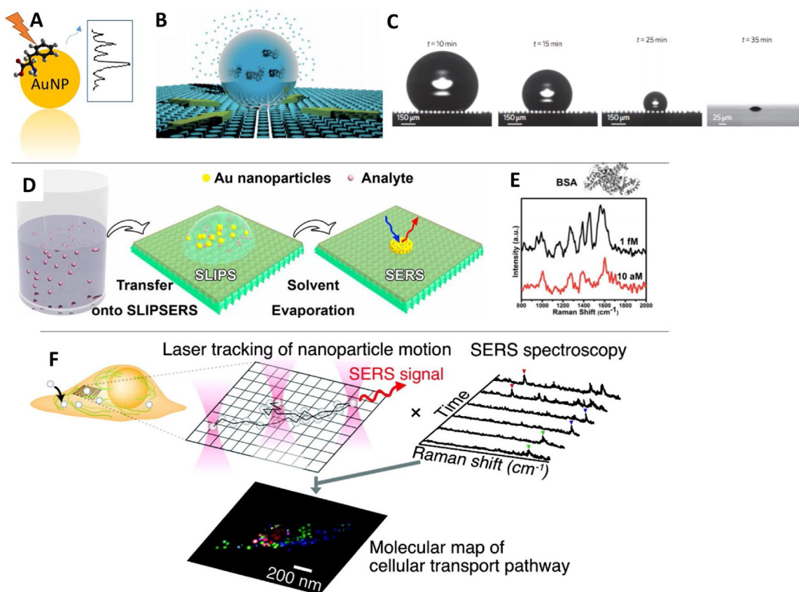
Fig. 8. (A) Principle of surface-enhanced Raman scattering (SERS). (B) Sing-molecule detection by super-hydrophobic surface (periodical silicon micropillar arrays with plasmonic nanostructures on the top of the pillars). (C) The optical images of the analyte drop on the micropillar arrays evaporating at four different times. The B and C are Printed with permission from Springer Nature [109]. (D) Single-molecule detection platform named slippery liquid infused porous surface-enhanced Raman scattering (SLIPSERS). (E) Ultra-sensitive detection of BSA protein using the platform of D. D and E are printed with permission from National Academy of Sciences [110]. (F) SERS spectra changes during AuNP endocytosis. Printed with permission from American Chemical Society [113].
