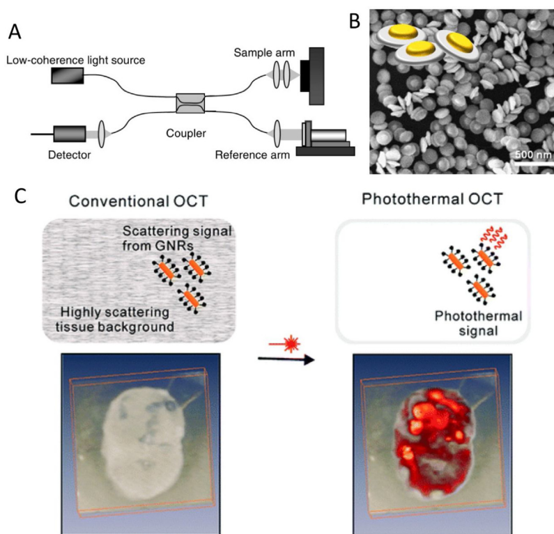
Fig. 13. (A) Optical coherence tomography (OCT) imaging working principle. Printed with permission from Springer Nature [174]. (B) Nanodisk for enhancing OCT. Printed with permission from American Chemical Society [178]. (C) OCT gets higher signal enhancement in sentinel lymph nodes (SLN) when using the Photothermal effect of AuNRs. Printed with permission from American Chemical Society [181].
