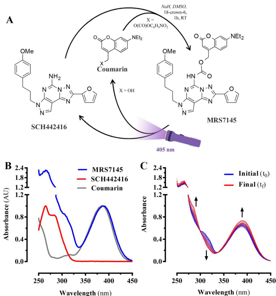
Fig. 1. Design, synthesis and photochemical properties of MRS7145. (A) The synthesis of MRS7145 involves a procedure using SCH442416 and 7-diethylamino-4-hydroxymethylcoumarin (coumarin). In brief, 60% NaH was first added to a solution of SCH442416 and 18-crown-6. After 15 min, a solution of the coumarin nitrophenyl carbonate was added. After 1 h, DMF was co-evaporated onto SiO 2 with toluene (3 ×) and chromatographed with 20 to 100% EtOAc/hexanes (see Materials and methods ). Upon irradiation with 405 nm visible light the irreversible photolytic reaction produced SCH442416. (B) Absorption spectra of 7-diethylamino-4-hydroxymethylcoumarin, SCH442416 and MRS7145 in PBS:DMSO 1:1 and 37 °C. (C) Time-course of spectral changes registered for MRS7145 in PBS:DMSO 1:1 upon irradiation at 405 nm and 37 °C during 30 min, which are consistent with the light-induced uncaging of SCH442416.
