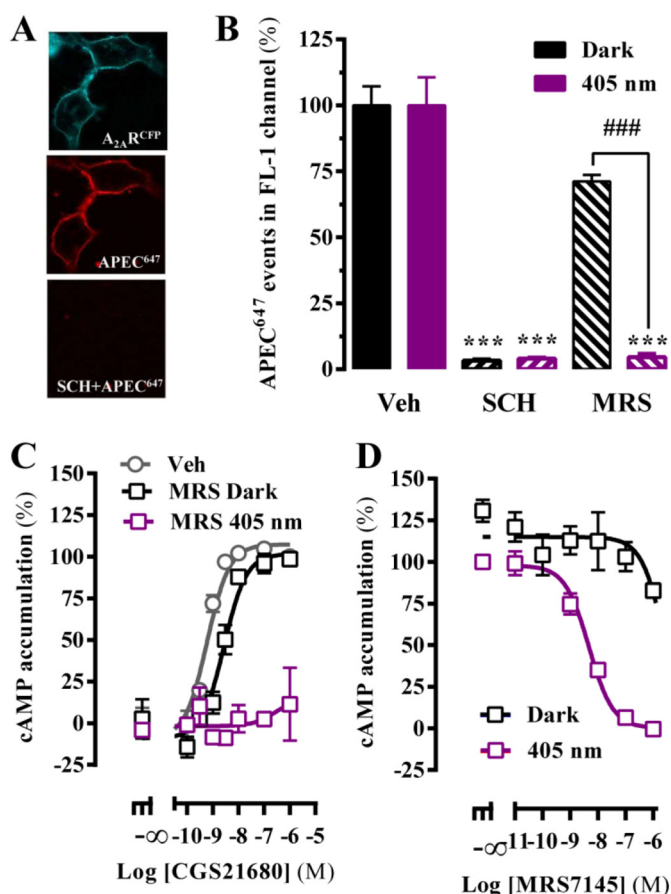
Fig. 2. MRS7145-dependent photo-control of exogenously and endogenously expressed adenosine A_{2A} receptor in cultured cells. (A) HEK-293 cells stably transfected with the human CFP-tagged adenosine A_{2A} receptor ( A_{2A}R^{CFP} ) were perfused with APEC 647 (MRS5842) (1 \mu M) in the absence and presence of SCH442416 (1 \mu M). (B) The binding properties of MRS7145 were measured by a flow cytometer throughout the incubation of APEC 647 (100 nM) in A_{2A}R -CFP cells in the presence of SCH442416 (1 \mu M) or MRS7145 (1 \mu M), all in dark conditions and upon irradiation at 405 nm. Data was expressed as a percentage of the specific events within the fluorescent region of analysis (Supplementary Fig. 5). The percentage of binding was calculated as described in Materials and Methods and expressed as mean \pm SEM ( n = 4 ). * P < 0.05 , ** P < 0.01 , *** P < 0.001 , **** P < 0.0001 , one-way ANOVA with a Tukey's multiple comparison test using the Veh + dark condition as a control. # P < 0.05 , ## P < 0.01 , ### P < 0.001 , #### P < 0.0001 , Student's t -test when comparing dark vs 405 nm conditions. Similar results were obtained in three independent experiments. (C) Determination of A_{2A}R -mediated cAMP accumulation in A_{2A}R -CFP cells. Normalized dose-response of CGS21680-induced cAMP accumulation in the absence (grey circles) or presence of MRS7145 in dark conditions (black squares) and upon irradiation at 405 nm (violet squares) are shown. (D) cAMP accumulation in A_{2A}R -CFP cells stimulated with CGS21680 (10 nM) in the absence or presence of increasing concentrations of MRS7145, both in dark conditions (black squares) and upon irradiation at 405 nm (violet squares). The percentage of cAMP accumulation was calculated as described in Materials and Methods and expressed as mean \pm SEM ( n = 3 ). Similar results were obtained in three independent experiments. (For interpretation of the references to colour in this figure legend, the reader is referred to the web version of this article.)
