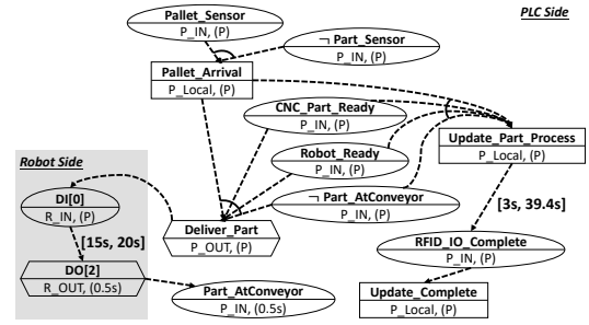
Fig. 5: The TECG of the Motivating Example
