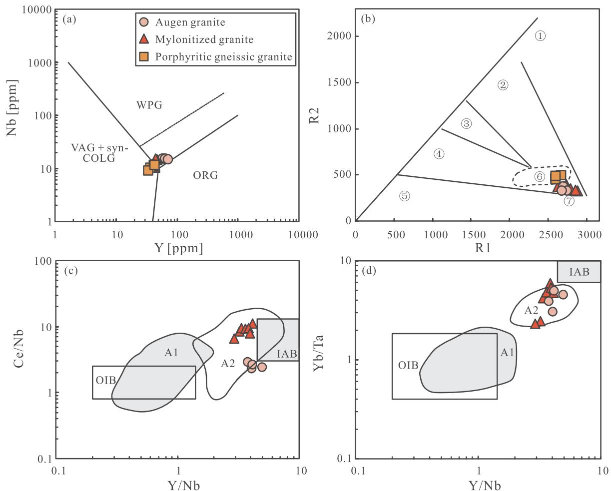
Fig. 13. Trace- and major-element discrimination diagrams for the tectonic setting of the studied granites. (a) Nb–Y (Pearce et al., 1984); (b) R1–R2 diagram of Batchelor and Bowden (1985): (1) mantle fractionates, (2) pre-plate collision, (3) post-collision, (4) late orogenic, (5) anorogenic, (6) syn-collision, and (7) post-orogenic; (c, d) Chemical subdivision of A-type granites (Eby, 1992), (A1) truly anorogenic rifting; (A2) post-collisional.
