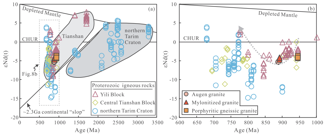
Fig. 8. \epsilon\text{Nd}(t) –Age plots for zircons from Precambrian igneous rocks of this study, from the Yili Block, Central Tianshan Block, and northern Tarim Craton (data from this study; Wang et al. (1991, 2014b,c, 2017); Chen et al. (1999, 2017); Hu et al. (2000, 2010); Zhang et al. (2007b, 2009, 2011, 2012c); Cao et al. (2011); Lei et al. (2013); Ye et al. (2013, 2016); Wu et al. (2014); Cai et al. (2018)).
