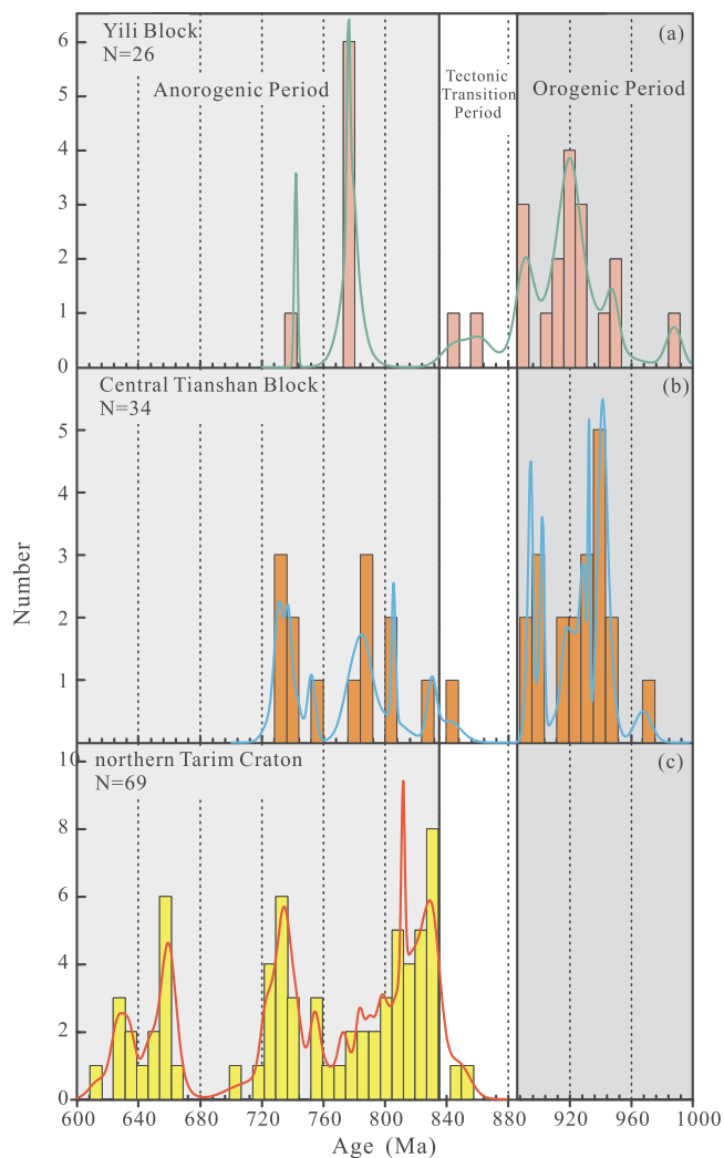
Fig. 14. Zircon U–Pb age frequency distributions for Neoproterozoic igneous rocks of the Yili Block, Central Tianshan Block, and Tarim Craton (data sources: Supplementary Table S5).
