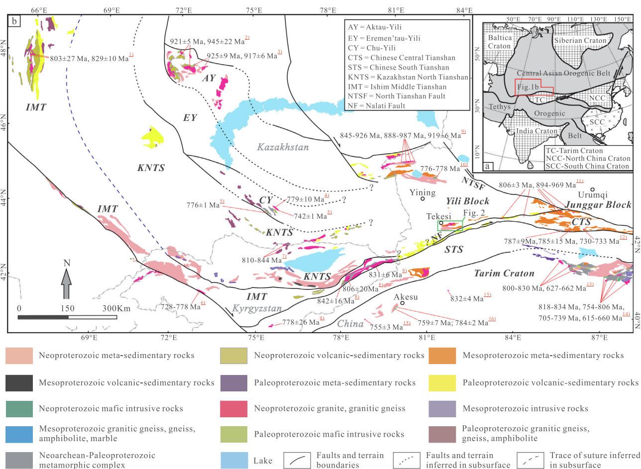
Fig. 1. (a) Simplified tectonic divisions of eastern Eurasia, showing the location of the Central Asian Orogenic Belt (CAOB) (modified after Kröner et al. (2007)); (b) Generalized tectonic framework of the southwestern CAOB and major surrounding units (simplified after Levashova et al. (2011)). Data sources: (1) Tretyakov et al. (2011, 2017); (2) Tretyakov et al. (2015); (3) Degtyarev et al. (2008); (4) Pilitsyna et al. (2019); (5) Kröner et al. (2007); (6) Konopelko et al. (2013); (7) Kröner et al. (2012); (8) Glorie et al. (2011); (9) Hu et al. (2010), Wang et al. (2014a), Huang (2017); (10) Wang et al. (2014b); (11) Yang et al. (2008), Long et al. (2011), Gao et al. (2015), Huang et al. (2015b); (12) Wang et al. (2014c, 2017), Gao et al. (2015); (13) Ge et al. (2012, 2013), Zhang et al. (2013 and references therein); (14) Chen et al. (2017), Han et al. (2018 and references therein); (15) Xu et al. (2013); (16) Zhang et al. (2009, 2012a).
