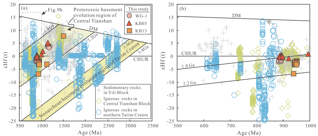
Fig. 9. \epsilon\text{Hf}(t) –Age plots for zircons from Precambrian rocks of the Yili Block, the Central Tianshan Block, and the northern Tarim Craton (data from this study; He et al. (2013, 2015a,b, 2018a); Lei et al. (2013); Ye et al. (2013, 2016); Zong et al. (2013); Ge et al. (2014a, b); Huang et al. (2014, 2015a,b, 2016, 2017); Wang et al. (2014c,d, 2017); Wu et al. (2014, 2018); Gao et al. (2015); Kovach et al. (2016); Chen et al. (2017); Cai et al. (2018)).
