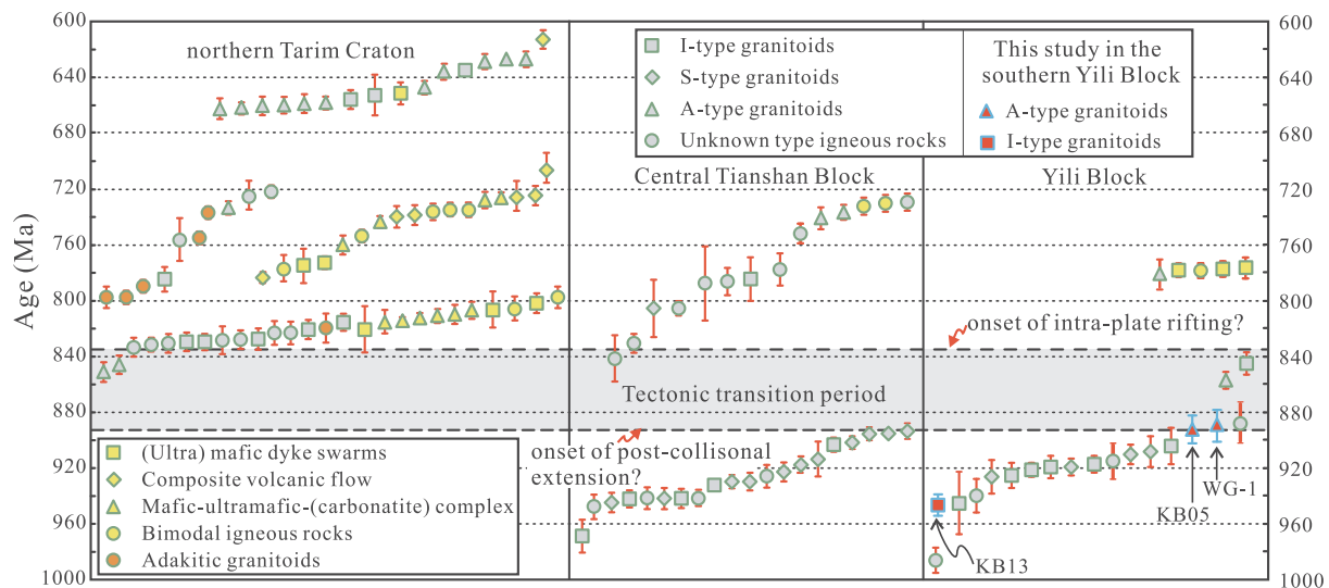
Fig. 15. Diagram illustrating the distribution of the Neoproterozoic magmatism in different genetic types from the Yili Block, Central Tianshan Block, and northern Tarim Craton (Data sources: Supplementary Table S5 ).
