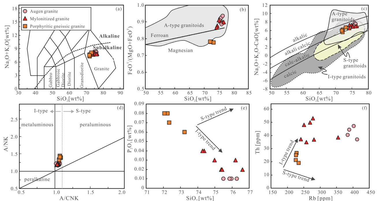
Fig. 6. Variation diagrams for the studied granites of the southern Yili Block. (a) Total-alkali–silica (TAS) classification (Middlemost, 1994); (b) \text{FeO}^T/(\text{FeO}^T + \text{MgO}) – \text{SiO}_2 (Frost et al., 2001); (c) (\text{Na}_2\text{O} + \text{K}_2\text{O} - \text{CaO}) – \text{SiO}_2 (Frost et al., 2001); (d) A/NK–A/CNK (Maniar and Piccoli, 1989); (e) \text{P}_2\text{O}_5 – \text{SiO}_2 ; and (f) Th–Rb (Chappell and White, 1992).
