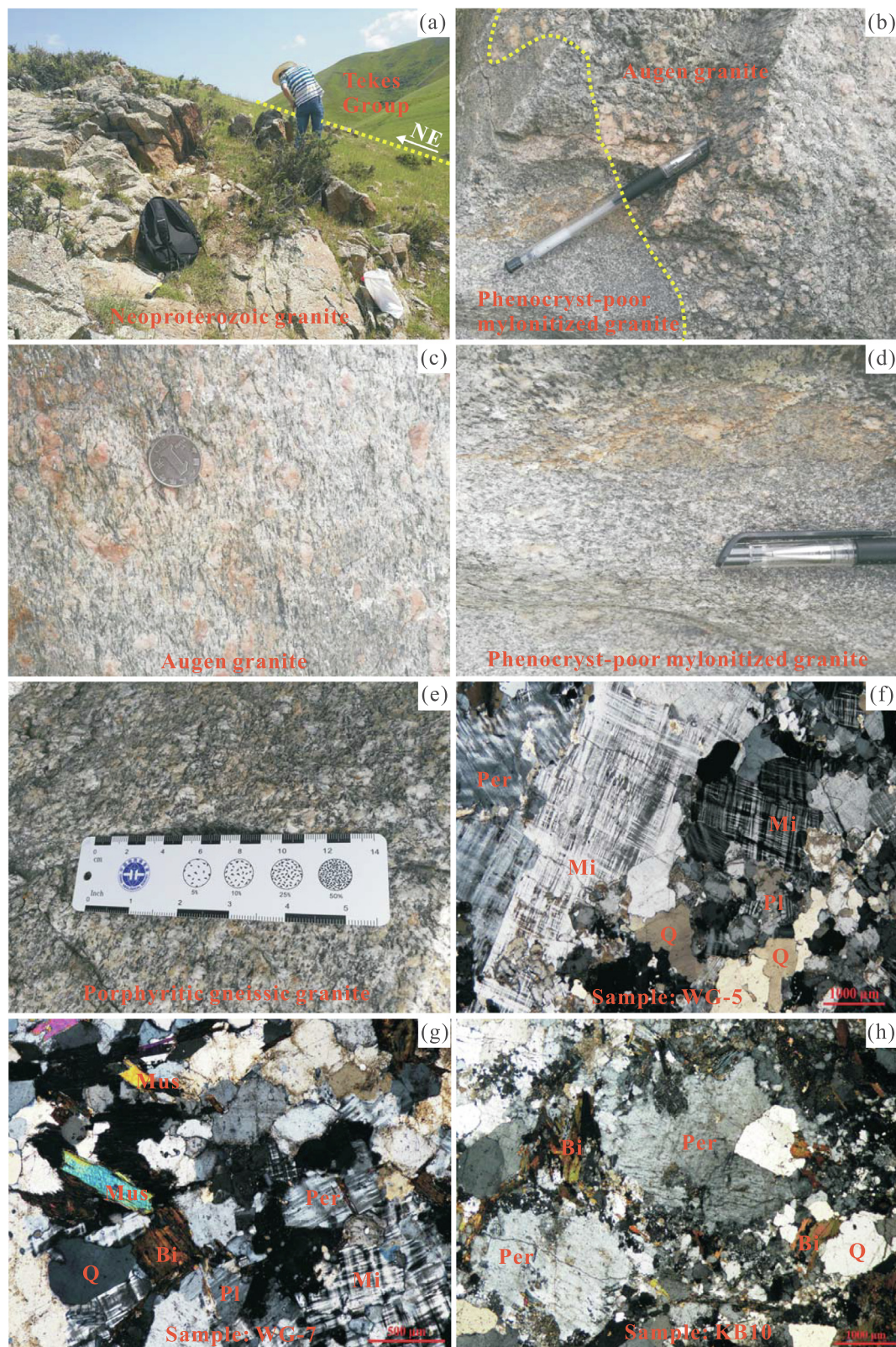
Fig. 3. Field and petrographic photographs of the studied Neoproterozoic granites in the southern Yili Block. (a) Neoproterozoic mylonitized granite; (b) Augen and mylonitized granites; (c) Augen granite; (d) Mylonitized granite; (e) Porphyritic gneissic granite; (f) Augen granite (sample WG-5); (g) Mylonitized granite (sample WG-7); (h) Porphyritic gneissic granite (sample KB10). (Per = Perthite; Mi = Microcline; Pl = Plagioclase; Bi = Biotite; Qz = Quartz; Mus = Muscovite).
