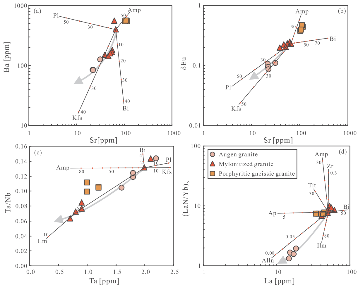
Fig. 12. Diagrams of fractional crystallization simulation (Ersoy and Helvacı, 2010). (a) Ba–Sr; (b) \delta\text{Eu} –Sr; (c) Ta/Nb–Ta; (d) (\text{La}/\text{Yb})_N –La. Pl = plagioclase; Kfs = K-feldspar; B = biotite; Amp = amphibole; Ap = apatite; Alln = allanite; Ilm = ilmenite; Tit = titanite; Zr = zircon.
