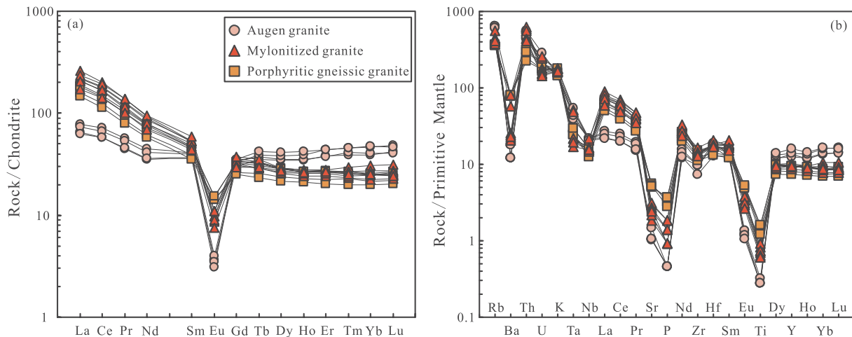
Fig. 7. Chondrite-normalized REE patterns and primitive mantle-normalized trace-element spider diagrams for the studied granites of the southern Yili Block. Normalizing values of chondrite and of primitive mantle are from Taylor and McLennan (1985) and Sun and McDonough (1989), respectively.
