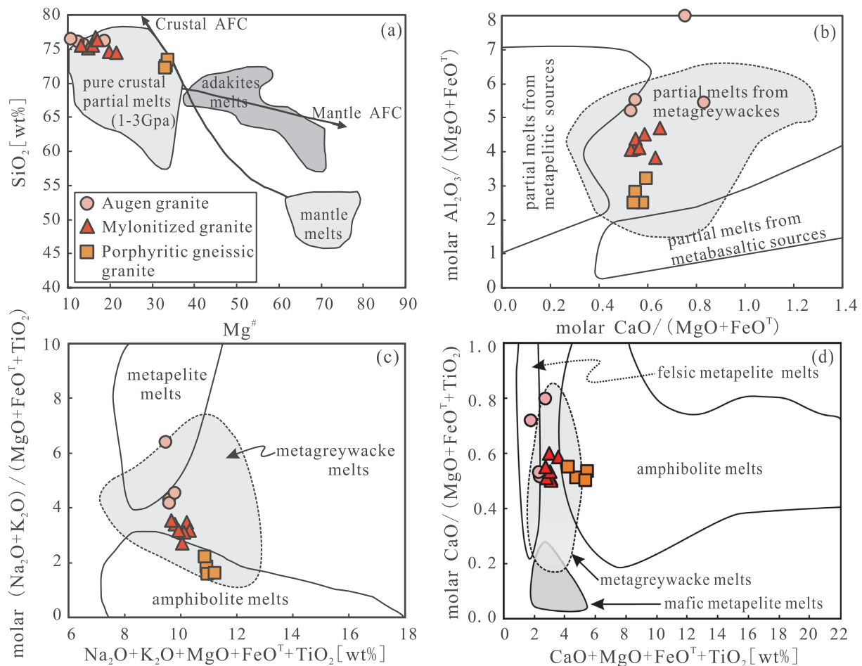
Fig. 11. Chemical compositions of the studied granites of the southern Yili Block. Outlined fields denote compositions of partial melts obtained in experimental studies by dehydration melting of various bulk compositions. The curves of mantle AFC and crustal AFC are after Stern and Kilian (1996). (Data sources: Vielzeuf and Holloway, 1988; Patiño Douce and Johnston, 1991; Rapp and Watson, 1995; Patiño Douce and Beard, 1996).
