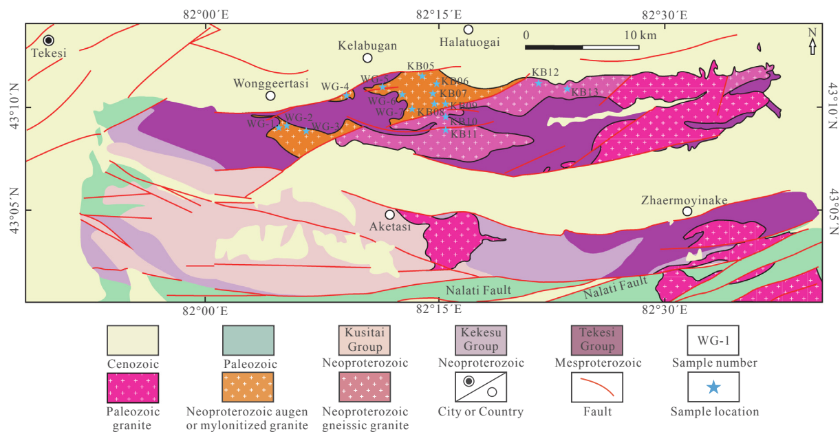
Fig. 2. Simplified geological map with sampling locations of the studied Neoproterozoic granites in the southern Yili Block (modified after XBGMR, 1978).
