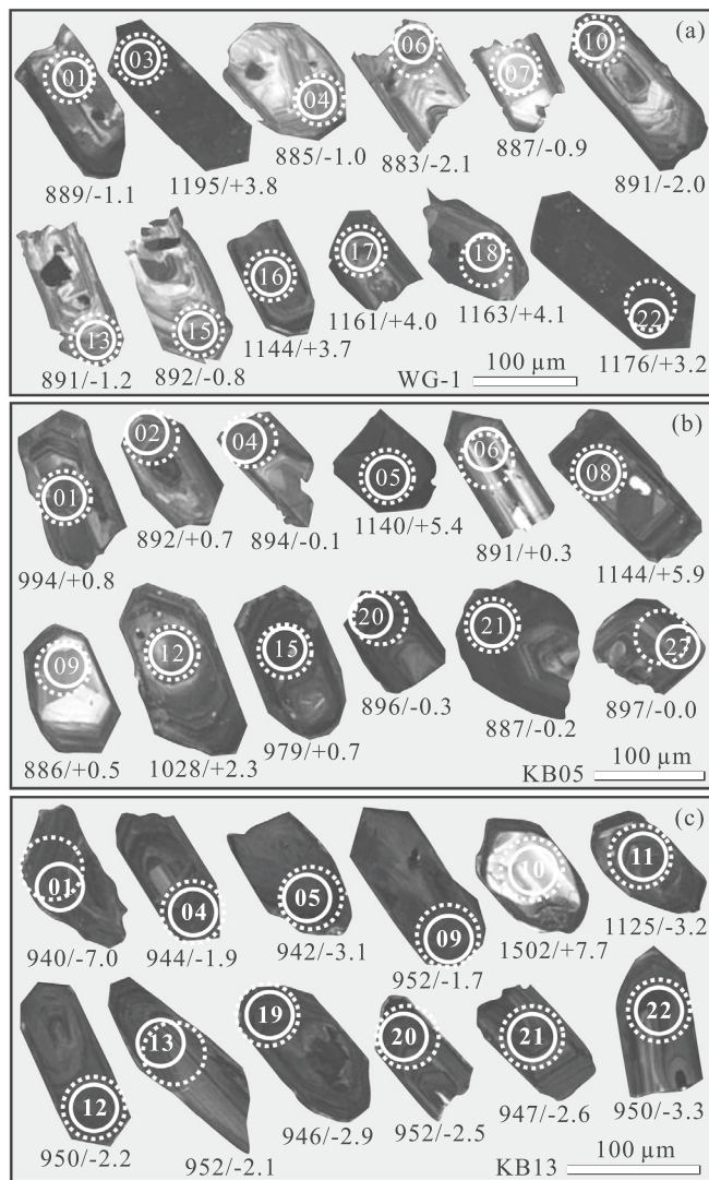
Fig. 4. Representative CL images of zircons from the studied granites in the southern Yili Block. (a) Sample WG-1 from augen granite; (b) KB05 from mylonitized granite; (c) KB13 from gneissic granite. (Solid and dashed circles represent points analysed for U–Pb and Lu–Hf isotopes, respectively).
