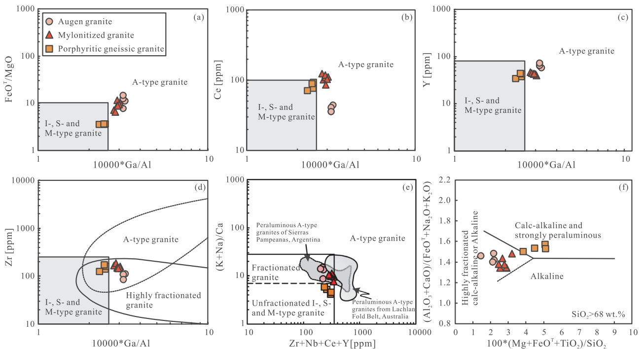
Fig. 10. (a–e) Chemical classification diagrams (after Whalen et al., 1987) in which the augen and mylonitized granites plot in the field of highly fractionated A-type granites; (f) Major-element classification diagram (after Sylvester, 1989) showing the fields of alkaline, calc-alkaline, and highly fractionated calc-alkaline rocks. The fields of A-type and highly fractionated granites in (d) are from Wu et al. (2017); the fields of peraluminous A-type granites are from the following sources: Sierras Pampeanas (Morales Cámara et al., 2017); Lachlan Fold Belt (Whalen et al., 1987).
