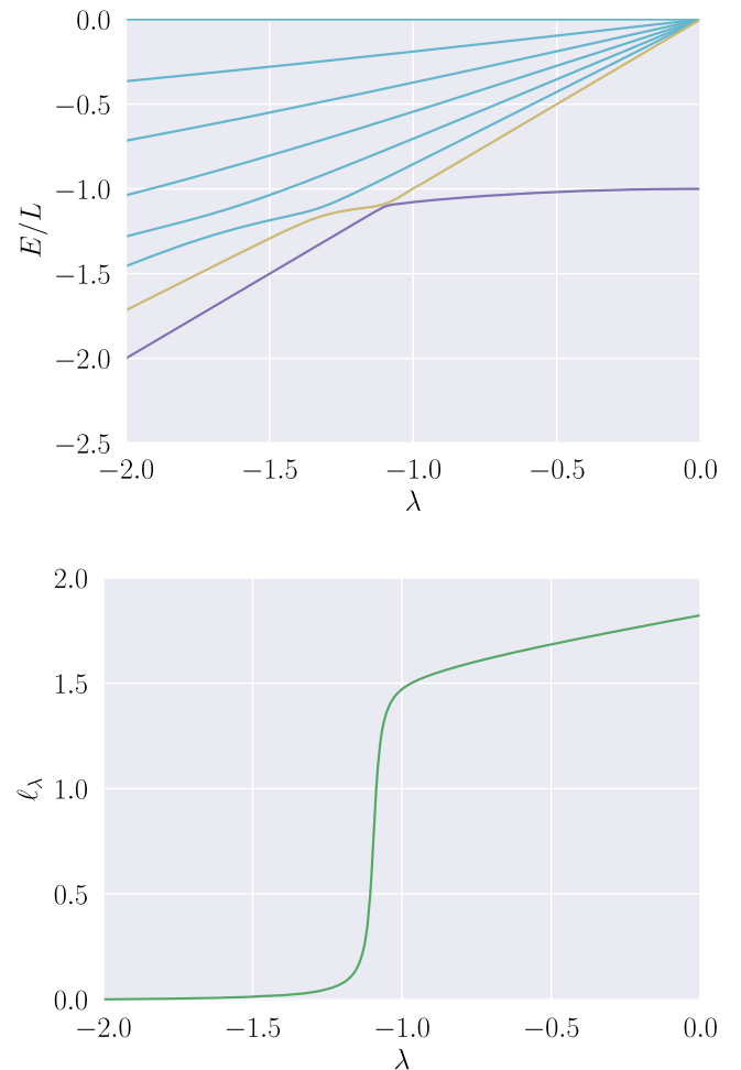
FIG. 6. Low-energy spectrum of a 14-spin disorder-free p -spin model for p = 51 described by Hamiltonian (34). The model has a first-order transition with an exponentially small gap separating the two phases. In the thermodynamic limit, the geodesic length \ell_\lambda jumps by \pi/2 at the critical point.
