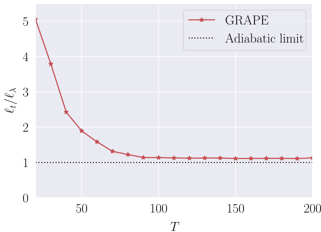
FIG. 7. Numerical verification of the geometric bound conjecture (2) for the ground state of a disorder-free p -spin model described by Hamiltonian (34).
