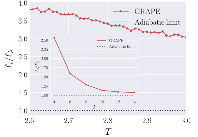
FIG. 2. Numerical justification of the conjecture [cf. Eq. (2)] across the quantum speed limit of preparing the interacting ground state of the Hamiltonian H_{3\text{LS}} following evolution generated by H_{3\text{LS}}(t) . The inset shows numerical evidence that the conjecture is saturated in the adiabatic limit. The parameters are \lambda_i/g = -2 = -\lambda_*/g . The optimal control algorithm used is GRAPE [45,53].
