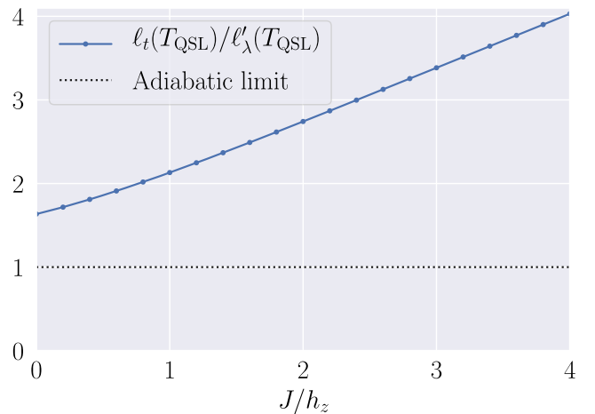
FIG. 1. Numerical justification of the conjecture (2), at the quantum speed limit of preparing the interacting ground state of H_{\text{3LS}} with the noninteracting fast-forward Hamiltonian H_{\text{2LS}}(t) . The parameters are \lambda_i/g = -2 = -\lambda_*/g .
