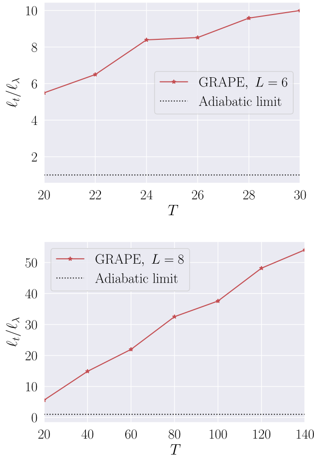
FIG. 5. Numerical verification of the geometric bound conjecture (2) for the excited states of the Hamiltonian (33).
