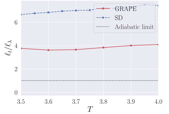
FIG. 3. Numerical justification of the conjecture [cf. Eq. (2)] in the high-fidelity region of the quantum state preparation problem in the many-body Hamiltonian (32) as a function of the protocol duration T . The parameters are \lambda_i/g = -2 = -\lambda_*/g , J/g = 1 , and L = 10 . We use SD to find (nearly) optimal bang-bang protocols \lambda(t) \in \{\pm 4\} of time step \delta t = 0.005J .
