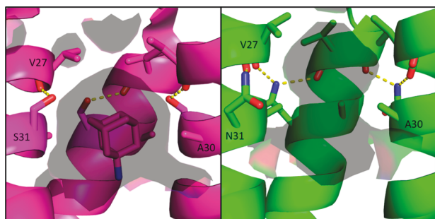
Figure 8. Solvent-accessible surface area inside the M2 pore at the adamantane binding site. Amantadine-bound WT structure in the Inward closed conformation 6BKK (left, magenta) vs S31N Inward closed conformation (green, right); solvent-accessible surface area (calculated using a 1.4 Å probe) is shown as a transparent surface. In the WT channel, Ser31 forms an intrahelix hydrogen bond and partially faces the pore. In the S31N mutant, Asn31 faces the monomer-monomer interface, twisting the monomer helices such that Ala30 faces the center of the pore. This constricts and elongates the pore at the amantadine binding site for the S31N mutant M2 channel.
