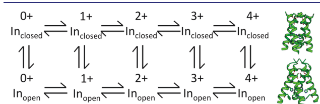
Figure 1. Simultaneous equilibria between the His37 tetrad charge states and the two conformational states, \text{Inward}_{\text{closed}} and \text{Inward}_{\text{open}} .
