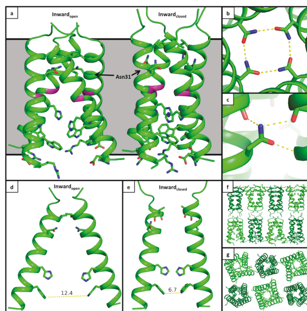
Figure 2. X-ray crystal structure of M2(22–46) S31N in two conformational states. (a) The \text{Inward}_{\text{open}} conformation is at left, and the \text{Inward}_{\text{closed}} conformation is at right (PDB: 6MJH). The monomer helices in the \text{Inward}_{\text{open}} conformation are straight, and in the \text{Inward}_{\text{closed}} conformation they are kinked at Gly34 (shown in purple). As previously observed in structure 5C02, Asn31 faces the center of the pore and forms H-bonds with Asn31 side chains from neighboring monomers in the \text{Inward}_{\text{open}} conformation. In the \text{Inward}_{\text{closed}} conformation, Asn31 faces away from the pore and forms H-bonds with carbonyls at the monomer–monomer interface. (b) Top-down view showing hydrogen-bonding networks formed by Asn31 in the \text{Inward}_{\text{open}} conformation. (c) Side view of the hydrogen-bonding network formed by Asn31 in the \text{Inward}_{\text{closed}} conformation. (d) Side view of the \text{Inward}_{\text{open}} conformation, only chains F and H shown. (e) Side view of the \text{Inward}_{\text{closed}} conformation, only chains A and C shown. (f) Side view of crystal lattice from structure 6MJH, with the \text{Inward}_{\text{open}} conformation in light green and the \text{Inward}_{\text{closed}} conformation in dark green. (g) Top-down view of crystal lattice.
