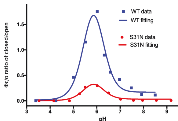
Figure 7. Fitting of experimental data as a function of pH, giving R square values 0.96 and 0.95 for WT and S31N, respectively, and producing the three pK_a 's for the Inward closed state ( pK_1: 6.4 \pm 1.1 , pK_2: 7.4 \pm 1.2 and pK_3: 4.4 \pm 0.8 ) and one pK_a ( 5.9 \pm 0.1 ) for the Inward open state. We set the pK_4 as a constant 3, but the fit was insensitive to its value, so long as it was set less than 4.0.
