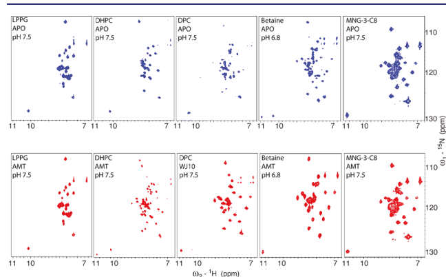
Figure 3. Conformational equilibrium between the Inward open and Inward closed conformations for M2(19–49) WT is dependent on detergent choice in 2D NMR experiments. Solution NMR spectra of M2(19–49) WT in multiple detergents, without inhibitors (blue, top), and with inhibitors (red, bottom). The Trp41 indole proton peak (bottom left corner of each spectrum) can be used to distinguish the conformational states; a peak with chemical shift of ~11.0 ppm corresponds to the Inward closed conformation, and a peak with chemical shift of ~10.2 ppm corresponds to the Inward open conformation. From left to right: In LPPG, M2 stays in the Inward open conformation in absence and in the presence of amantadine. In DHPC, the presence of amantadine shifts a small portion of the protein in the Inward open conformation to the Inward closed conformation. In DPC, the inhibitor WJ10 almost fully shifts the Inward open to the Inward closed conformation. In C 14 -betaine, both conformations are observed in the absence of any drugs, and addition of amantadine fully shifts the protein to the Inward closed conformation. In MNG-3-C8, the protein stays in the Inward closed conformation in absence or presence of amantadine.
