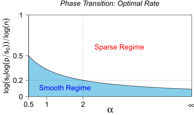
Figure 1. The minimax lower bound is n^{-2\alpha/(2\alpha+1)} when \alpha, p, s_0 and n fall into smooth regime. Otherwise, the minimax lower bound is s_0 \log(p/s_0)/n in the sparse regime.
