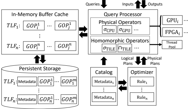
Figure 9: LightDB architecture
