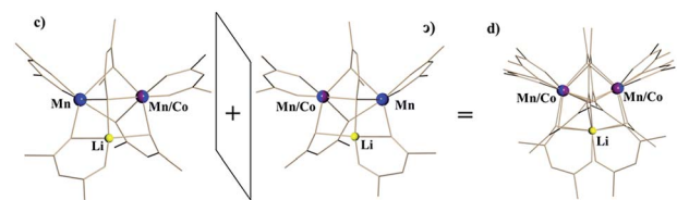
Fig. 5 Disordered unit (d) in the crystal structure of \text{LiMn}_{1.5}\text{Co}_{0.5}(\text{thd})_5 ( 1b ) as a superposition of two enantiomers ( S , A , A -c and R , A , A -c).
