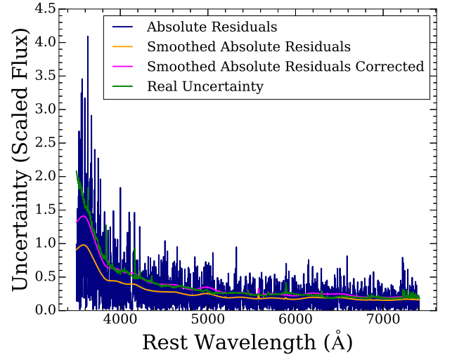
Figure 12. Uncertainty spectra corresponding to the spectrum of SN 2005lz presented in Fig. 11. The blue curve is the absolute residual spectrum from the difference between the clipped spectrum and the smoothed spectrum, the green curve is the real uncertainty spectrum from the CfA archive, the yellow curve is the smoothed absolute residual spectrum, and the pink curve is the same spectrum after applying a small scaling in order to better match the green curve.
