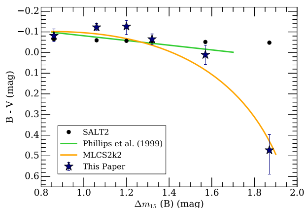
Figure 22. The relationship between \Delta m_{15}(B) and B - V colour at maximum light. The blue stars are measurement made from our composite spectra in Fig. 21. The black circles are measurements made from maximum-light SALT2 template spectra with effective \Delta m_{15}(B) corresponding to the mean values of \Delta m_{15}(B) from our composite spectra. The green and orange curves are fits from Phillips et al. (1999) and Phillips (1993), respectively.
