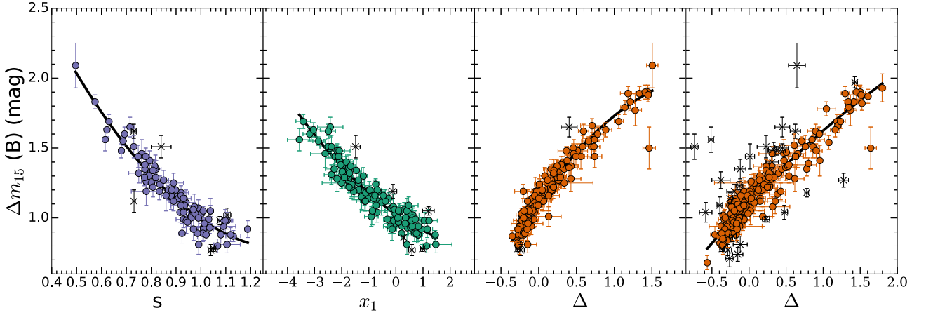
Figure 10. Power-law relationships between \Delta m_{15}(B) and the light-curve shape parameters s (SALT; first), x_1 (SALT2; second), \Delta (MLCS using R_V = 3.1 ; third), and \Delta (MLCS using R_V = 2.5 ; fourth). We use these relationships to determine an estimate of \Delta m_{15}(B) when there is no explicit measurement available. In all panels, points marked with a black 'x' are 3\sigma outliers and are not included when fitting the relation.
