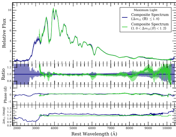
Figure 27. Same format as Fig. 15 except we compare our maximum-light composite spectrum (blue curve) from Fig. 26 and our maximum-light composite spectrum with 1.0 < \Delta m_{15}(B) < 1.2 mag (green curve).
