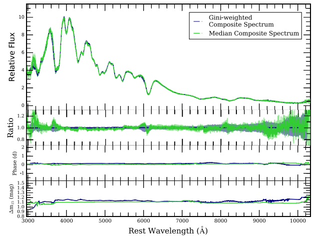
Figure 16. A comparison between Gini-weighted composite spectra and median composite spectra constructed from the subsample of 96 SNe Ia with -1 < \tau < +1 d and \Delta m_{15}(B) < 1.8 mag (blue and green curves, respectively). The panel format is the same as Fig. 15.
