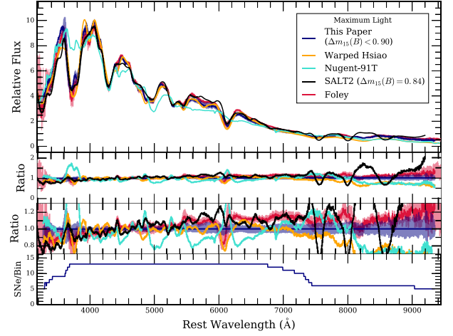
Figure 31. Same as Fig. 26 except the composite spectrum (blue curve) is constructed using a phase bin of -1 < \tau < +1 d and a \Delta m_{15}(B) bin of \Delta m_{15}(B) < 0.90 mag. The maximum-light Hsiao template spectrum has been warped to match the B -, V -, and R -band photometry measured from the composite spectrum. The red curve is the Foley maximum-light, \Delta = -0.27 template spectrum. The light-blue is the Nugent-91T template spectrum, and the black curve is the maximum-light SALT2 model spectrum corrected for light-curve shape such that it has an effective \Delta m_{15}(B) = 0.84 mag.
