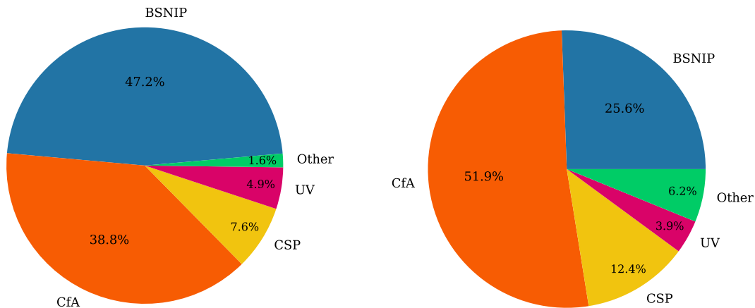
Figure 1. (left): Contributions of each major data source to the total number of SNe in the data base. (right): Contributions of each major data source to the total number of spectra in the data base. The BSNIP sample provides the largest number of individual SNe, while the CfA sample tends to provide the largest number of spectra per SN.
