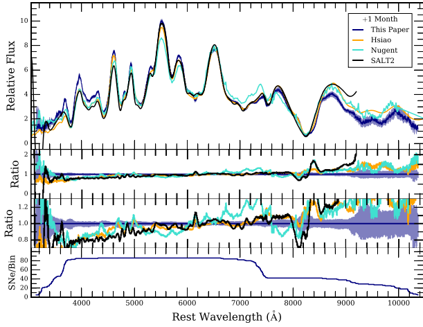
Figure 30. Same as Fig. 26 except the composite spectrum (blue curve) is constructed using a phase bin of +28 < \tau < +32 d and \Delta m_{15}(B) < 1.8 mag.
