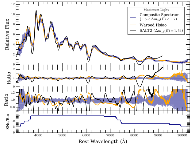
Figure 32. Same as Fig. 31 except the composite spectrum (blue curve) is constructed using a phase bin of -3 < \tau < +3 d and a \Delta m_{15}(B) bin of 1.50 < \Delta m_{15}(B) < 1.70 mag. The maximum-light SALT2 model spectrum is corrected for light-curve shape such that it has an effective \Delta m_{15}(B) = 1.64 mag.
