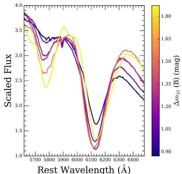
Figure 23. The Si II \lambda 5972 and \lambda 6355 absorption features of our maximum-light composite spectra from Fig. 21. The colour bar ranges from slow-declining light-curve shapes ( \Delta m_{15}(B) = 0.86 mag; dark purple) to fast-declining light-curve shapes ( \Delta m_{15}(B) = 1.87 mag; yellow).
