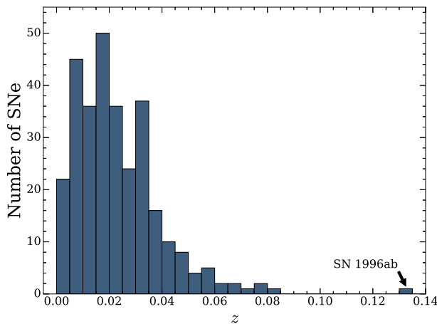
Figure 8. Histogram of the number of SNe Ia per redshift bin.
