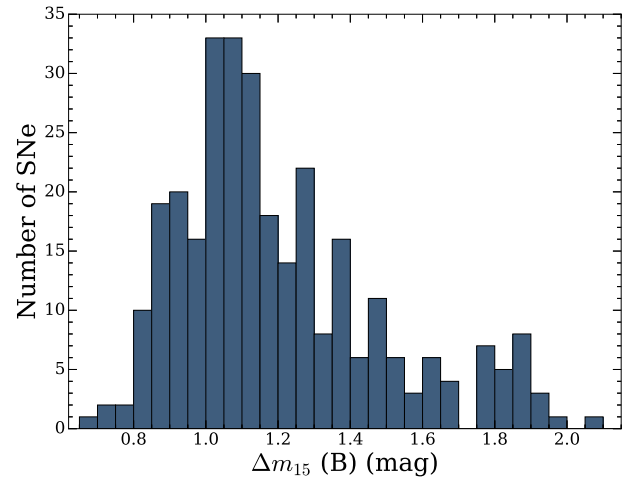
Figure 6. Histogram of the number of SNe Ia per \Delta m_{15}(B) bin. This distribution is skewed towards slower declining events and peaks at \Delta m_{15}(B) = 1.12 mag (typical for normal SNe Ia).
