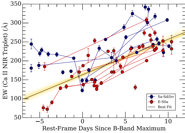
Figure 37. Ca II NIR Triplet EW evolution for SNe residing in late- (blue points) and early- (red points) type galaxies. Measurements coming from the same SNe are connected by lines. The black curve is our linear best fit to the evolution of the whole sample ( y = (9.4 \pm 0.6)x + 163 \pm 4 ). The yellow curves are best-fitting lines generated from bootstrap resampling of the data.
