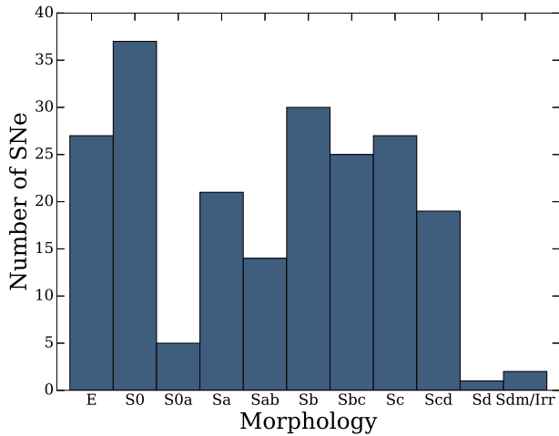
Figure 7. Histogram of the number of SNe Ia per bin in host-galaxy morphology.
