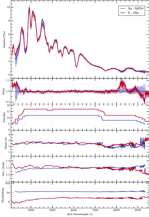
Figure 35. Same format as Fig. 14. The blue curves show the properties of our late-type composite spectrum and the red curves show the properties of our early-type composite spectrum. Both of these composite spectra were constructed using a phase bin of 0 < \tau < +6 . The late-type composite spectrum was constructed using a light-curve shape bin of 1.20 < \Delta m_{15}(B) < 1.45 mag. The early-type composite spectrum was constructed using a light-curve shape bin of 1.10 < \Delta m_{15}(B) < 1.50 mag.
