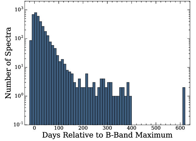
Figure 4. Histogram of the number of individual SN spectra at each epoch in the nominal sample.
