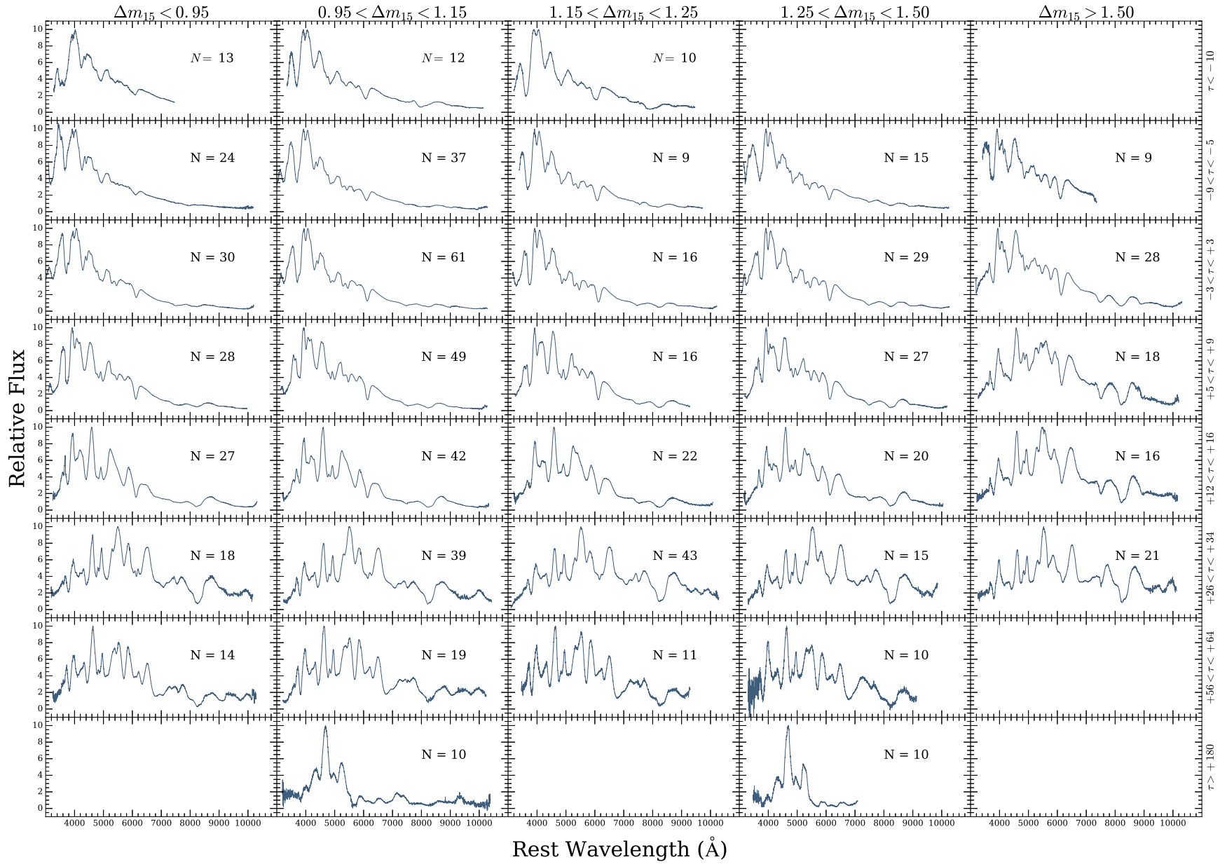
Figure 25. Phase and \Delta m_{15}(B) -binned composite spectra. Columns from left to right correspond to \Delta m_{15}(B) bins of \Delta m_{15}(B) < 0.95 mag, 0.95 < \Delta m_{15}(B) < 1.15 mag, 1.15 < \Delta m_{15}(B) < 1.25 mag, 1.25 < \Delta m_{15}(B) < 1.5 mag, and \Delta m_{15}(B) > 1.5 mag. Rows from top to bottom corresponds to phase bins of \tau < -10 d, -9 < \tau < -5 d, -3 < \tau < +3 d, +5 < \tau < +9 d, +12 < \tau < +16 d, +26 < \tau < +34 d, +56 < \tau < +64 d, and \tau > +180 d. The number of individual spectra included in each composite spectrum is stated in the corresponding panel. Composite spectra have varying wavelength ranges because we require at least five individual spectra at any given wavelength. Blank panels correspond to regions of this parameter space where we do not currently have enough data to generate a representative composite spectrum.
