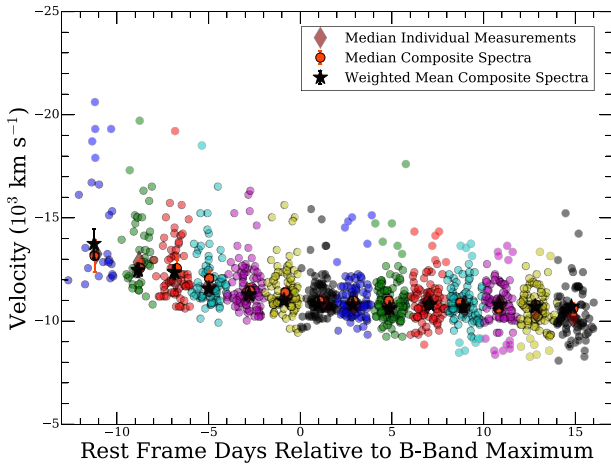
Figure 20. Velocity evolution of our composite spectra created from the nominal sample. Black stars are measurements from the weighted mean composite spectra and orange circles are measurements from median composite spectra. The smaller circle points are measurements from the individual spectra. These are colour coded to distinguish the borders of the phase bins defined for the composite spectra. The brown diamonds correspond to the median of the individual measurements within each bin.
