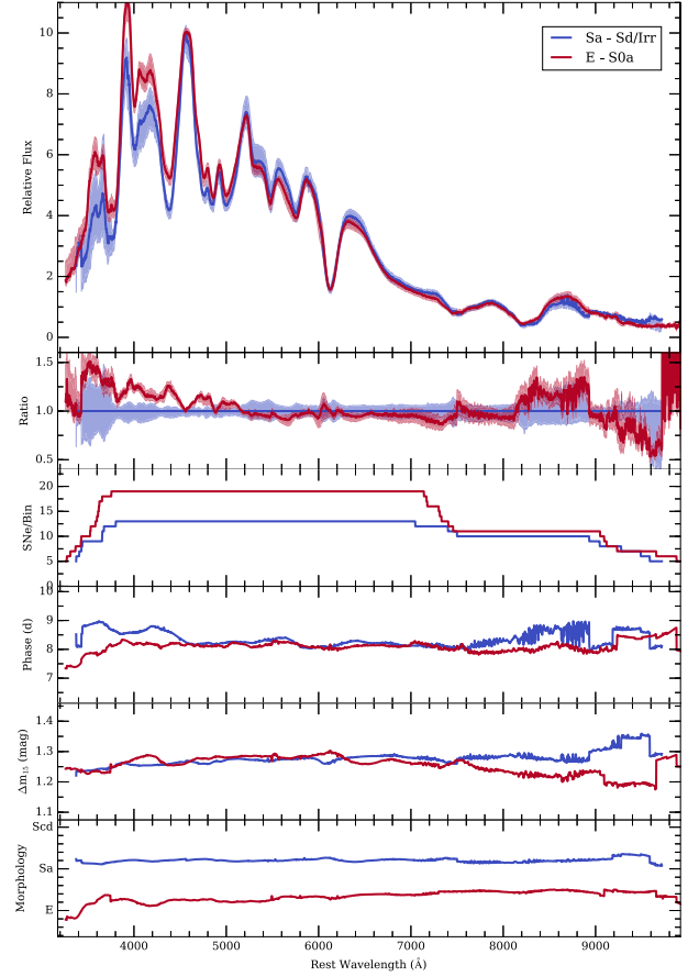
Figure 36. Same format as Fig. 14. The blue curves show the properties of our late-type composite spectrum and the red curves show the properties of our early-type composite spectrum. Both of these composite spectra were constructed using a phase bin of +6 < \tau < +11 . The late-type composite spectrum was constructed using a light-curve shape bin of 1.17 < \Delta m_{15}(B) < 1.48 mag. The early-type composite spectrum was constructed using a light-curve shape bin of 1.15 < \Delta m_{15}(B) < 1.45 mag.
