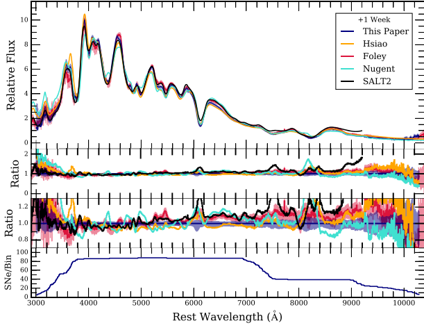
Figure 29. Same as Fig. 26 except the composite spectrum (blue curve) is constructed using a phase bin of +6 < \tau < +8 d and \Delta m_{15}(B) < 1.8 mag.
