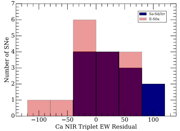
Figure 38. Histograms of the late- (blue) and early- (red) type mean Ca II NIR Triplet EW residuals per SN from Fig. 37.
