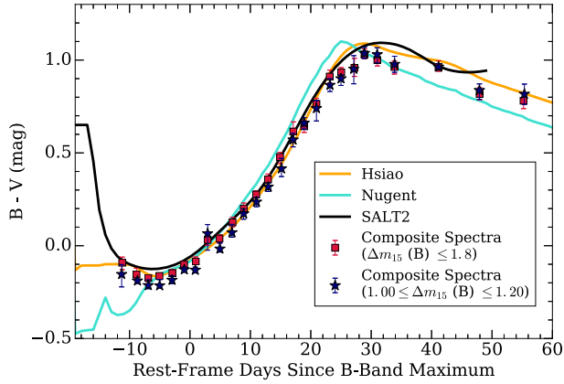
Figure 19. Comparison of the B - V colour evolution of various SN Ia template spectra and our composite spectra created from the nominal sample. The orange, light-blue, and black curves are the Hsiao, Nugent, and SALT2 template spectra, respectively. The red squares are colour measurements from composite spectra generated from the nominal sample with \Delta m_{15}(B) < 1.8 mag. The blue stars are colour measurements from composite spectra generated from the nominal sample using only SNe where 1.00 \leq \Delta m_{15}(B) \leq 1.20 mag. Bin sizes of 2 d are used for phase \leq +30 d and bin sizes of 4 d are used for phase > +30 d.
