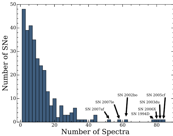
Figure 3. Histogram of the number of individual spectra per SN in the nominal sample.
