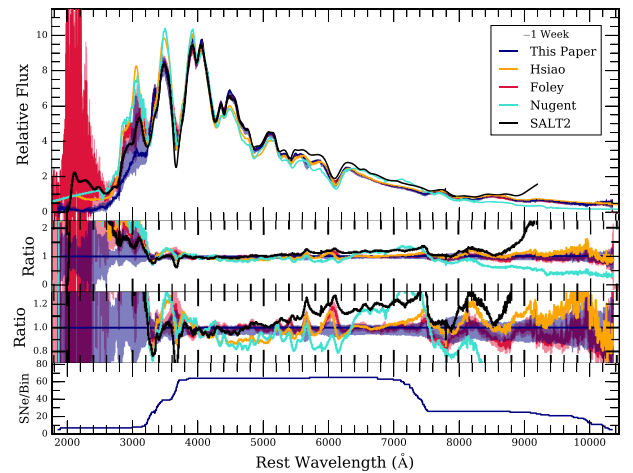
Figure 28. Same as Fig. 26 except the composite spectrum (blue curve) is constructed using a phase bin of -8 < \tau < -6 d and \Delta m_{15}(B) < 1.8 mag.
