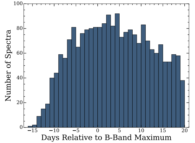
Figure 5. Histogram of the number of individual SN spectra at each epoch within 20 d of maximum brightness in the nominal sample.
