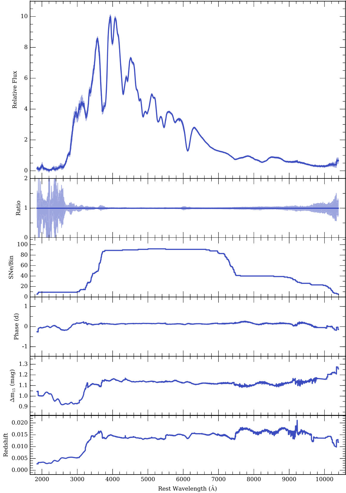
Figure 14. ( first panel ): Maximum-light composite spectrum created from our nominal sample consisting of spectra from 145 spectra of 96 SNe ( -1 < \tau < +1 d, and \Delta m_{15}(B) < 1.8 mag). The light-blue region is the 1\sigma bootstrap sampling uncertainty. ( second panel ): The light-blue region is the ratio of the 1\sigma bootstrap sampling uncertainty relative to the composite spectrum. ( third panel ): The number of individual spectra contributing to each wavelength bin. For this composite spectrum, a minimum of 5 and a maximum of 96 spectra contribute at any given wavelength. ( fourth panel ): The average phase relative to maximum brightness as a function of wavelength for this composite spectrum. ( fifth panel ): The average value of \Delta m_{15}(B) as a function of wavelength for this composite spectrum. ( sixth panel ): The average redshift of the composite spectrum as a function of wavelength.
