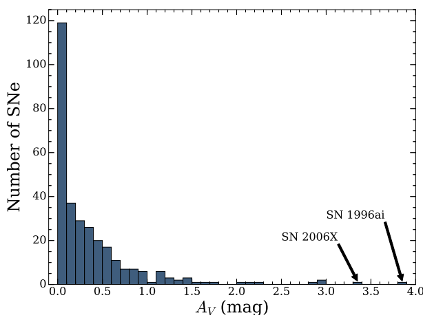
Figure 9. Histogram of the number of SNe Ia per host-galaxy extinction bin.
