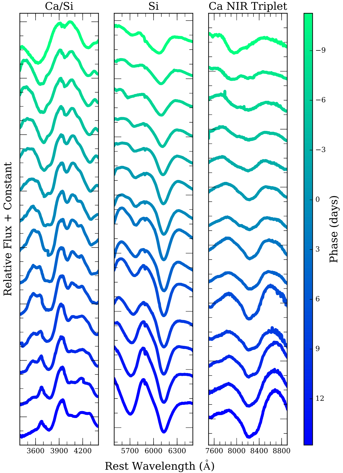
Figure 18. Zoomed-in composite spectra within 16 d of maximum light created from the nominal sample. The spectral absorption features associated with Ca II H&K, Si II, and the Ca II NIR triplet are shown in the left-hand, middle, and right-hand panels, respectively. Bin sizes of 2 d are used for each of these composite spectra.
