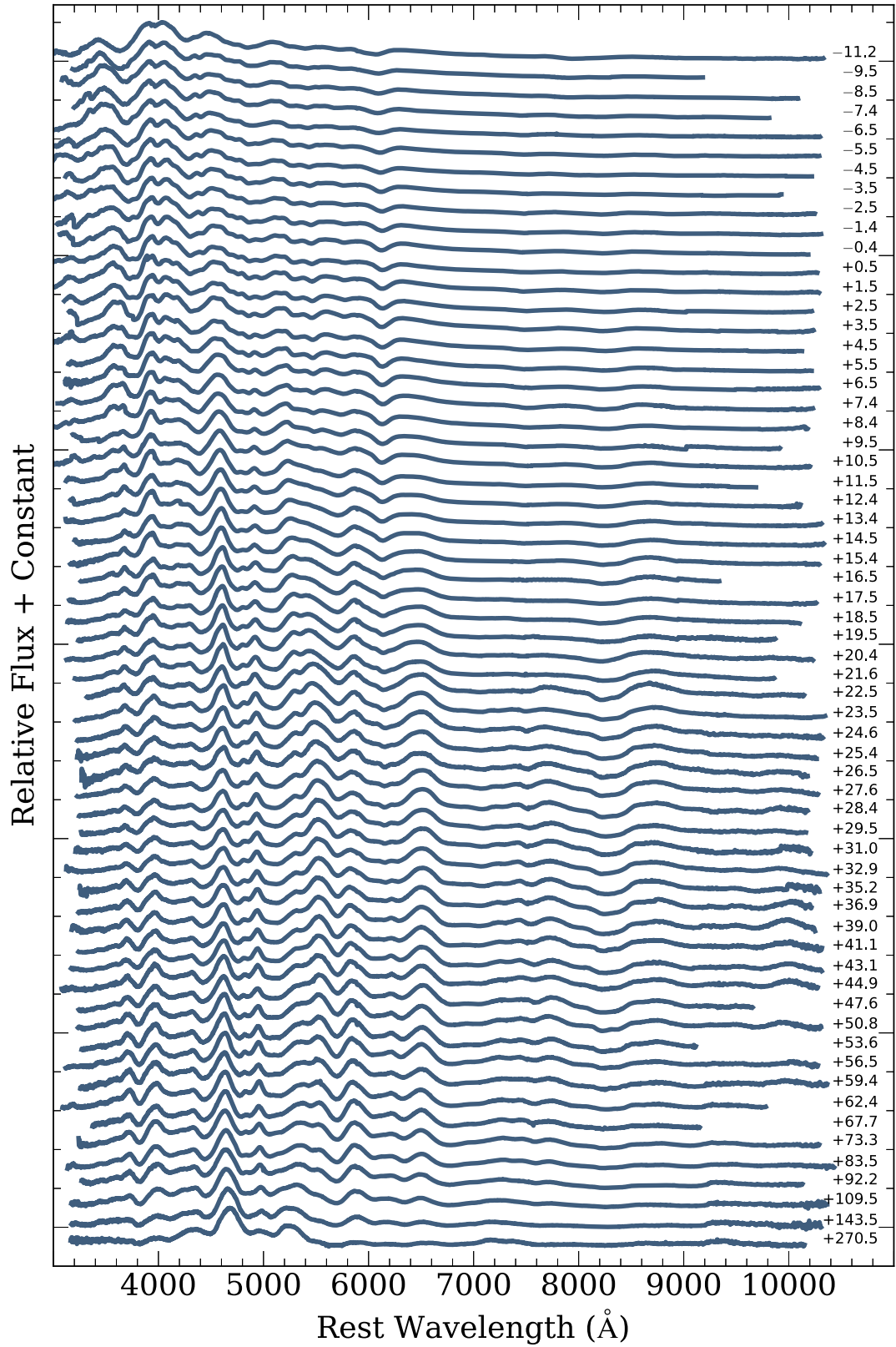
Figure 17. Composite spectra generated from the nominal sample showing the time evolution of spectral features of SNe Ia. A time series is plotted with effective phases of t = -11.3 to t = 271.2 d relative to B maximum brightness. Minimum bin sizes of 1 d are enforced near maximum brightness. Bin sizes are adjusted accordingly at later epochs to include a statistically significant ( N \geq 20 ) sample for each composite spectrum.
