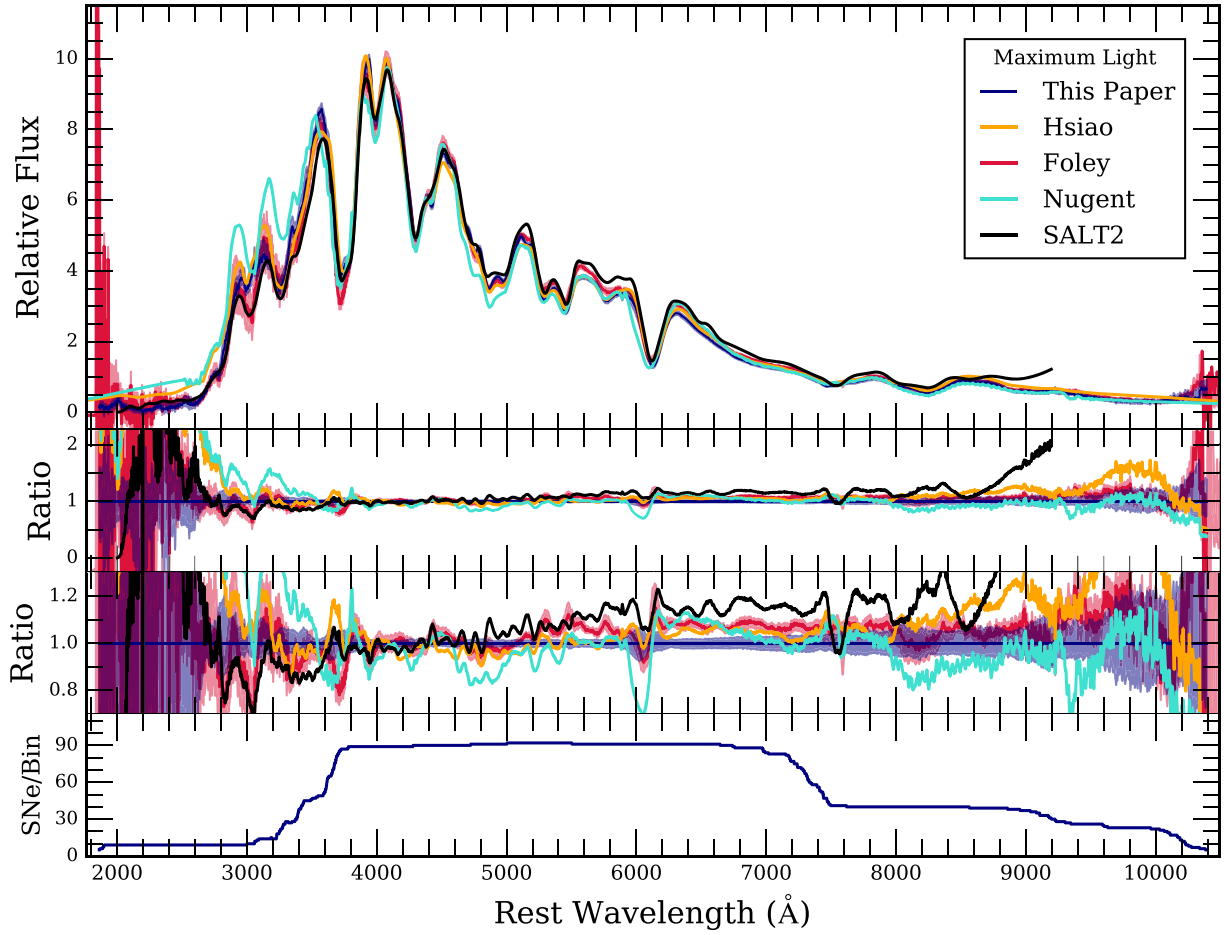
Figure 26. ( first panel ): Comparison of our maximum-light composite spectrum (blue curve) from Fig. 14 to maximum-light template spectra from Hsiao (orange curve), Foley (red curve), Nugent (light-blue curve), and SALT2 (black curve). The blue- and red-shaded regions are the 1\sigma bootstrapping uncertainty on the composite spectra from this work and Foley, respectively. ( second panel ): The ratio as a function of wavelength of a given template spectrum to our maximum-light composite spectrum. ( third panel ): Zoomed-in version of the second panel to emphasize smaller differences between template spectra. The light-blue shaded region is the 1\sigma bootstrap variation of the total maximum-light composite spectrum. ( fourth panel ): The number of individual spectra contributing to each wavelength bin of the total maximum-light composite spectrum.
