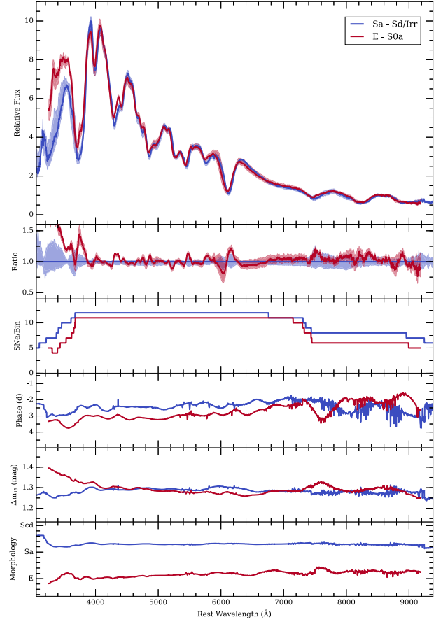
Figure 34. Same format as Fig. 14 except the bottom panel now displays the average host-galaxy morphology of a given composite spectrum as a function of wavelength. The blue curves show the properties of our late-type composite spectrum and the red curves show the properties of our early-type composite spectrum. Both of these composite spectra were constructed using a phase bin of -6 < \tau < 0 . The late-type composite spectrum was constructed using a light-curve shape bin of 1.20 < \Delta m_{15}(B) < 1.45 mag. The early-type composite spectrum was constructed using a light-curve shape bin of 1.15 < \Delta m_{15}(B) < 1.50 mag.
