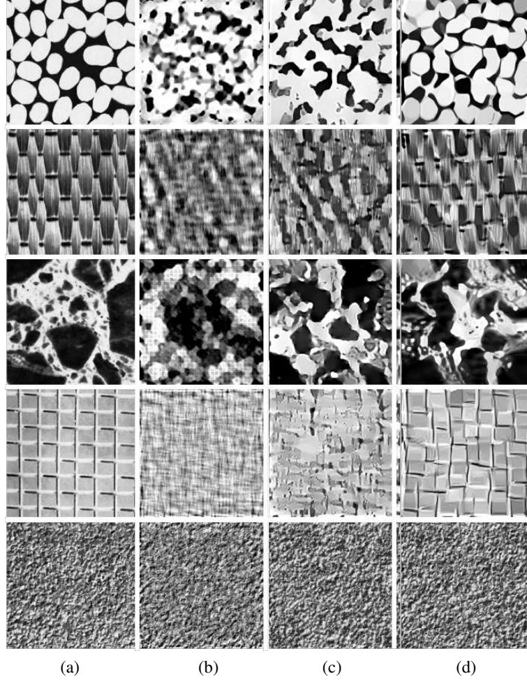
Figure 5. (a) Original texture. (b) texture synthesized with a microcanonical gradient descent model with a vector \Phi_d(x) of wavelet \mathbf{I}^2 norms. (c) \Phi_d(x) has wavelet \mathbf{I}^1 norms. (d) \Phi_d(x) has wavelet scattering coefficients.
