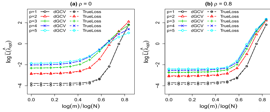
Figure 4. The logarithm of averaged true empirical losses versus \log(m)/\log(N) with a sample size N = 2^{12} and (a) \rho = 0 , (b) \rho = 0.8 .
