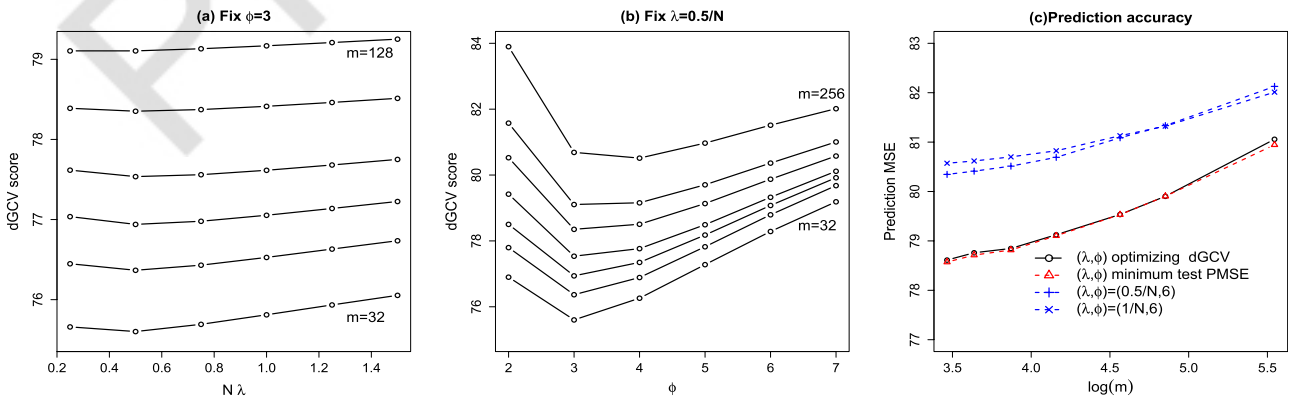
Figure 8. (a) dGCV score versus N\lambda with m = 32 (the bottommost) to m = 128 (the uppermost); (b) dGCV score versus \phi with m = 32 (the bottommost) to m = 256 (the uppermost); (c) the prediction mean squared errors on the testing samples versus \log(m) .
