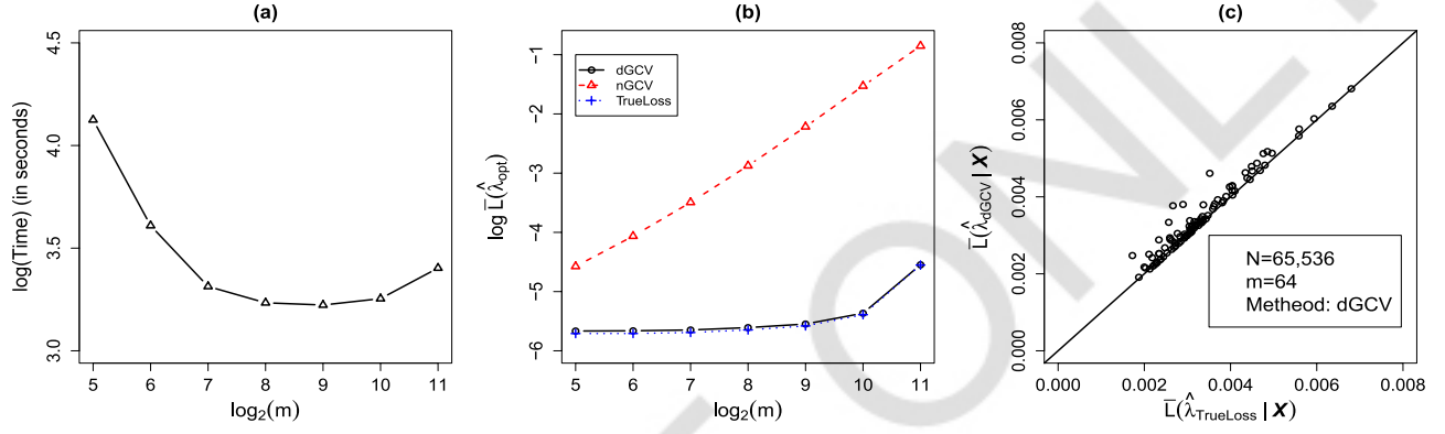
Figure 5. (a) The logarithm of computational time (in seconds) versus \log_2(m) ; (b) the logarithm of averaged true empirical losses versus \log_2(m) ; (c) scatterplots of true empirical losses of function estimators. Note that in (b), \hat{\lambda}_{\text{opt}} in the y-axis denotes one of \hat{\lambda}_{\text{dGCV}} , \hat{\lambda}_{\text{nGCV}} and \hat{\lambda}_{\text{TrueLoss}} for each curve.
