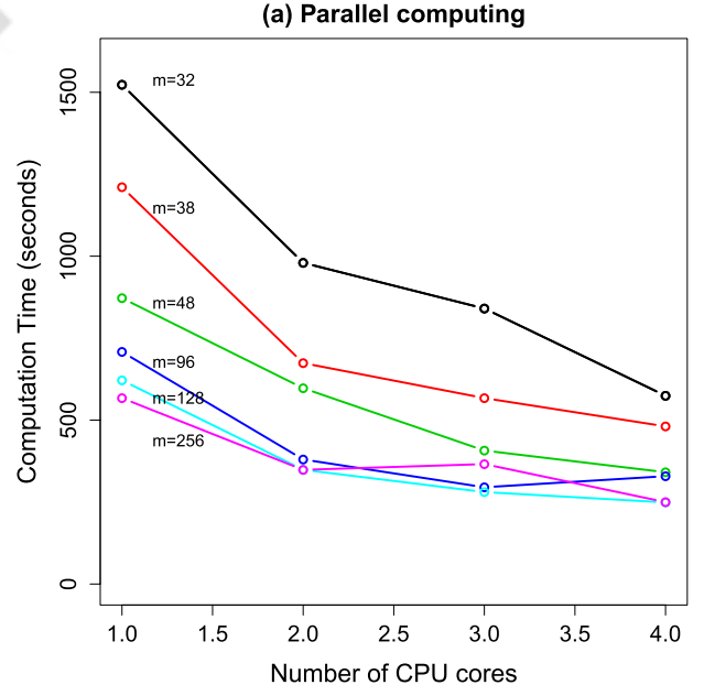
Figure 7. Computing times versus number of CPU cores.
