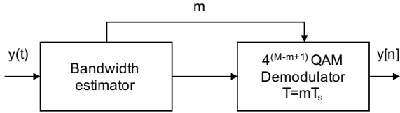
Fig. 4: Block diagram for the HBM demodulator.
