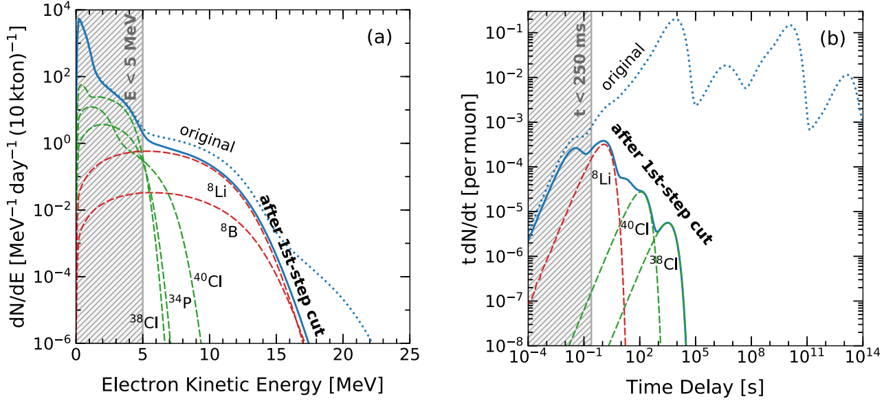
FIG. 3. Spallation spectra in DUNE after the first-step cut (discard events with t < 250 ms), assuming a 5-MeV energy threshold. Events in the gray shaded regions are discarded, which introduces 1% downtime. Left panel (a) : Energy spectra of spallation \beta s (with nominal 7% energy resolution). Blue dotted line: pre-cut spallation spectrum. Blue solid line: postcut spallation spectrum. Green dashed lines: \beta s from selected high- A isotopes. Red dashed lines: \beta s from selected low- A isotopes. Right panel (b) : Time profile of spallation \beta s, normalized per vertical muon, with the same labeling conventions.
