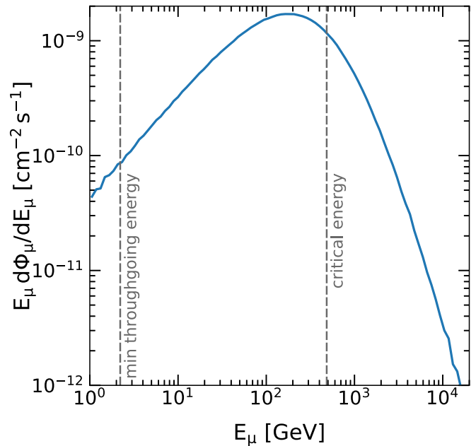
FIG. 1. Simulated cosmic-ray muon flux at DUNE (4850 ft underground) as a function of muon total energy [44–46]. The dashed line near 2 GeV corresponds to the minimum-ionization energy loss for a vertical muon passing through DUNE’s fiducial volume. The dashed line at 484 GeV shows the muon critical energy in liquid argon.
