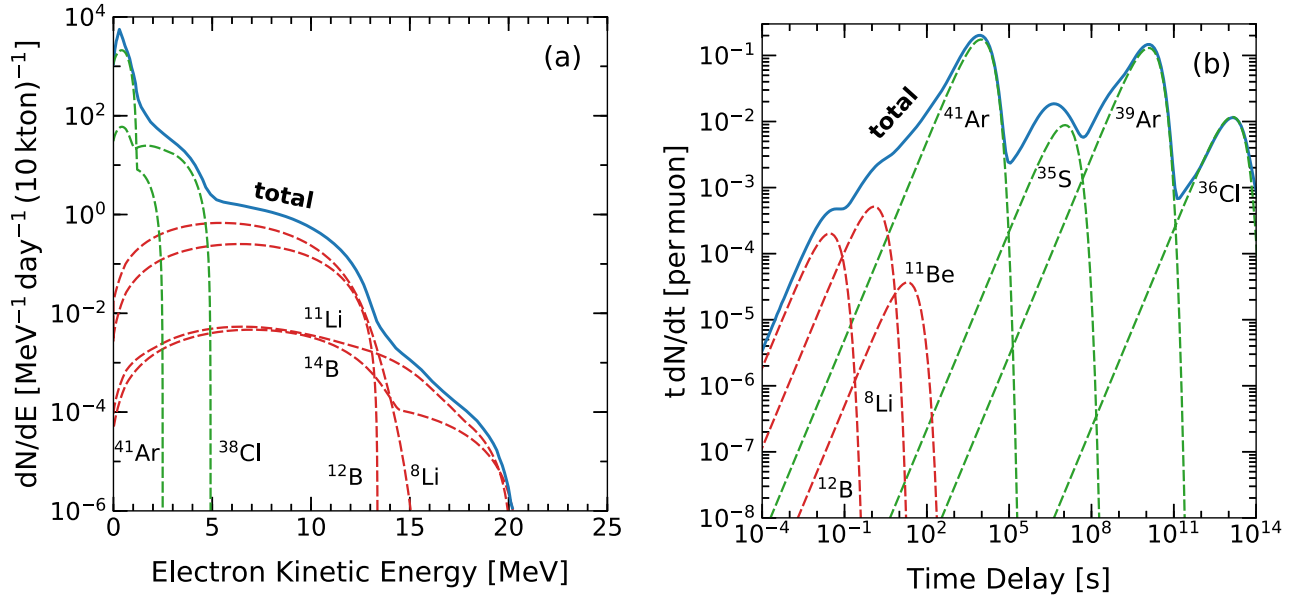
FIG. 2. Spallation spectra in DUNE before cuts (assuming equilibrium between isotope production and decay). Left panel (a) : Energy spectra of spallation \beta s (no energy smearing yet). Blue solid line: total spallation rate. Green dashed lines: \beta s from selected high- A isotopes. Red dashed lines: \beta s from selected low- A isotopes. Right panel (b) : Time profile of spallation \beta s, normalized per vertical muon, with the same labeling conventions.
