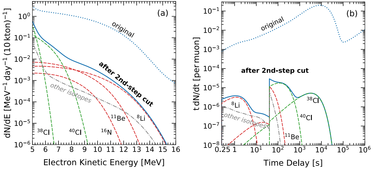
FIG. 5. Spallation spectra in DUNE after both the first-step and second-step cuts. The total dead time is 5%. Note the change of energy and time ranges compared to Fig. 3. Left panel (a) : Energy spectra of spallation \beta s (including 7% energy resolution). Blue dotted line: precut spallation spectrum. Blue solid line: postcut spallation spectrum. Green dashed lines: \beta s from selected high- A isotopes. Red dashed lines: \beta s from selected low- A isotopes. Gray dash-dotted line: remaining postcut backgrounds from the isotopes not listed individually. Right panel (b) : Time profile of spallation \beta s, normalized per vertical muon, with the same labeling style. The sharp feature at 40 s is due to the time duration of the cylinder cut.
