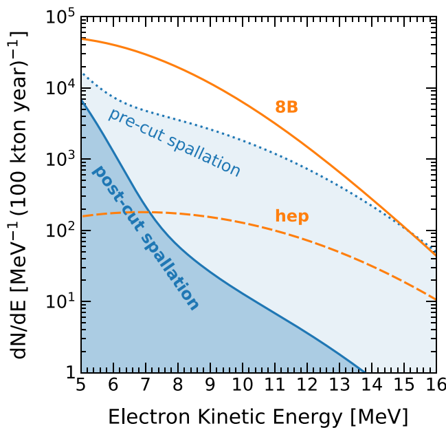
FIG. 10. Same as Fig. 7, but with 20% energy resolution.
