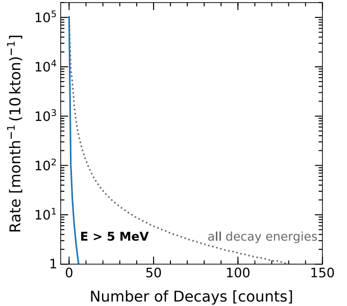
FIG. 13. Spallation isotope decay multiplicities per muon in DUNE. Bin size is 1 count. Gray dotted line: all spallation betas. Blue solid line: spallation decays above the 5-MeV threshold (in electron energy).
