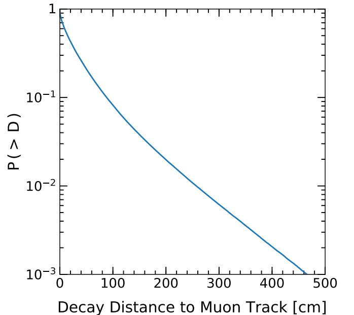
FIG. 4. Reverse cumulative distribution of spallation \beta s that survive from the first-step cut in perpendicular distance to the muon track.
