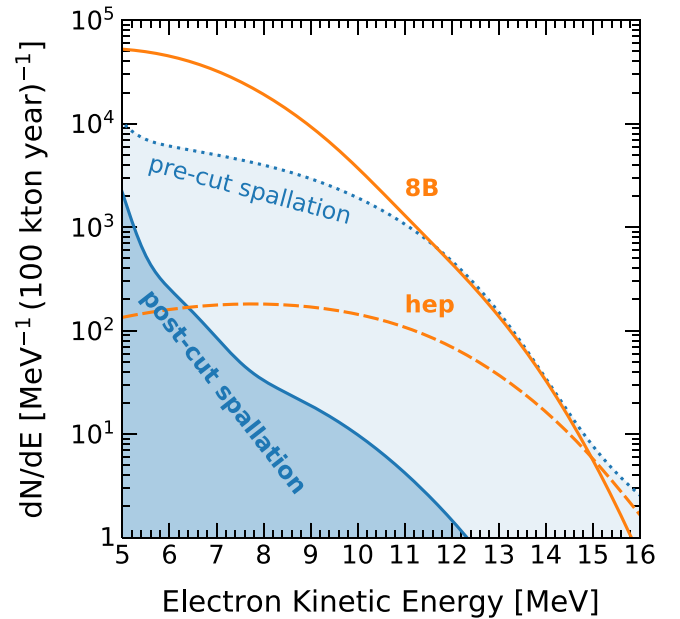
FIG. 7. Solar neutrino signal rates [1] and spallation background rates in DUNE, with nominal 7% energy resolution. (Other backgrounds, due especially to neutron capture, which dominates at low energy, are not shown.) The dead time imposed by the spallation cut is not accounted for the signal rates. Orange solid line: total ^8\text{B} signal rates from charged-current channel and elastic-scattering channel. Orange dashed line: total ^7\text{He} signal rates from the two channels. Light blue shaded: precut spallation spectrum. Dark blue shaded: postcut spallation spectrum (same as Fig. 5).
