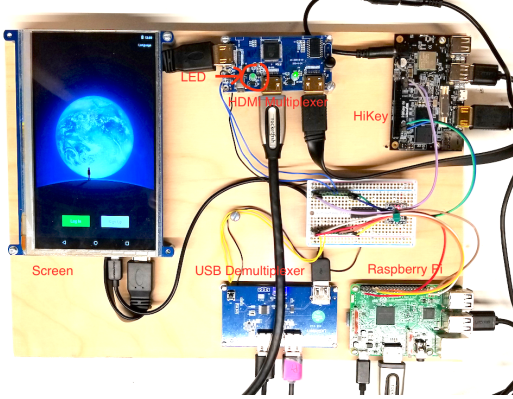
Figure 10: Hardware Implementation
