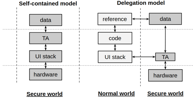
Figure 1: TrustZone UI Design Models
