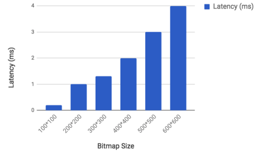
Figure 13: Image Rendering Overhead
