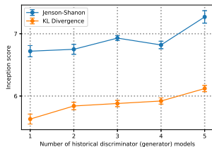
Fig. 6: We show that Fictitious-GAN can improve Inception score as a meta-algorithm with larger number of historical models, We select 2 divergence metrics from Table 1: Jenson-Shanon and KL divergence.
