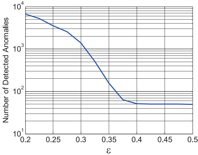
Fig. 6. Variation in the number of detected anomalies as function of \varepsilon .
