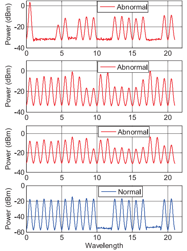
Fig. 5. Examples of normal and abnormal data instances.
