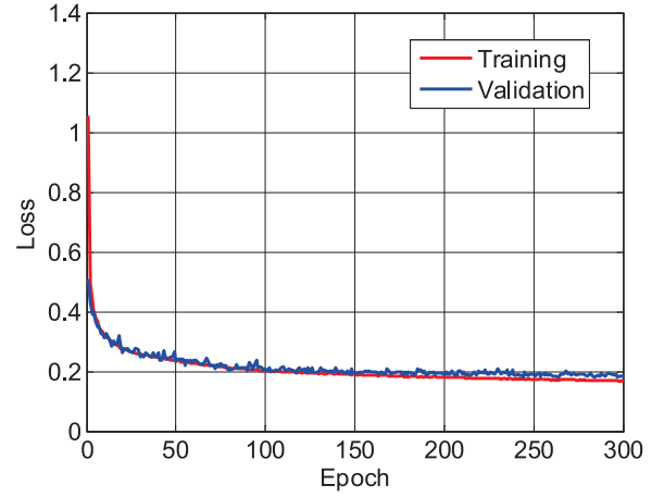
Fig. 7. Losses of the DRCM during training.
