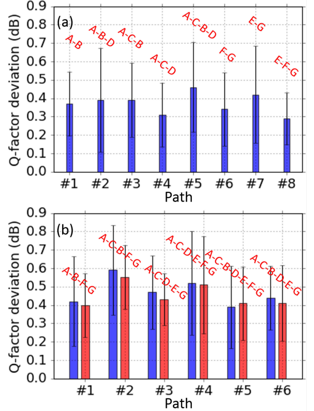
Fig. 6. Q-factor deviations of the evaluation sets for (a) domain manager-level ANN bank and (b) broker-level ANN bank. The blue and red bars correspond to hierarchical and omniscient QoT estimators.
