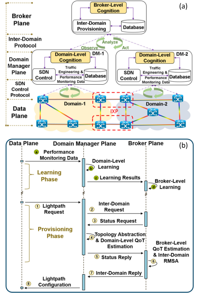
Fig. 1. (a) Broker-based multi-domain provisioning with Hierarchical Cognition. IXP: internet-exchange point; DM: domain managers; (b) Workflow of the proposed system.
