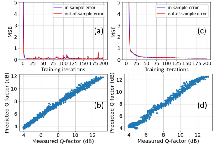
Fig. 5. Inter-domain learning performance for path A-C-D-E-F-G. (a) MSE vs. training iterations for omniscient estimator; (b) QoT prediction accuracy for omniscient estimator; (c) MSE vs. training iterations for hierarchical estimator; (d) QoT prediction accuracy for hierarchical estimator.
