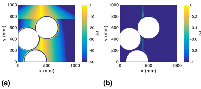
Figure 8. Cost reduction \Delta J , modeled after (9), for sampled x and y in the presence of obstacles, given second-order needle variation controls. The first- and second-order mode insertion gradients are evaluated with the controls from (11). Figures 8a and 8b are identical, but shown over a different range to illustrate that even when looking at small variations of the first-order mode insertion gradient, the second-order method is reliably negative. The bright vertical line in Fig. 8b is vertically aligned with the target located at [400 mm, 1000 mm], where first-order solutions are singular. No data are sampled inside the white circles, as these indicate the infeasible occupied region.
