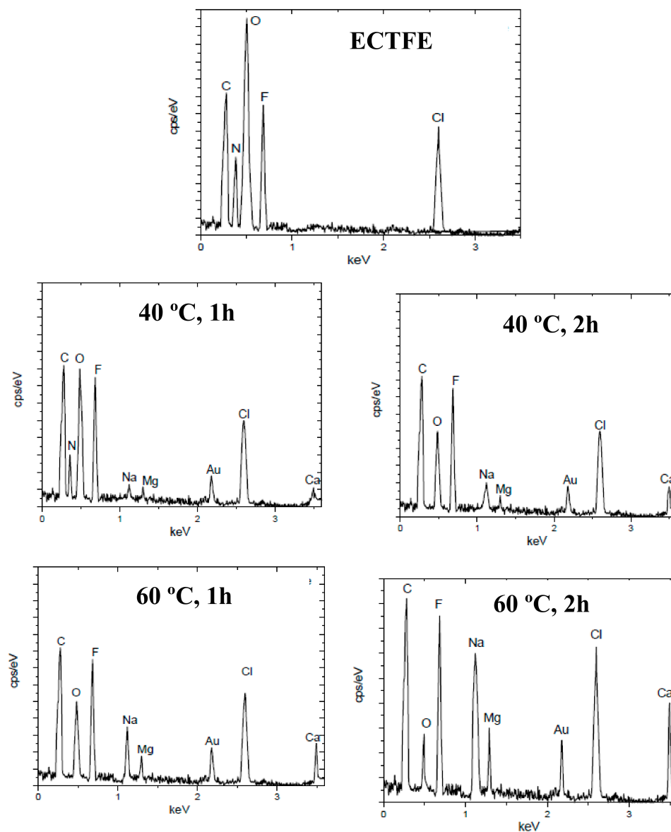
Figure 8. The EDX spectra for fouled membranes: base and modified.
