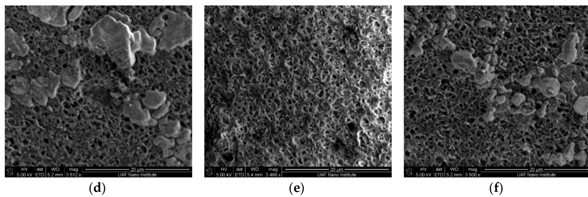
Figure 7. The SEM images for the fouled membranes (a) Base ECTFE; (b) base membrane after MD; (c) 1 h 40 °C modified membrane after MD; (d) 2 h 40 °C modified membrane after MD; (e) 1 h 60 °C modified membrane after MD; (f) 2 h 60 °C modified membrane after MD.
