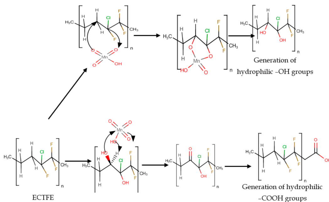
Scheme 1. The schematic of the formation of hydrophilic functional groups ( -\text{OH} and -\text{COOH} ) on surface oxidation of ECTFE membrane by \text{KMnO}_4 .
