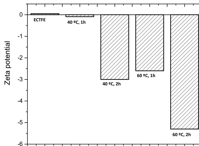
Figure 4. The zeta potential for the modified membranes.
