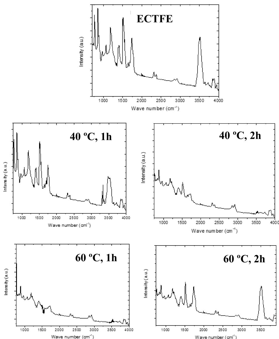
Figure 9. FTIR spectra for fouled membranes: base and modified.
