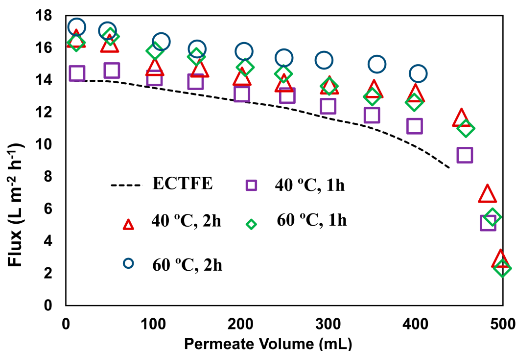
Figure 5. The performance of modified membranes during membrane distillation using real PW as feed.
