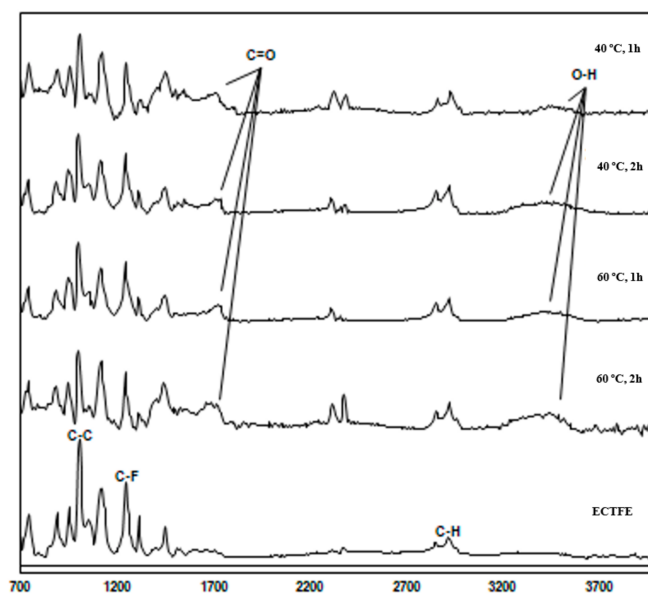
Figure 2. FTIR spectra for virgin and modified ECTFE membranes.
