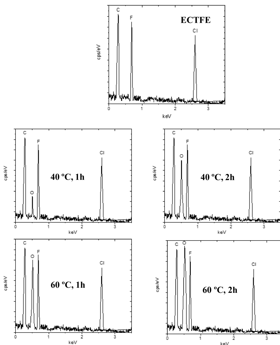
Figure 3. The EDX spectra for modified membranes.
