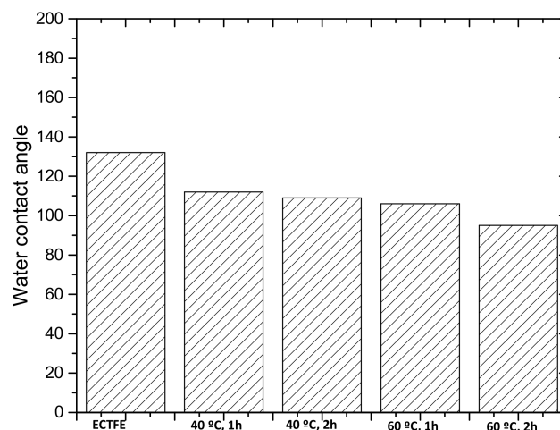
Figure 1. Water contact angles for modified ECTFE membranes.
