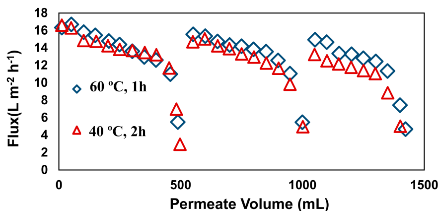
Figure 6. The performance of modified membranes after three consecutive MD cycles with onsite cleaning.
