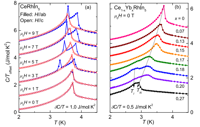
FIG. 11. (a) Specific heat divided by temperature C/T for CeRhIn_5 in applied magnetic fields \mu_0 H of up to 9 T; H was applied parallel to both the ab plane (filled circles) and along the c axis (open circles). Note that data measured in different magnetic fields have been offset from one another by an amount \delta C/T = 1.0 J/mol K 2 for visual clarity. When H \parallel c , we observe a single feature at T_N which is gradually suppressed to lower temperature with increasing H . When H \parallel ab and \mu_0 H > 3 T, we observe a feature at T_N and a magnetic-field-induced phase transition at T_I ( T_I < T_N ). (b) C/T data for Ce_{1-x}Yb_xRhIn_5 are plotted in the vicinity of T_N . The data for different concentrations have been offset from one another by an amount \delta C/T = 0.5 J/mol K 2 for visual clarity. A second feature emerges at temperatures T_I < T_N for x_{act} > 0.18 . Dashed lines are guides to the eye which emphasize the evolution of T_N and T_I with Yb concentration.
