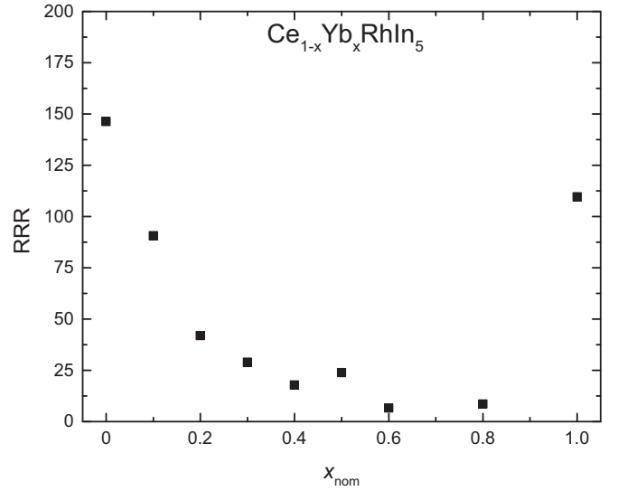
FIG. 7. Calculated RRR values from \rho(T) plotted vs x_{\text{nom}} for \text{Ce}_{1-x}\text{Yb}_x\text{RhIn}_5 . At x_{\text{nom}} = 0 , the \text{RRR} \approx 150 . As Yb is introduced, the RRR drops precipitously. For the pure \text{YbRhIn}_5 compound, the RRR increases to above 110, suggesting that substituted samples are likely to yield low RRR values, potentially related to the issues raised regarding synthesis in the range x_{\text{nom}} > 0.8 discussed in the text.
