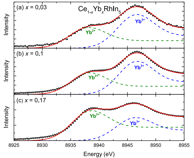
FIG. 4. Measured Yb L_{III} edge data for Ce_{1-x}Yb_xRhIn_5 are plotted as black circles. The fit to the two-edge model is shown as the red solid line, while the dashed green line represents the contribution from Yb^{2+} , and the dashed blue line represents the contribution from Yb^{3+} . The results are shown over the same energy ranges for x = 0.03 , 0.1, and 0.17 in panels (a), (b), and (c), respectively.
