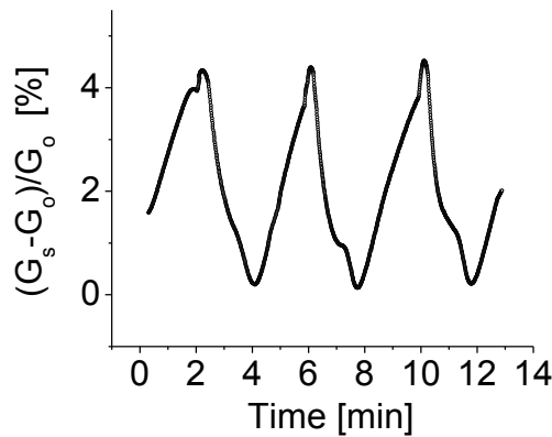
Figure 8 The responses of the prototype at operating temperature of 80^\circ C , bias voltage of 1.0 V to H_2 gas with concentration of 2k ppm.
