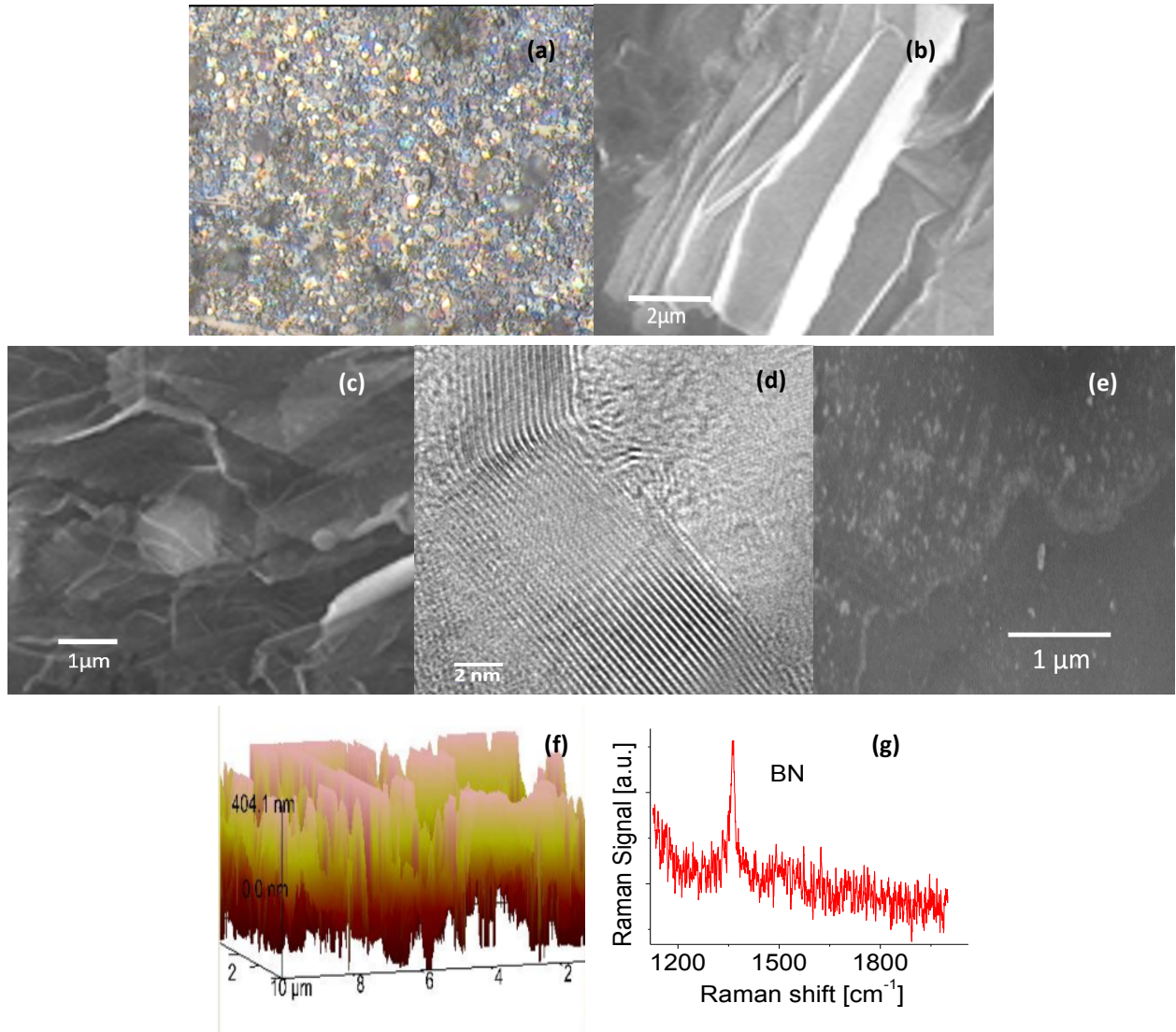
Figure 1(a) optical microscope, (b, c) SEM, (d) HRTEM, (f) AFM images, and (g) Raman spectrum of the as-prepared BNNS film, and (e) SEM image of functionalized BNNS film.
