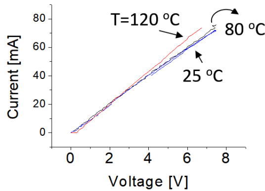
Figure 4 Electrical current-voltage (IV) properties of the functionalized BNNS sample at different temperatures.
