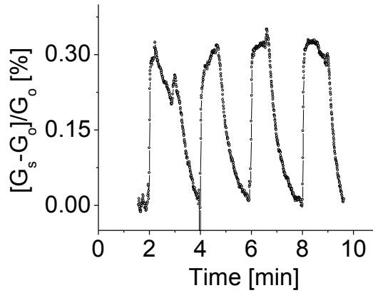
Figure 7 The responses of the prototype at room temperature, 1.0 V bias voltage to H_2 gas with concentration of 2k ppm.
