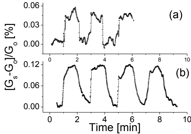
Figure 6 The responses of the prototype at room temperature, 0.5V bias voltage to CH 4 gas with concentrations of (a) 200 ppm and (b) 2k ppm.
