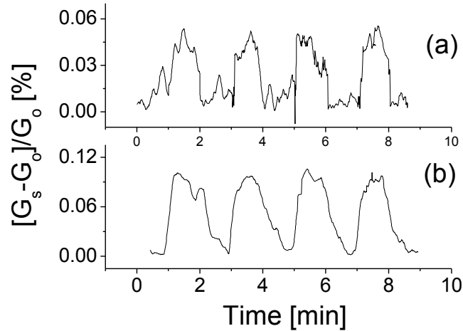
Figure 5 The responses of the prototype at room temperature, 0.5 V bias voltage to H 2 gas with the concentrations of (a) 200 ppm and (b) 2k ppm, respectively.
