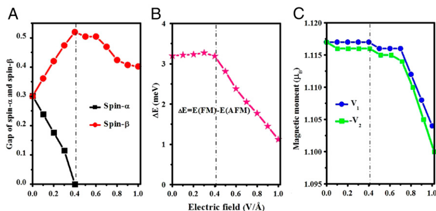
Fig. 4. (A–C) Electric field dependence of (A) the band gap of spin- \alpha and spin- \beta states, (B) energy difference between ferromagnetic and antiferromagnetic interlayer coupling, and (C) the magnetic moments of V_1 and V_2 . The critical field ( 0.4 \text{ V/Å} ) is indicated by a dashed-dotted line.
