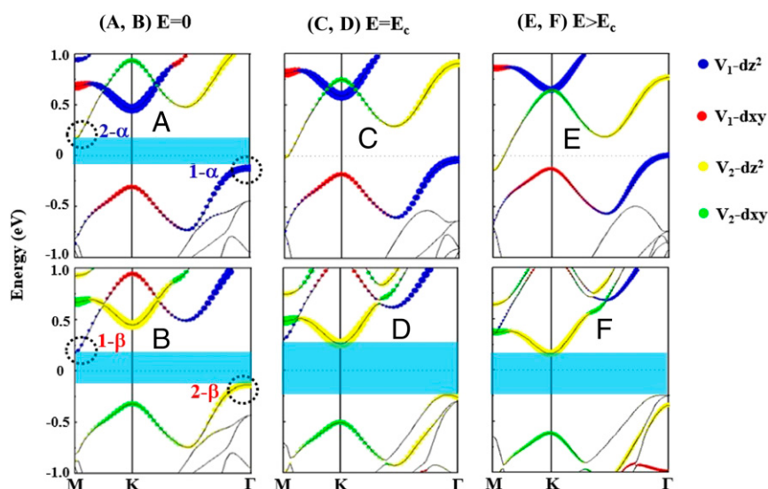
Fig. 3. (A–F) Orbital- and spin-resolved band structures of bilayer 2H-VSe 2 with (A and B) E = 0 , (C and D) E = E_c = 0.4 \text{ V/Å} , (E and F) E = 0.8 \text{ V/Å} , (A, C, and E) spin- \alpha , and (B, D, and F) spin- \beta . With a positive electric field applied, all layer-2-related bands (in yellow and green) are pushed down while layer-1 bands (in blue and red) are lifted up. After reaching the critical field, the band edges in spin- \alpha states touch at M- \Gamma (C), whereas the band edges in spin- \beta states separate farther apart and evolve from M- \Gamma (B) to K- \Gamma (F).
