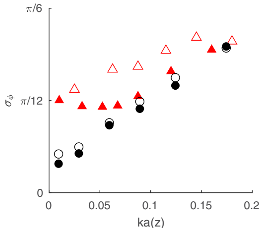
FIG. 10. Standard deviation of the wave-period-averaged polar angle \phi as a function of nondimensional wave shear ka(z) for different particle shapes: long rods (closed triangles), short rods (open triangles), large disks (closed circles), and small disks (open circles). The data come from \beta = 1.005 for all shapes except long rods which have \beta = 1.01 , and data are included only for particles that had evolved in the waves for at least 10 wave periods.
