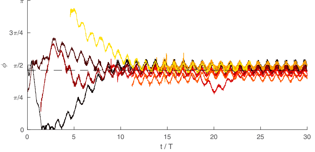
FIG. 5. Time series of the polar angle \phi for several neutrally buoyant ( \beta = 1 ) long rods in WC2 waves. Though their initial \phi values were uncontrolled, the particles all settle onto an oscillatory limit cycle at the wave frequency about a similar angle. The wave-preferred angle \phi_w^* expected from theory is marked with a dashed line.
