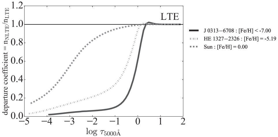
Figure 1. Comparison of departure coefficients of the FeI ground level as a function of the optical depths \log \tau_{5000} for the Sun and two UMP stars SMSS J0313–6708 and HE 1327–2326. Departures from LTE are more severe in the UMP stars than in the Sun.
