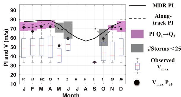
FIG. 9. As in Fig. 6, but for the Southern Hemisphere region.
