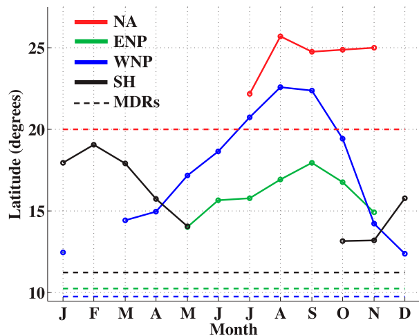
FIG. 3. Seasonal cycles (solid lines) in the average latitudes of each basin's observed maximum intensity ( V_{\max} , as defined in section 2b); shown for every month with at least five observed storms over 1980–2015. Regions are the North Atlantic (red), eastern North Pacific (green), western North Pacific (blue), and Southern Hemisphere (black). The average latitude of each main development region (which does not vary over the seasonal cycle) is shown for comparison (dashed lines).
