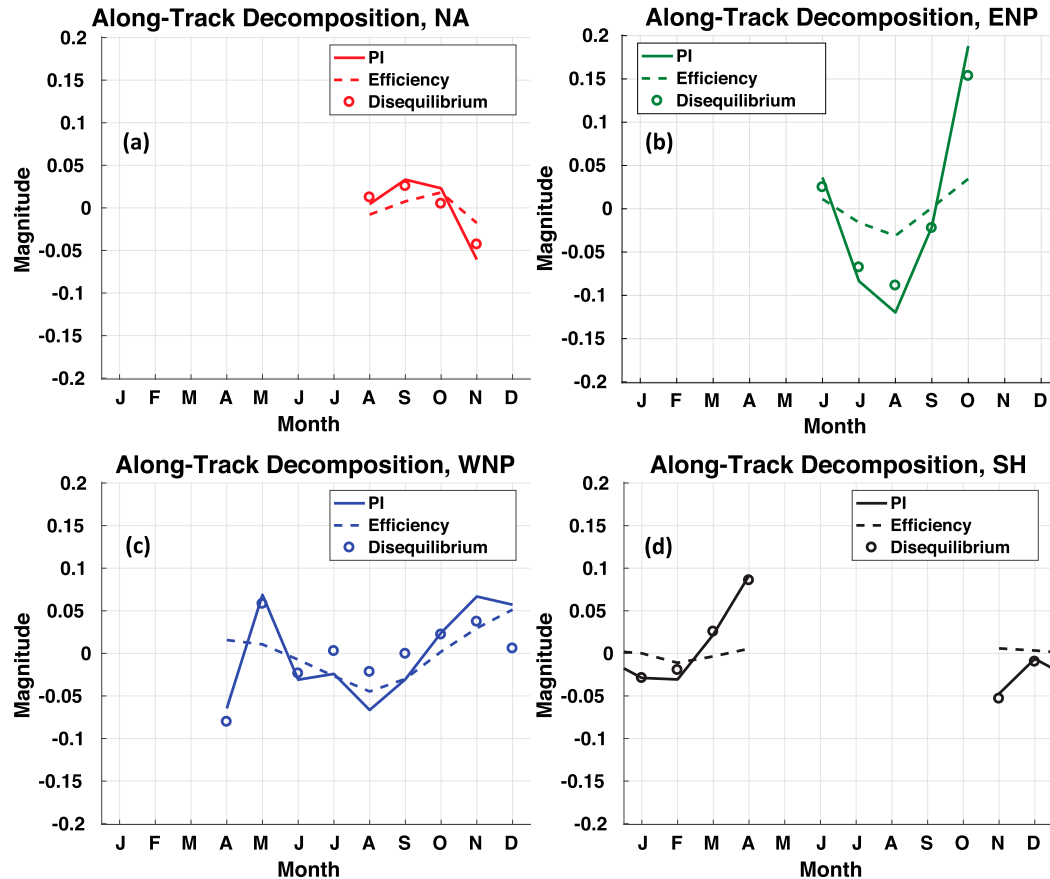
FIG. 5. Along-track seasonal anomalies of 2 times the logarithm of TC PI [solid curves; left-hand-side of Eq. (1)], the logarithm of thermodynamic efficiency [dashed curves; first term on right-hand-side of Eq. (1)], and the logarithm of thermodynamic disequilibrium [circles; second term on right-hand-side of Eq. (1)], for the (a) North Atlantic, (b) eastern North Pacific, (c) western North Pacific, and (d) Southern Hemisphere regions.
